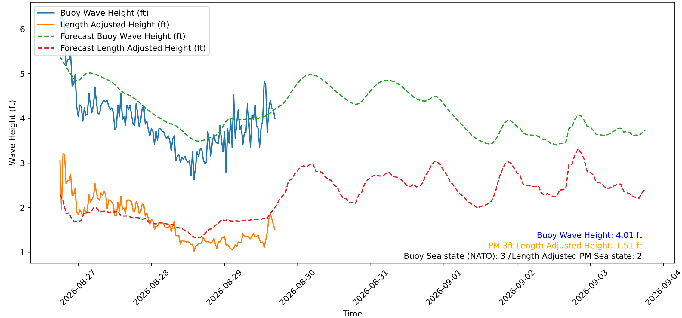
Wave Heights over Time for Green Beach at 2026-08-29 17:31:12
