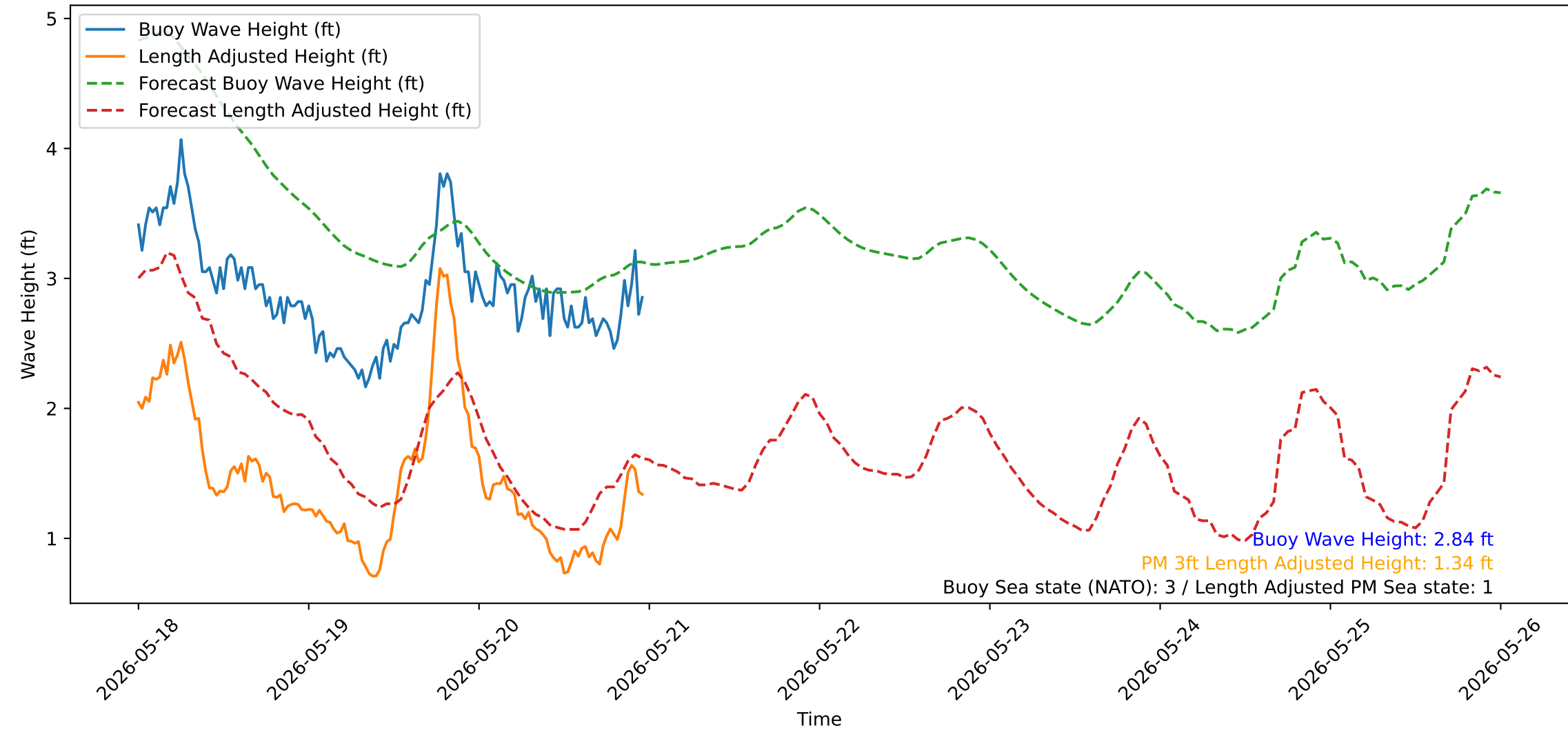
Wave Heights over Time for Green Beach at 2026-05-20 23:51:14
