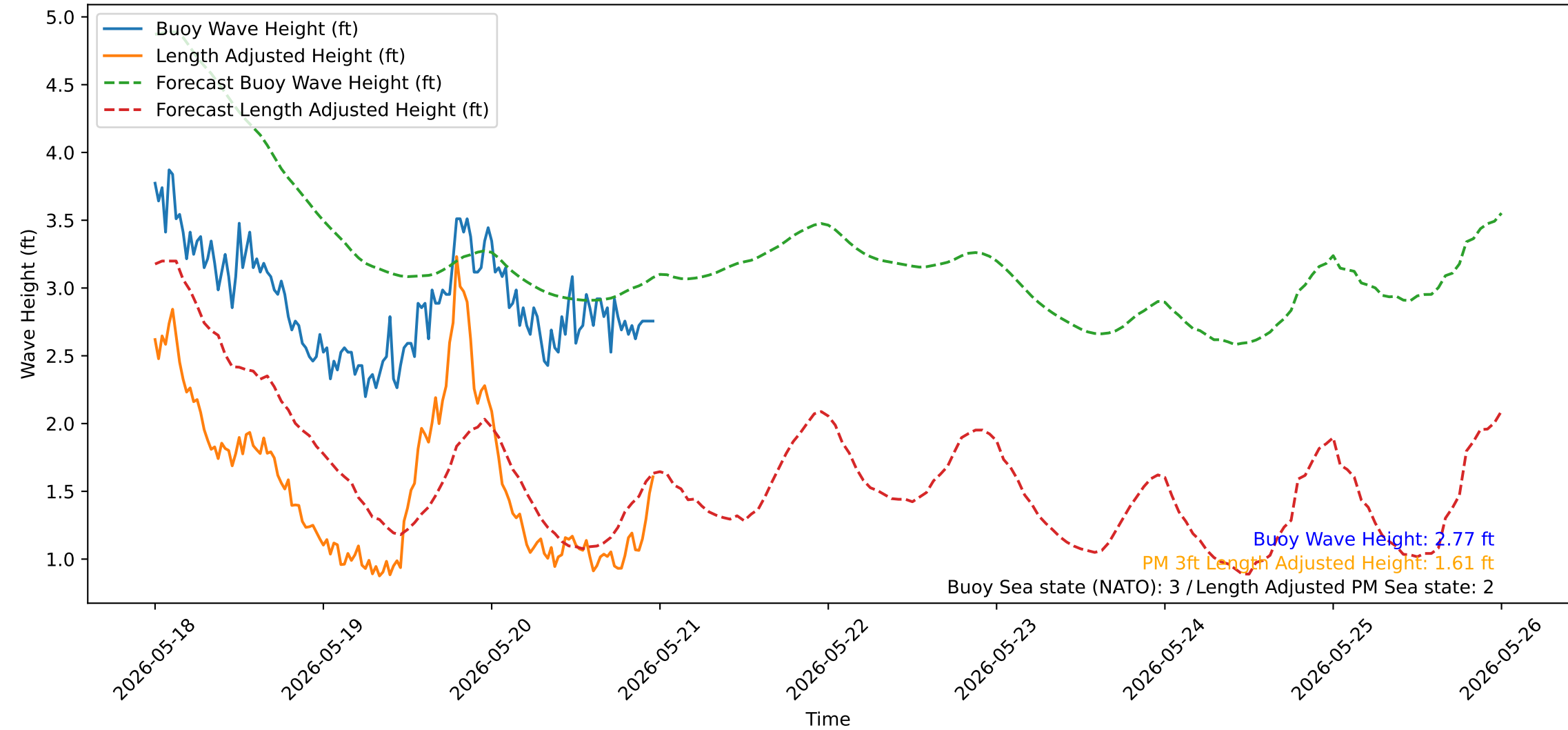
Wave Heights over Time for Oceanside Harbor at 2026-05-20 23:50:32
