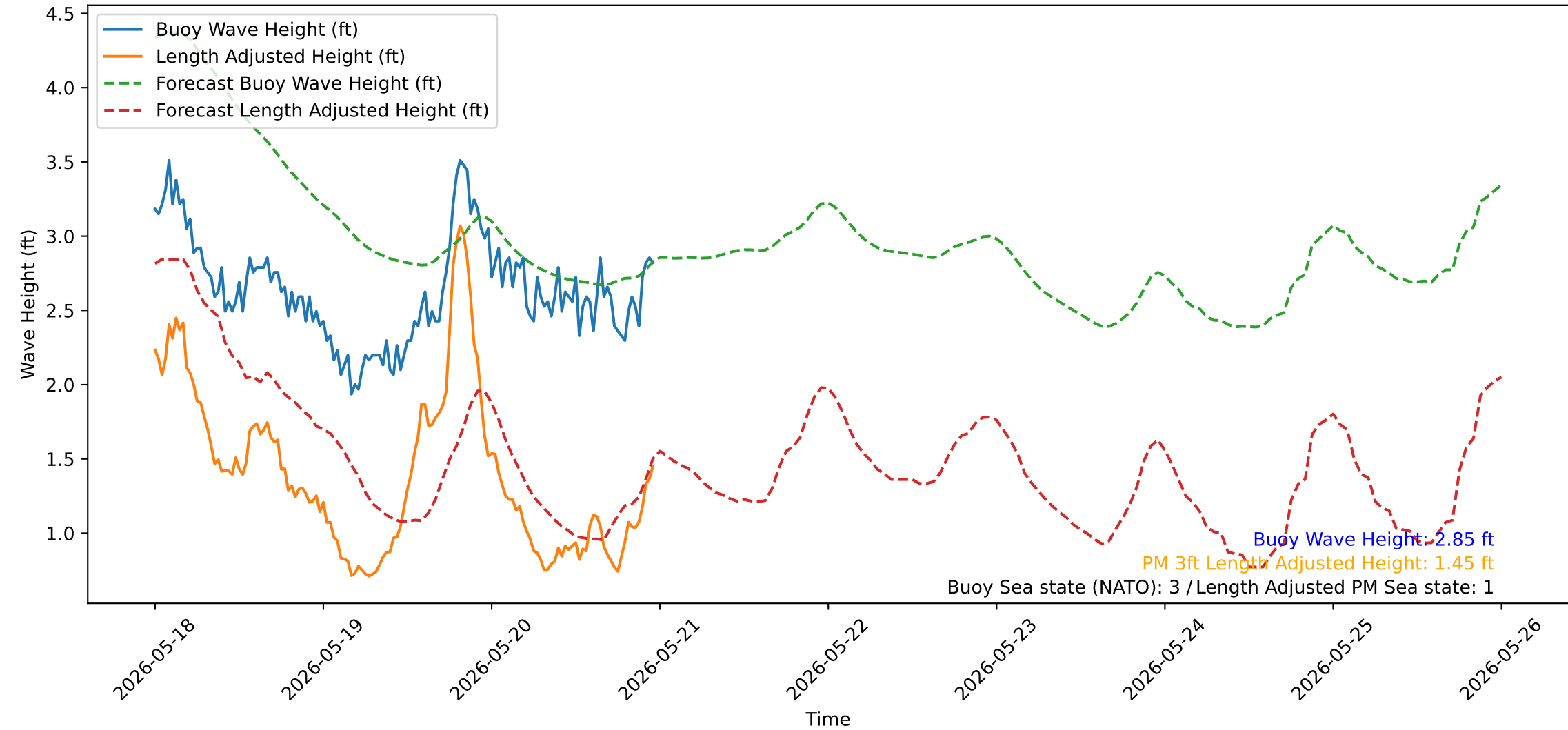
Wave Heights over Time for Red Beach at 2026-05-20 23:50:52
