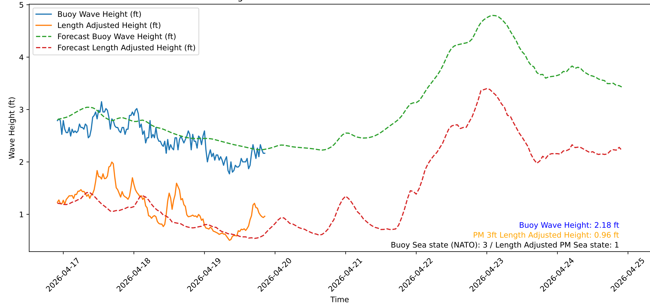
Wave Heights over Time for Red Beach at 2026-04-19 21:30:51
