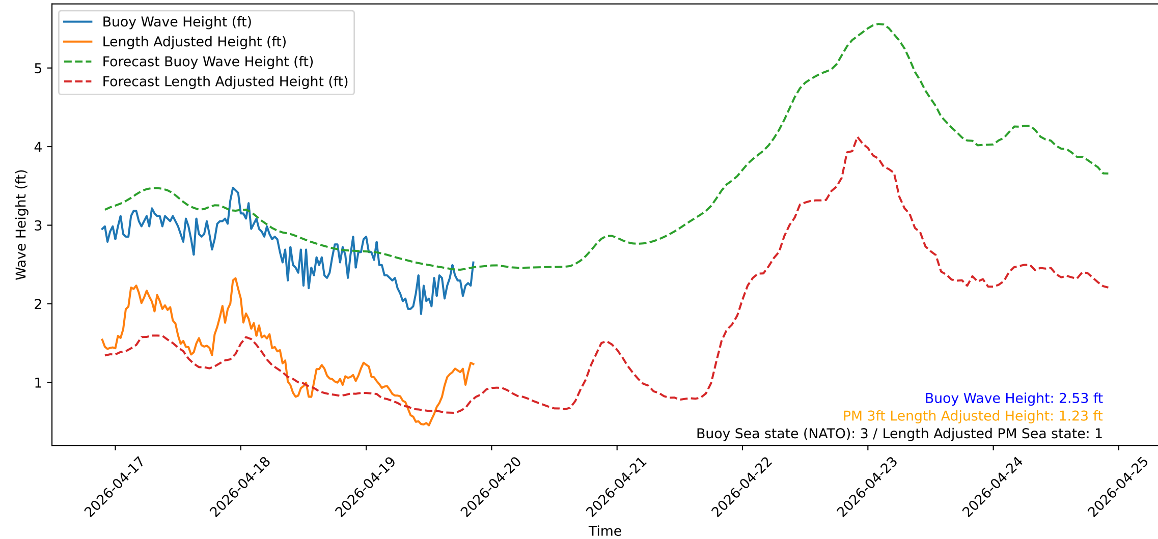
Wave Heights over Time for Green Beach at 2026-04-19 21:31:13
