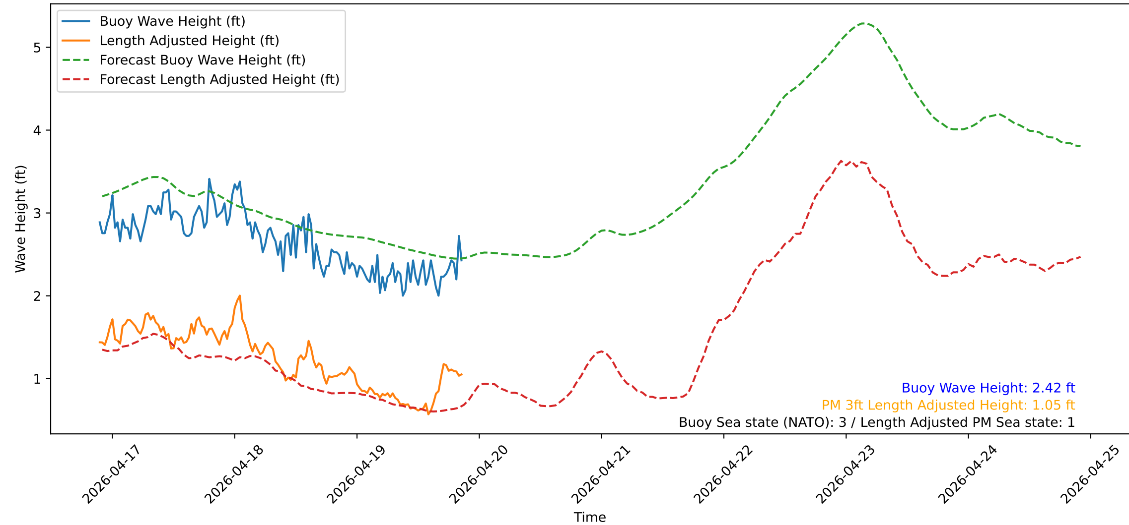
Wave Heights over Time for Oceanside Harbor at 2026-04-19 21:30:32
