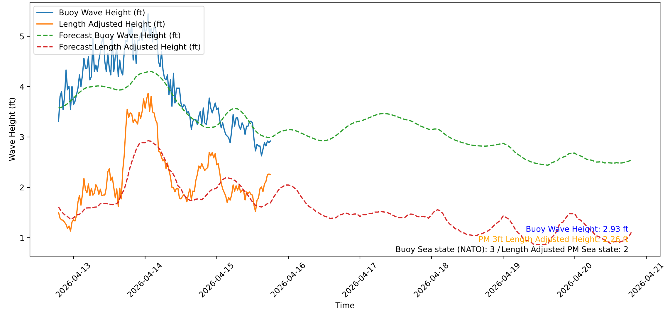
Wave Heights over Time for Oceanside Harbor at 2026-04-15 18:50:31
