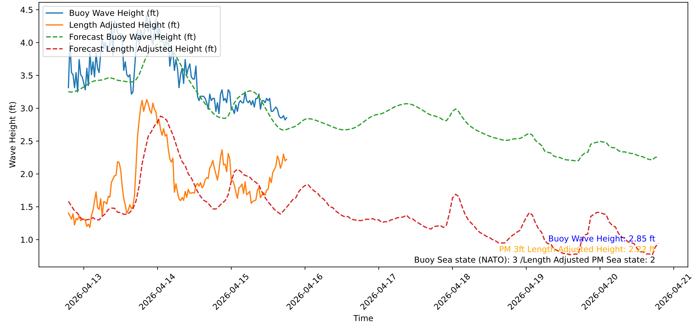
Wave Heights over Time for Red Beach at 2026-04-15 18:50:51
