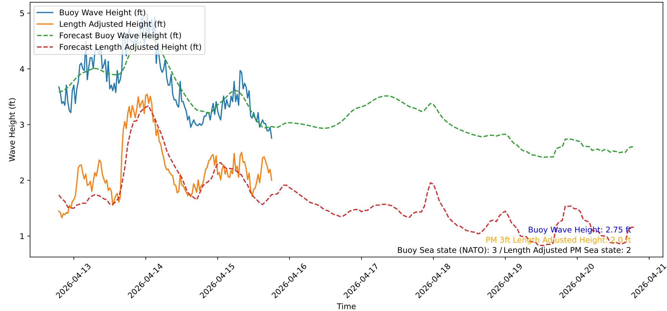
Wave Heights over Time for Green Beach at 2026-04-15 18:51:13
