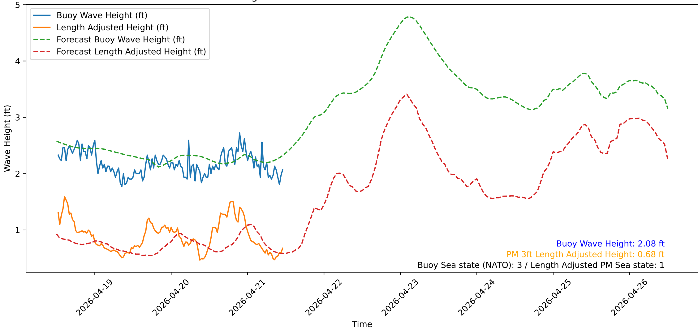
Wave Heights over Time for Red Beach at 2026-04-21 12:20:52
