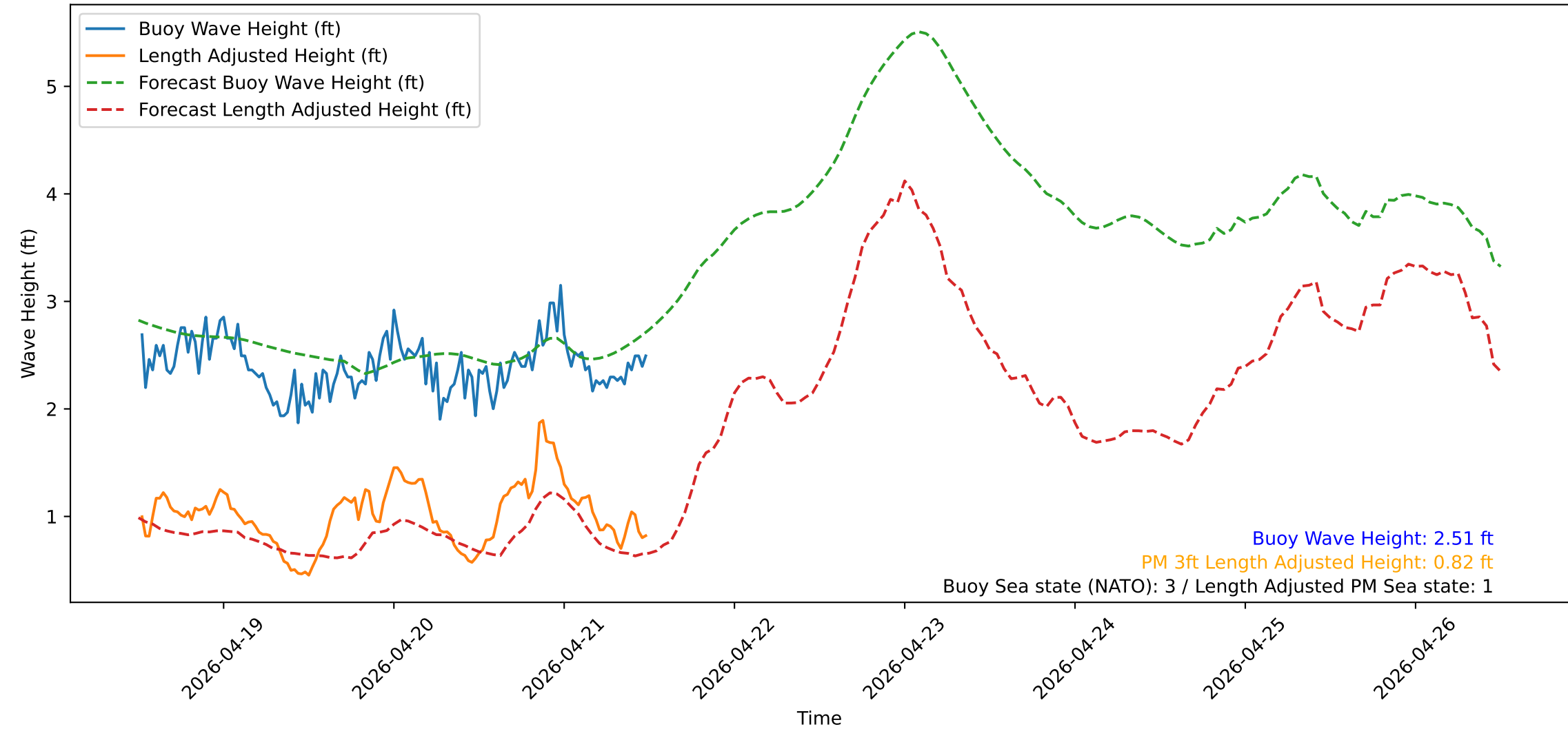
Wave Heights over Time for Green Beach at 2026-04-21 12:21:15
