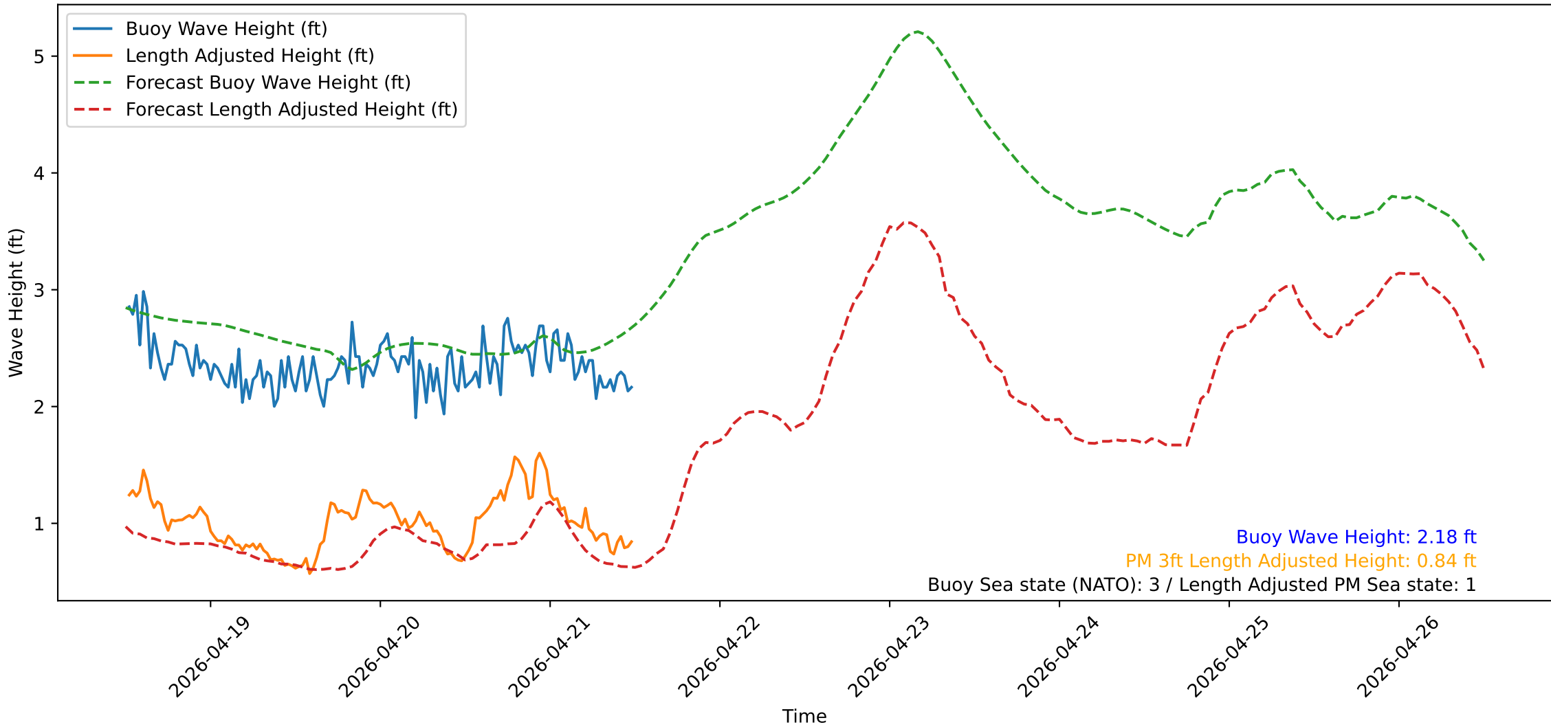
Wave Heights over Time for Oceanside Harbor at 2026-04-21 12:20:32
