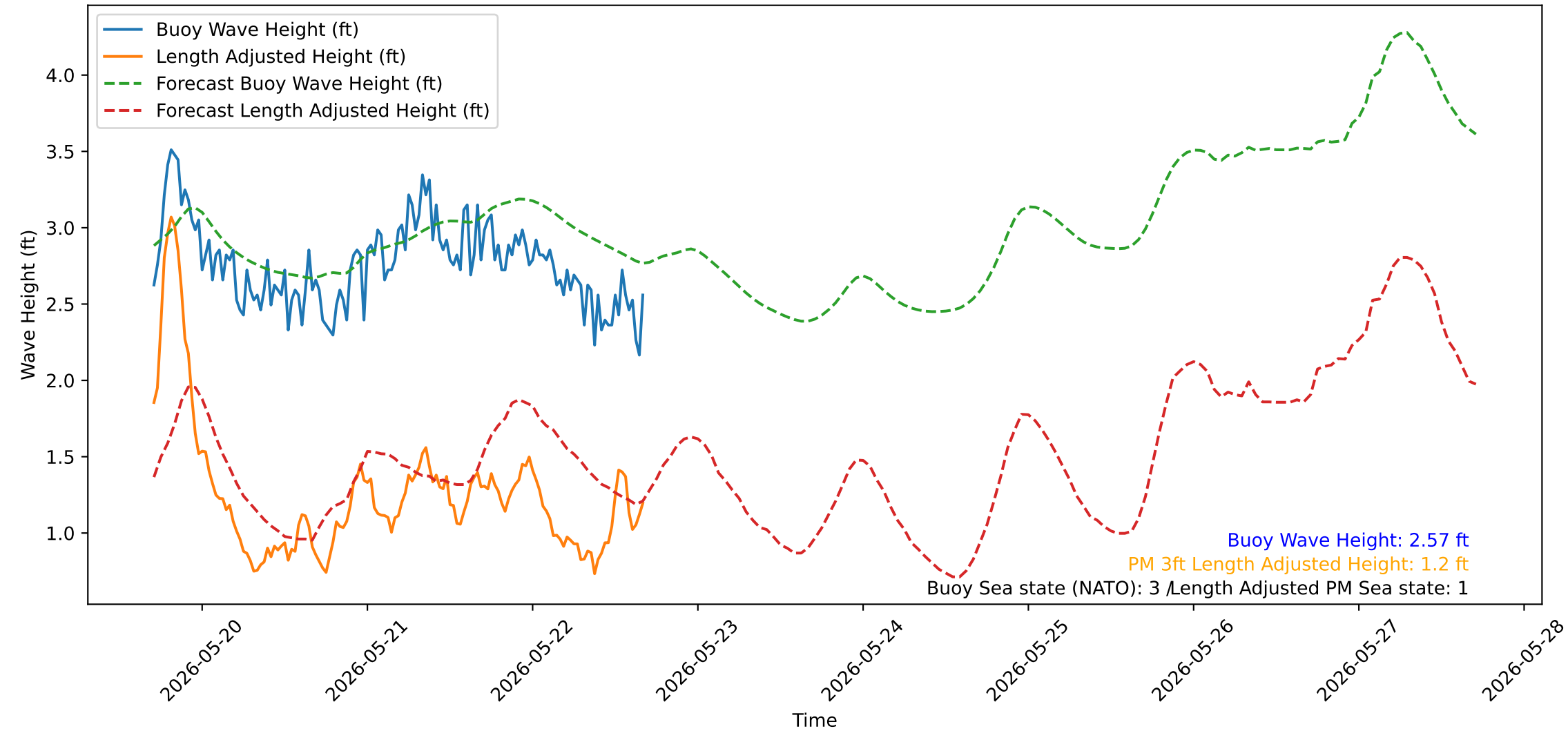
Wave Heights over Time for Red Beach at 2026-05-22 16:40:51
