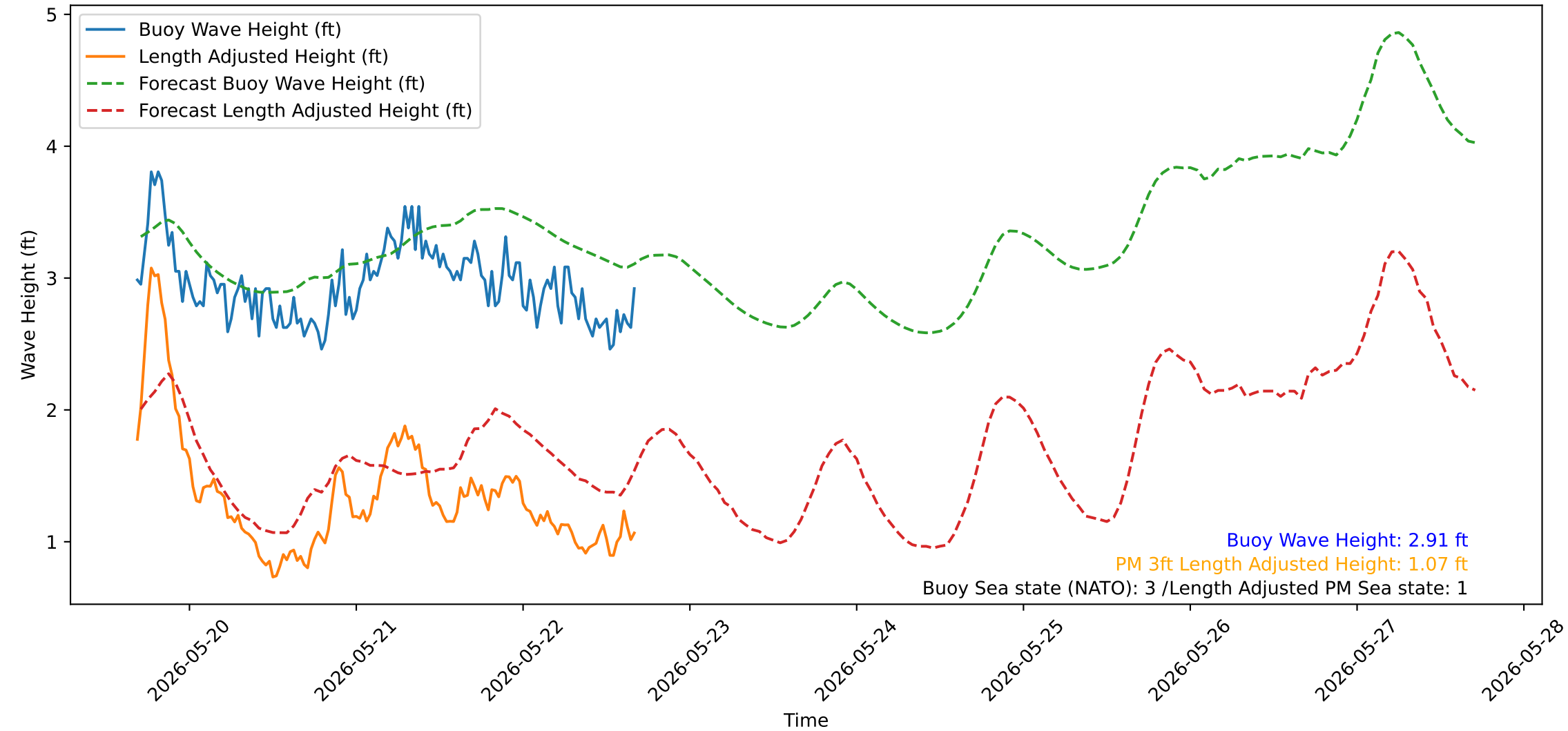
Wave Heights over Time for Green Beach at 2026-05-22 16:41:14
