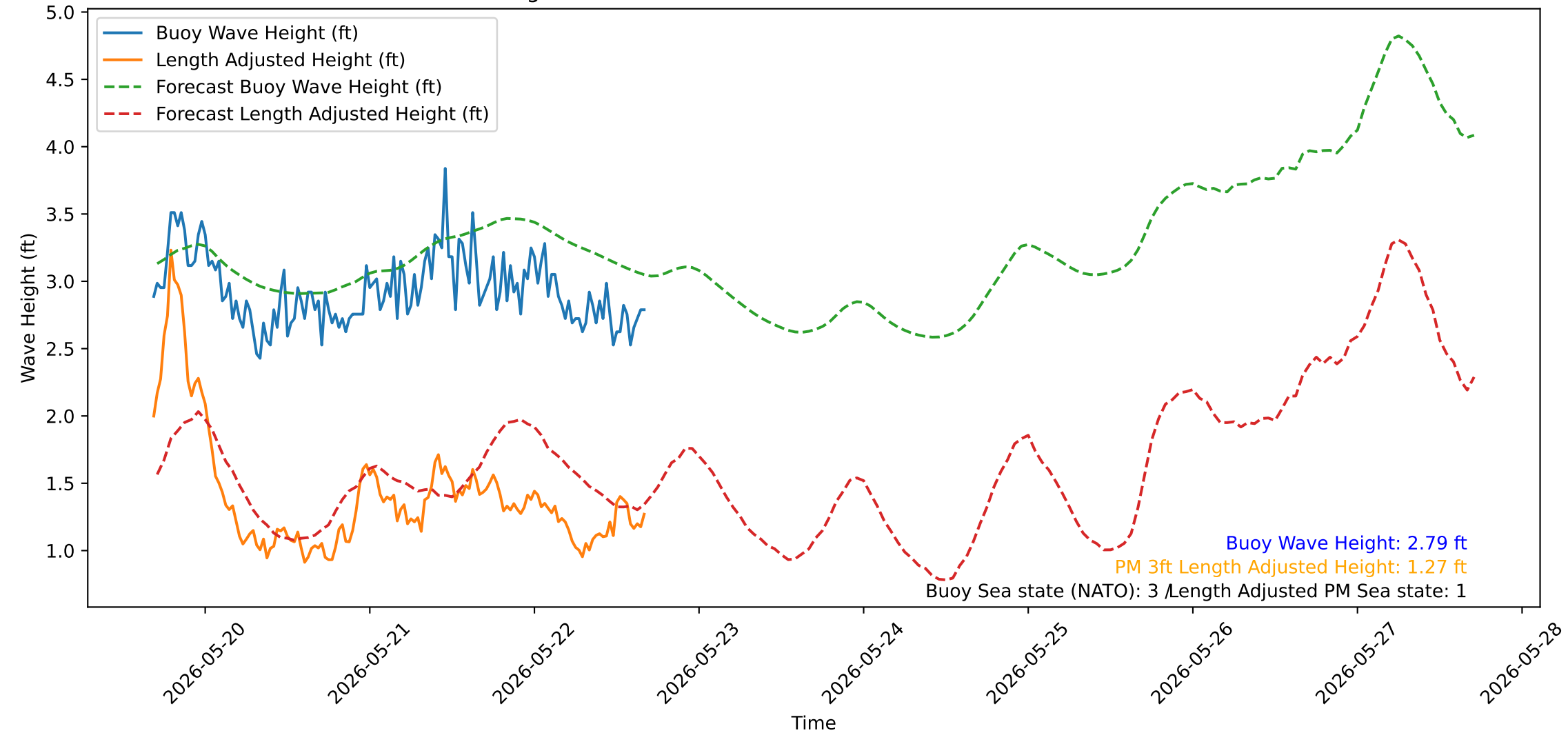
Wave Heights over Time for Oceanside Harbor at 2026-05-22 16:40:31
