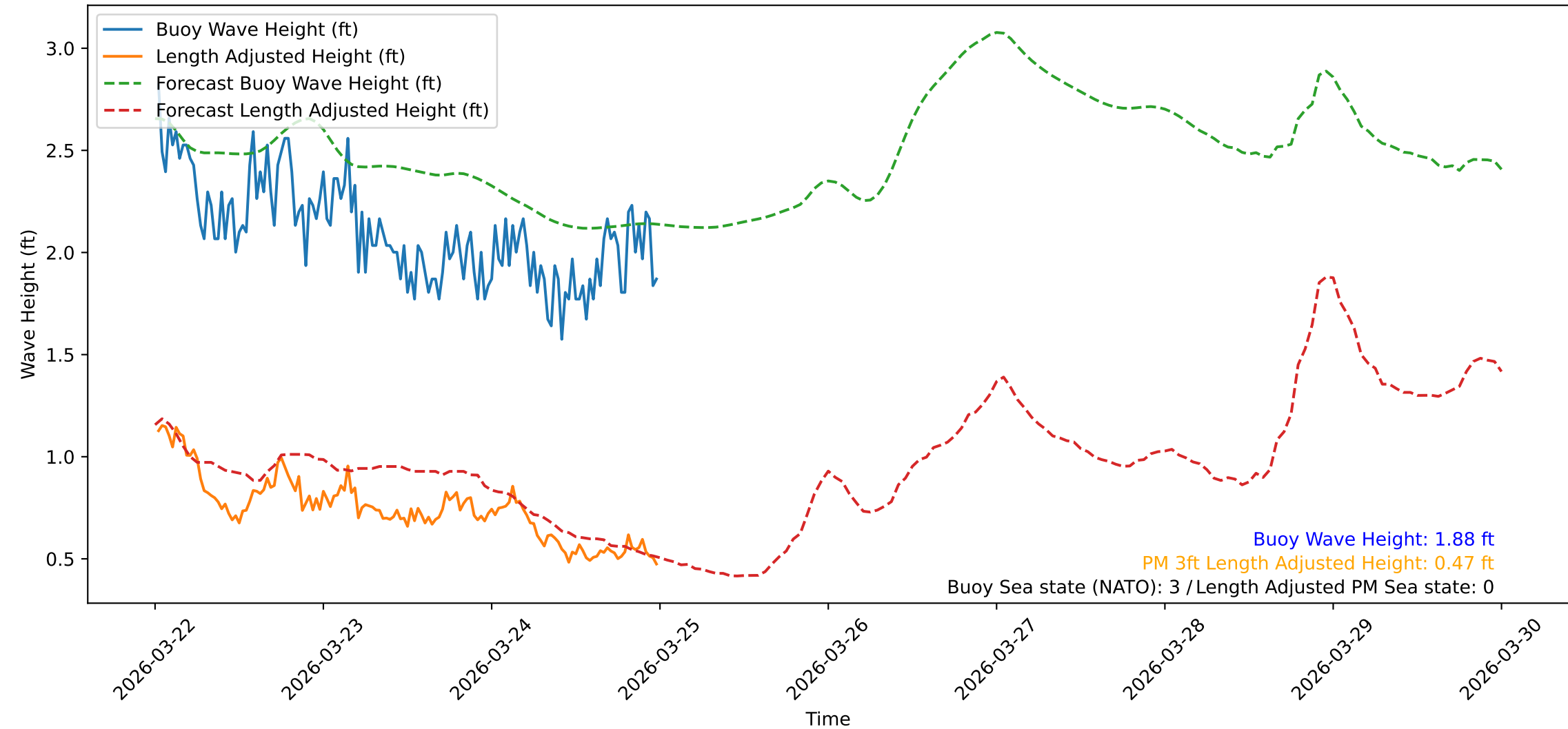
Wave Heights over Time for Oceanside Harbor at 2026-03-25 00:20:32
