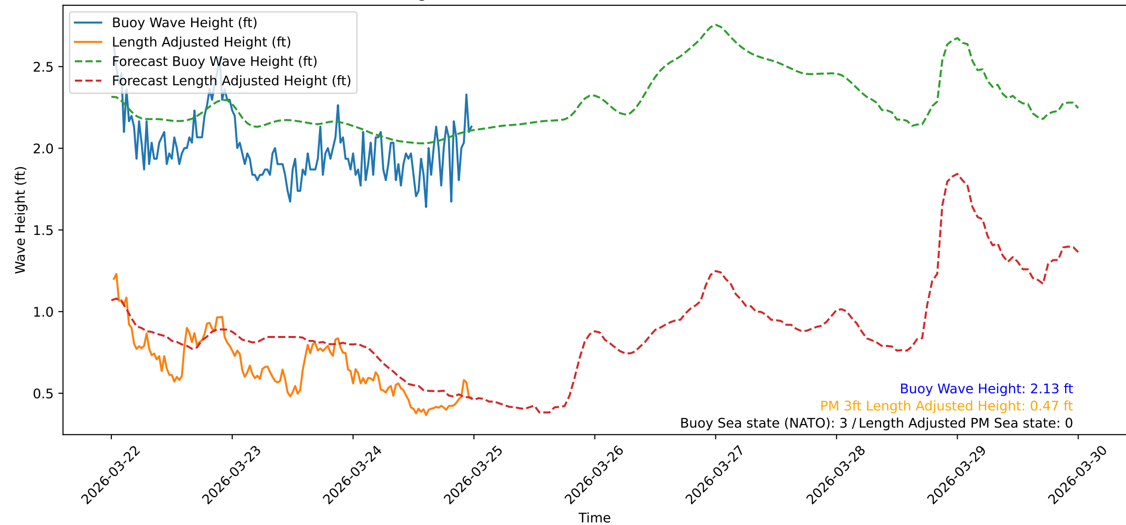
Wave Heights over Time for Red Beach at 2026-03-25 00:20:48
