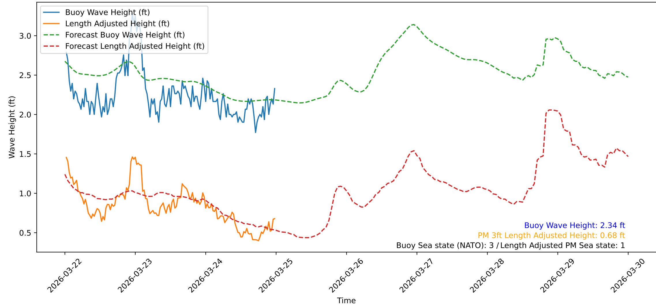
Wave Heights over Time for Green Beach at 2026-03-25 00:21:10
