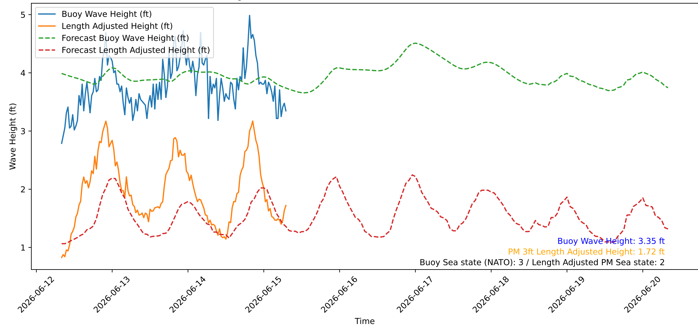
Wave Heights over Time for Oceanside Harbor at 2026-06-15 08:00:26
