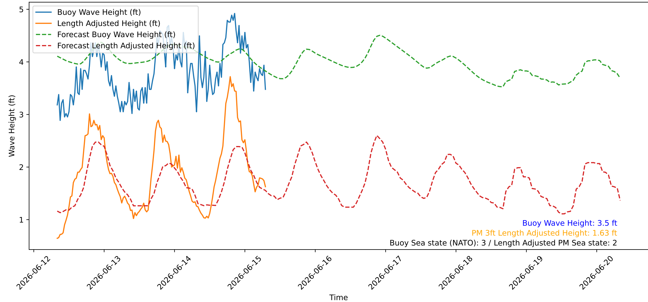
Wave Heights over Time for Green Beach at 2026-06-15 08:01:09
