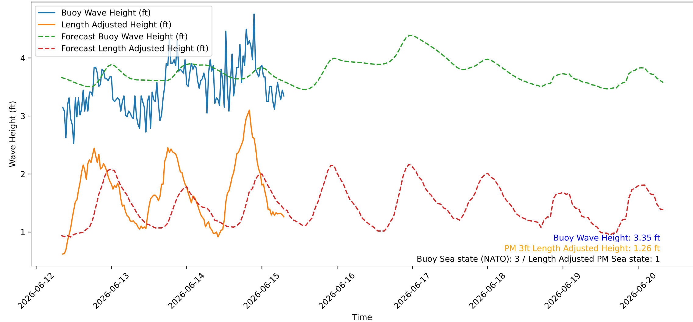
Wave Heights over Time for Red Beach at 2026-06-15 08:00:46
