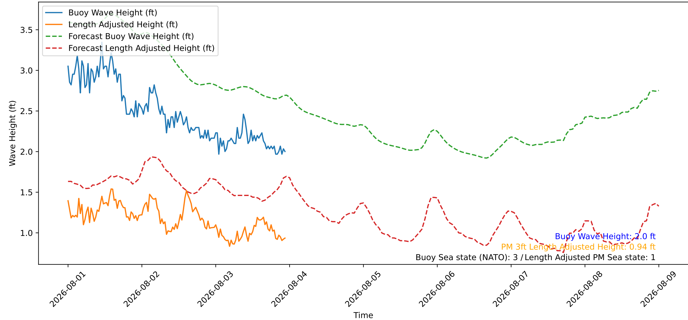
Wave Heights over Time for Red Beach at 2026-08-03 23:30:45
