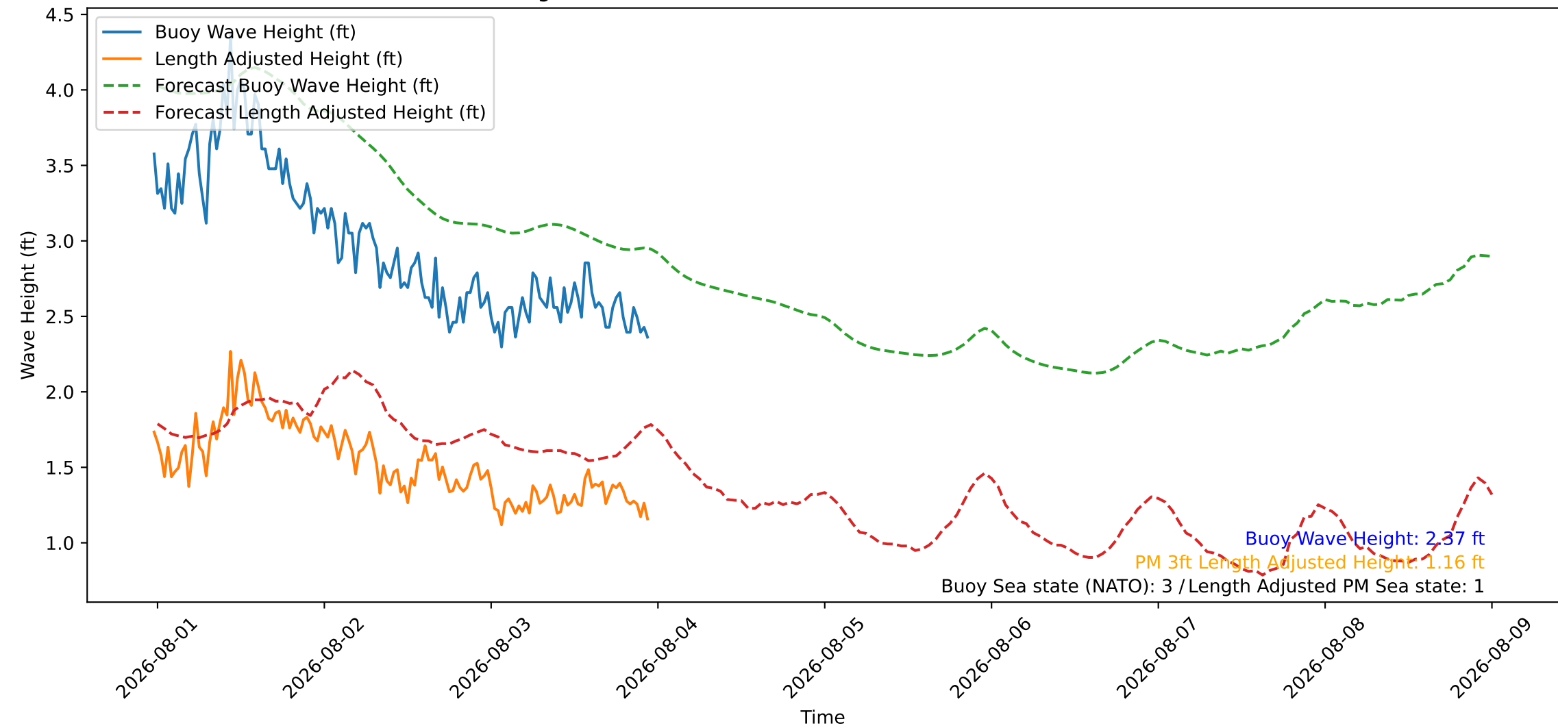
Wave Heights over Time for Oceanside Harbor at 2026-08-03 23:30:25
