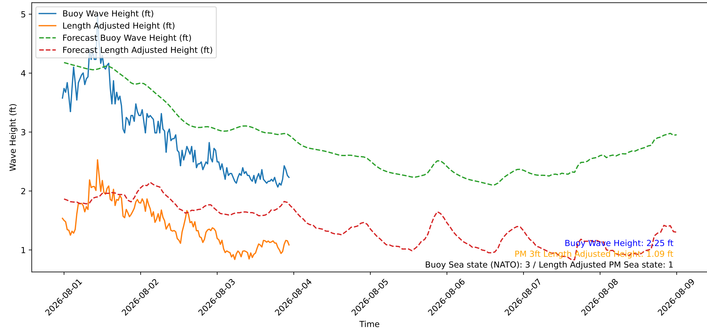
Wave Heights over Time for Green Beach at 2026-08-03 23:31:07
