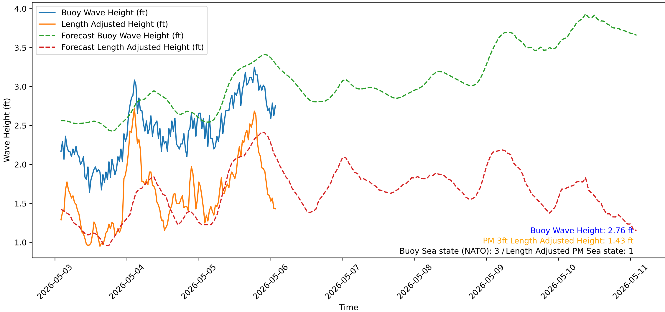
Wave Heights over Time for Oceanside Harbor at 2026-05-06 02:10:31
