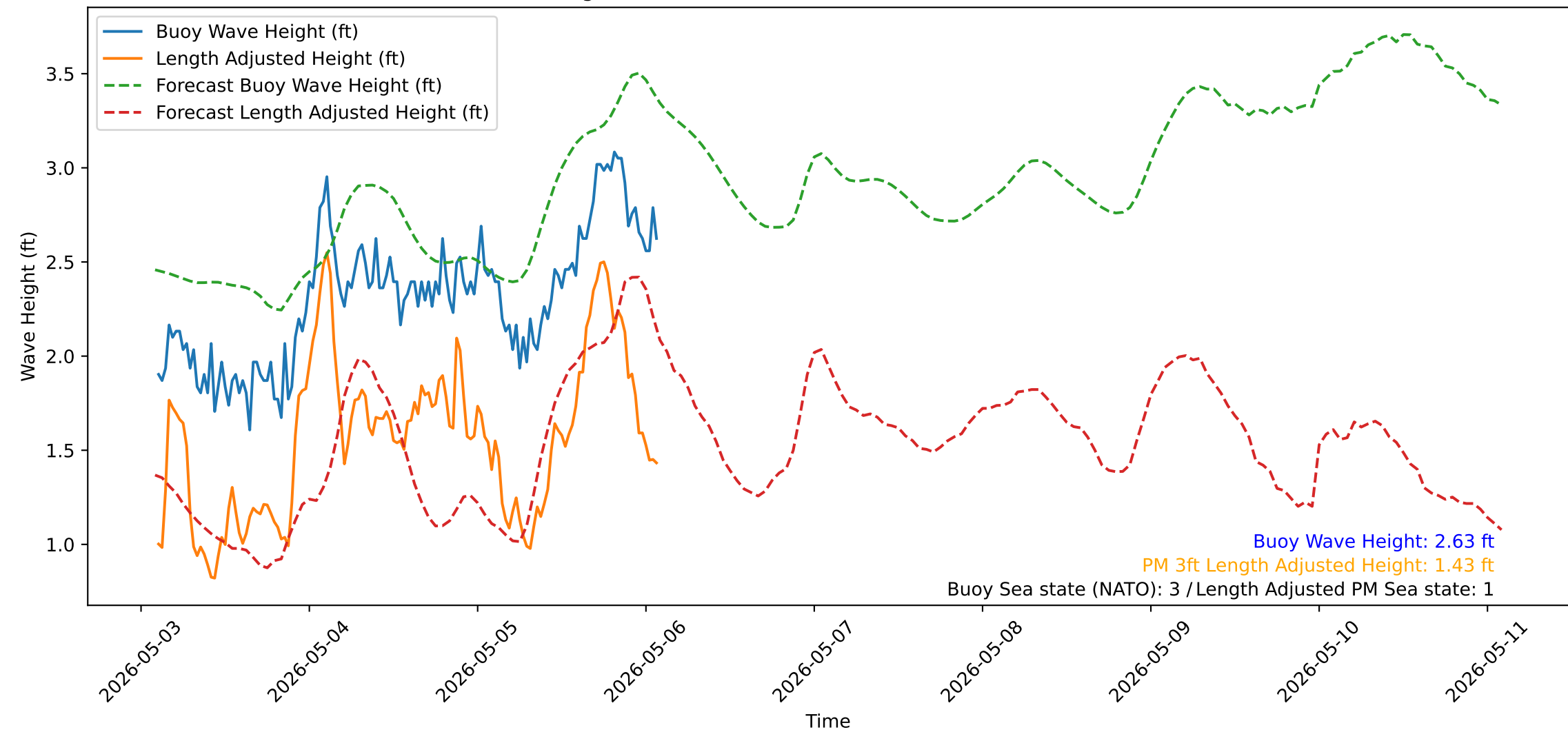
Wave Heights over Time for Red Beach at 2026-05-06 02:10:51
