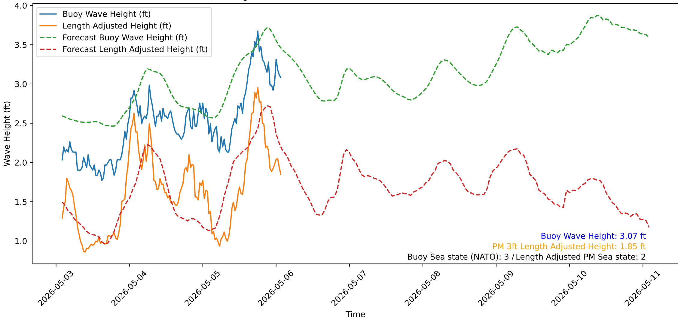
Wave Heights over Time for Green Beach at 2026-05-06 02:11:13
