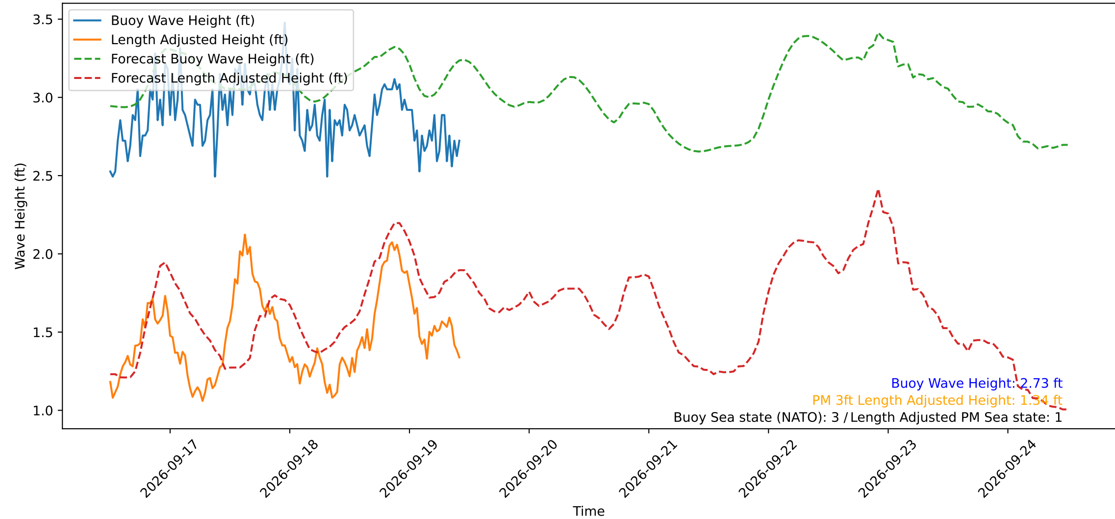
Wave Heights over Time for Green Beach at 2026-09-19 11:31:10
