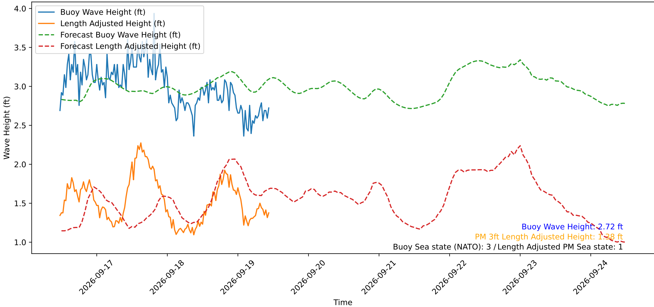
Wave Heights over Time for Oceanside Harbor at 2026-09-19 11:30:29
