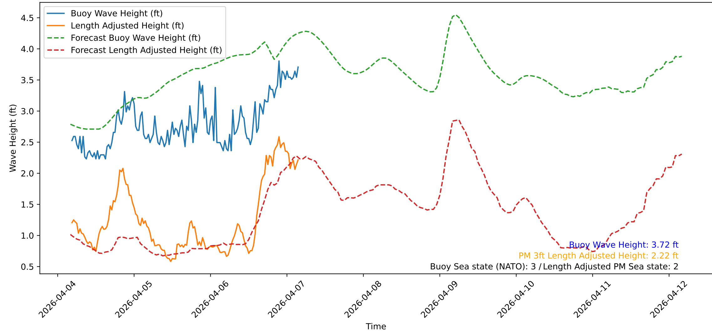
Wave Heights over Time for Green Beach at 2026-04-07 04:21:11
