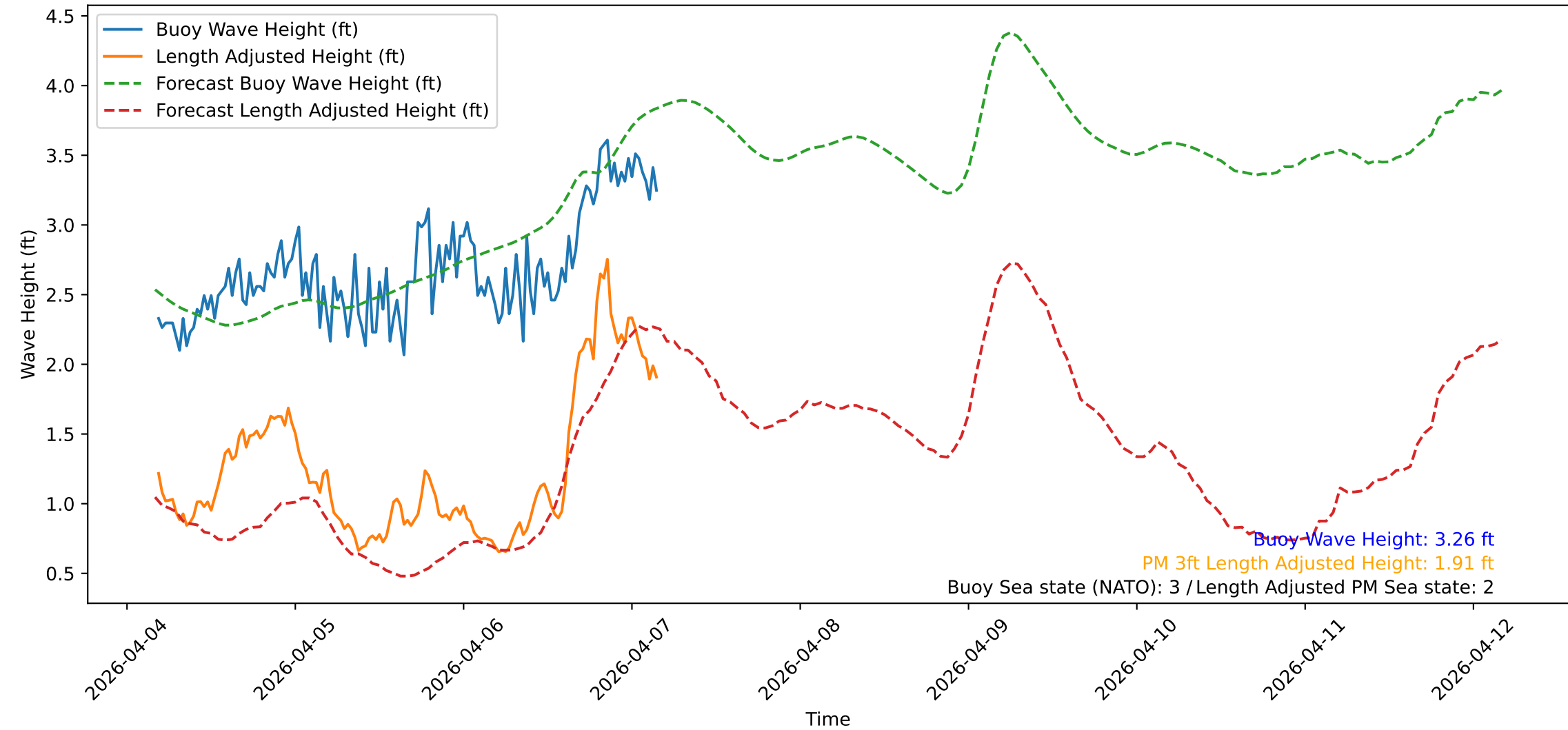
Wave Heights over Time for Oceanside Harbor at 2026-04-07 04:20:31
