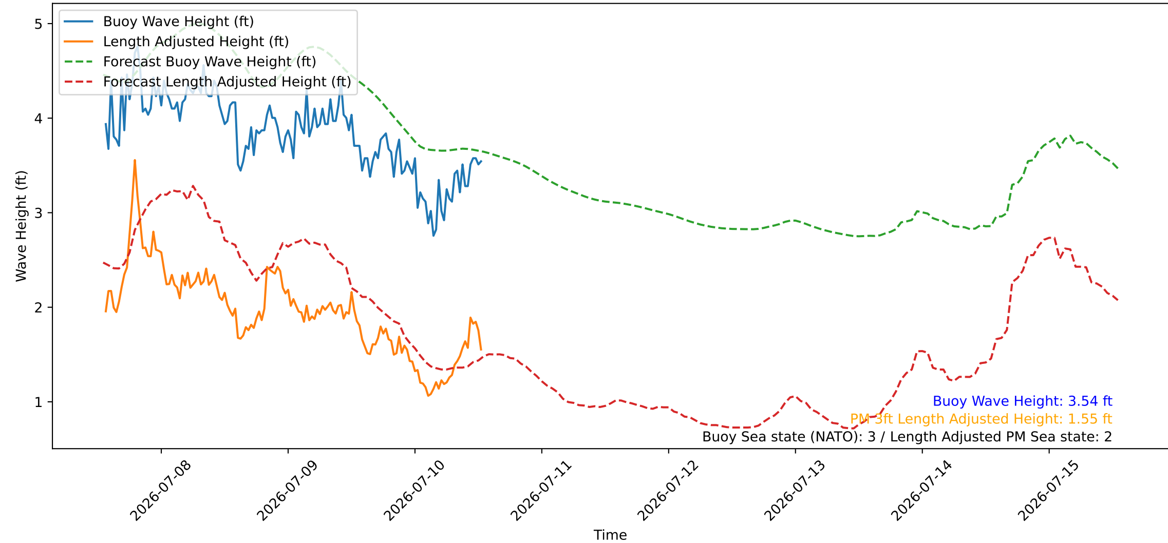
Wave Heights over Time for Green Beach at 2026-07-10 13:21:09
