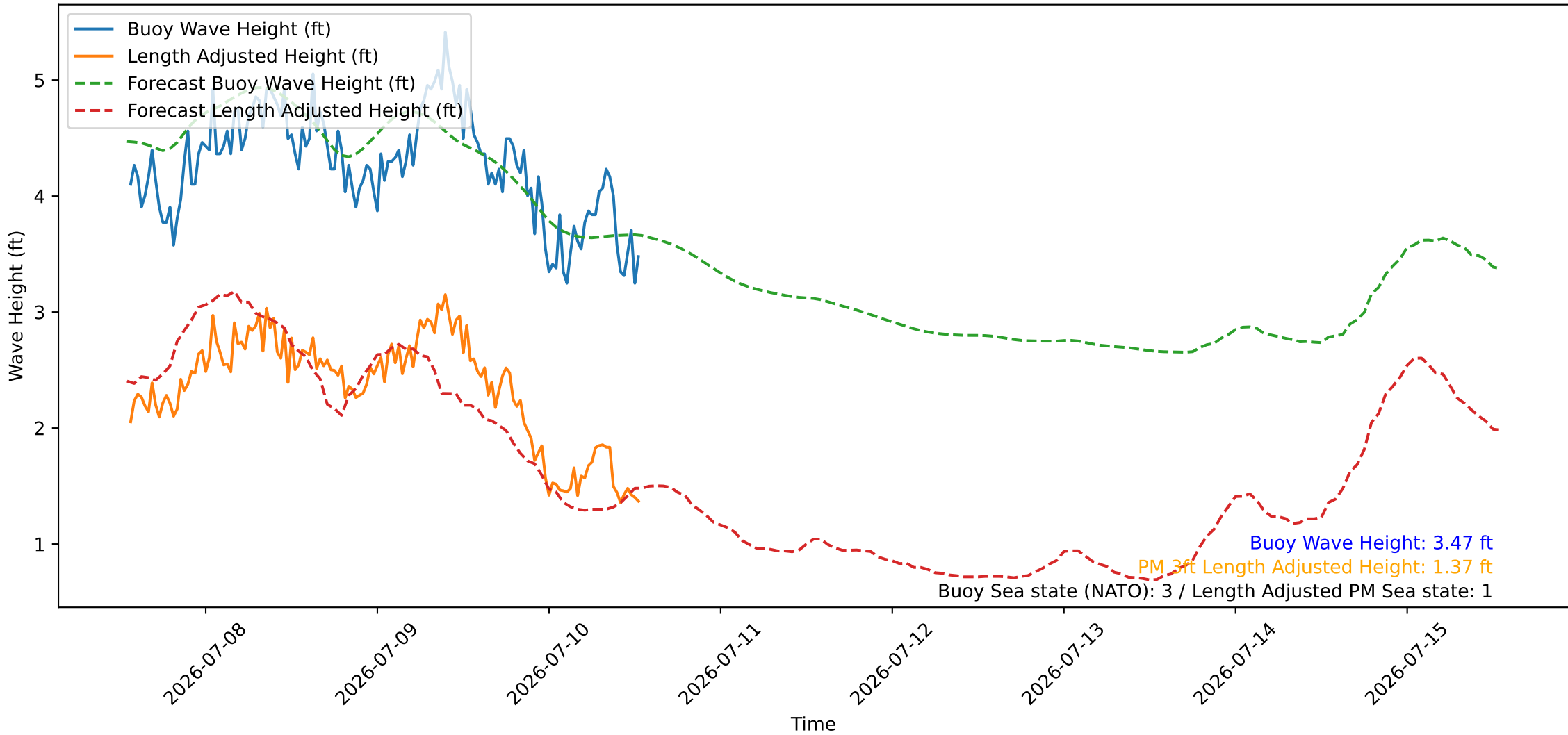
Wave Heights over Time for Oceanside Harbor at 2026-07-10 13:20:26
