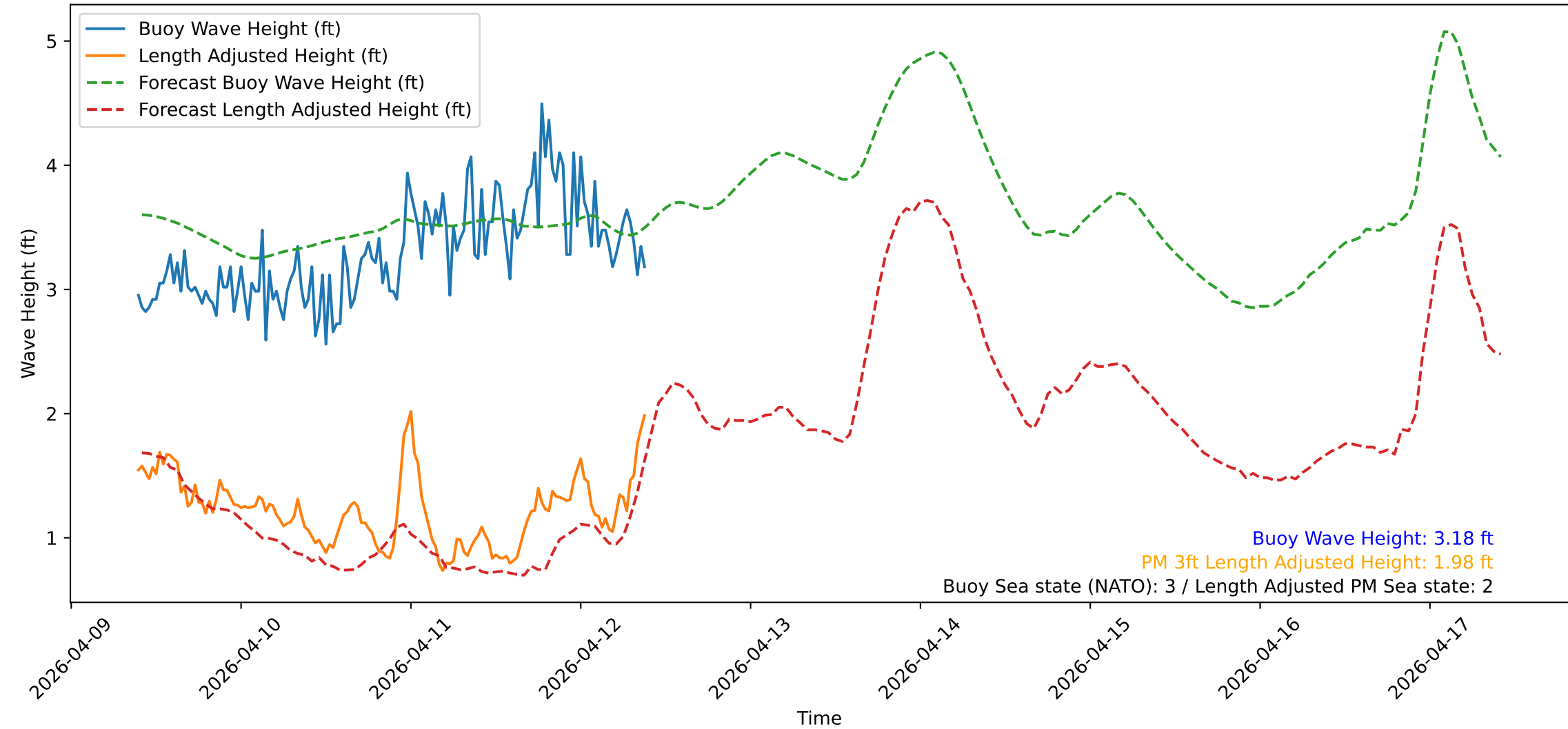
Wave Heights over Time for Green Beach at 2026-04-12 09:41:13
