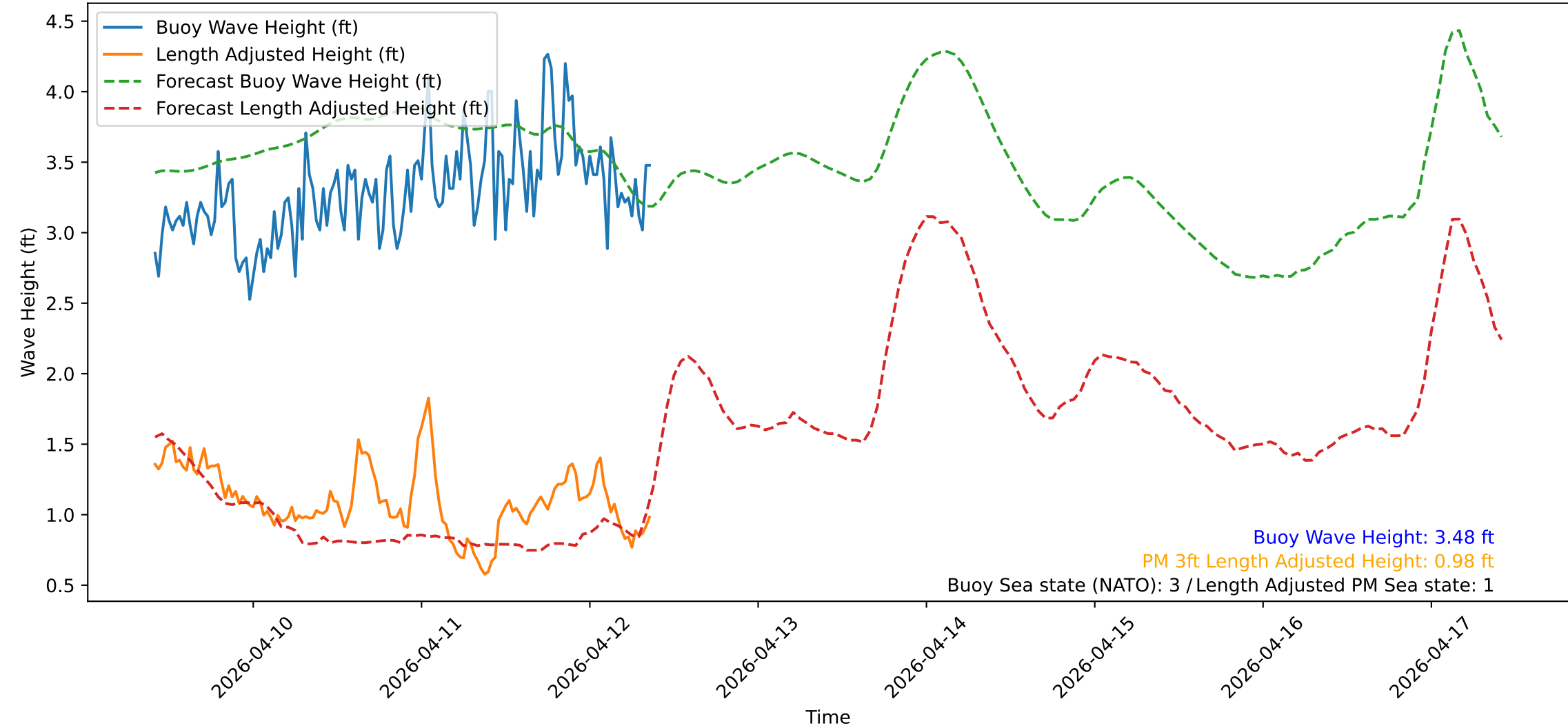
Wave Heights over Time for Red Beach at 2026-04-12 09:40:50
