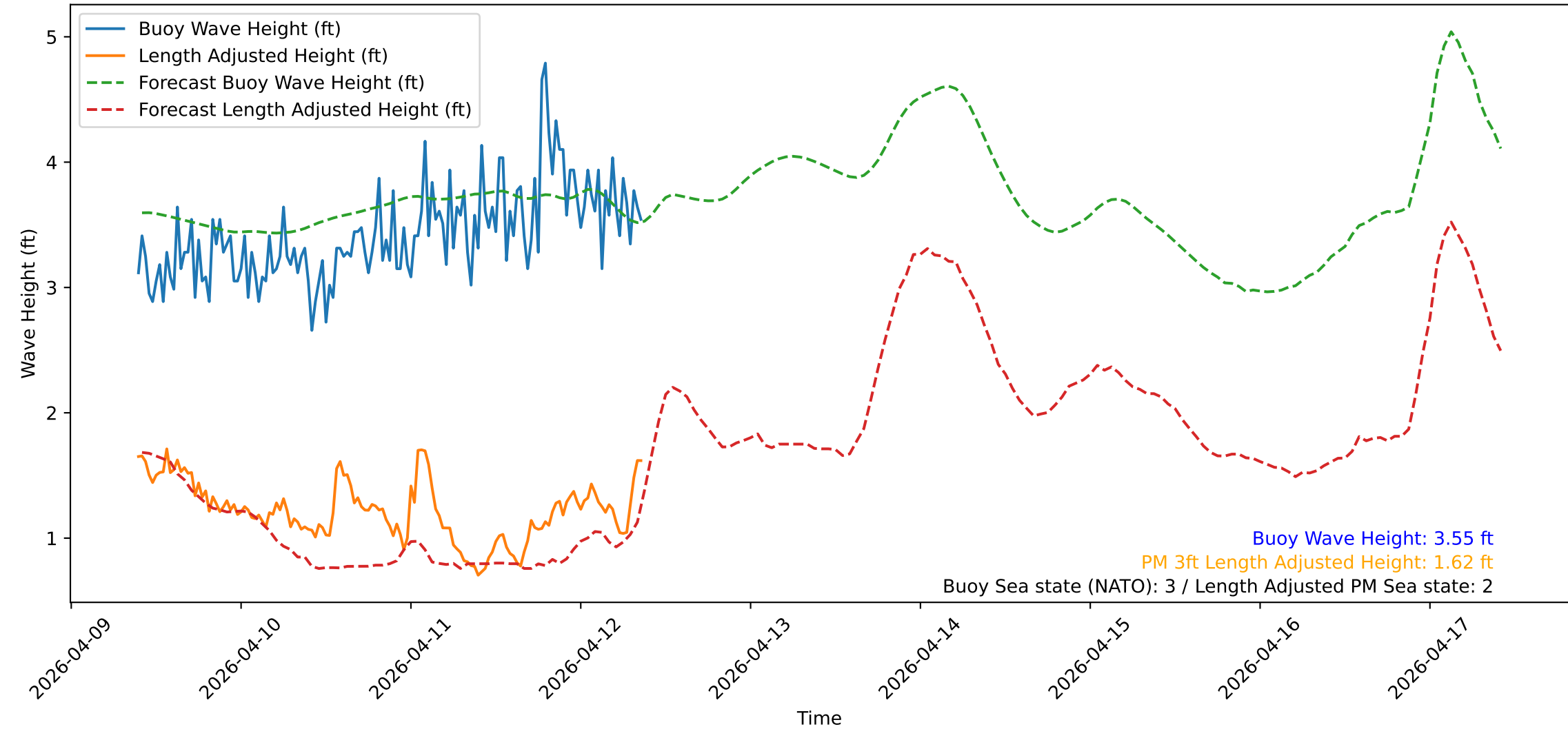
Wave Heights over Time for Oceanside Harbor at 2026-04-12 09:40:32
