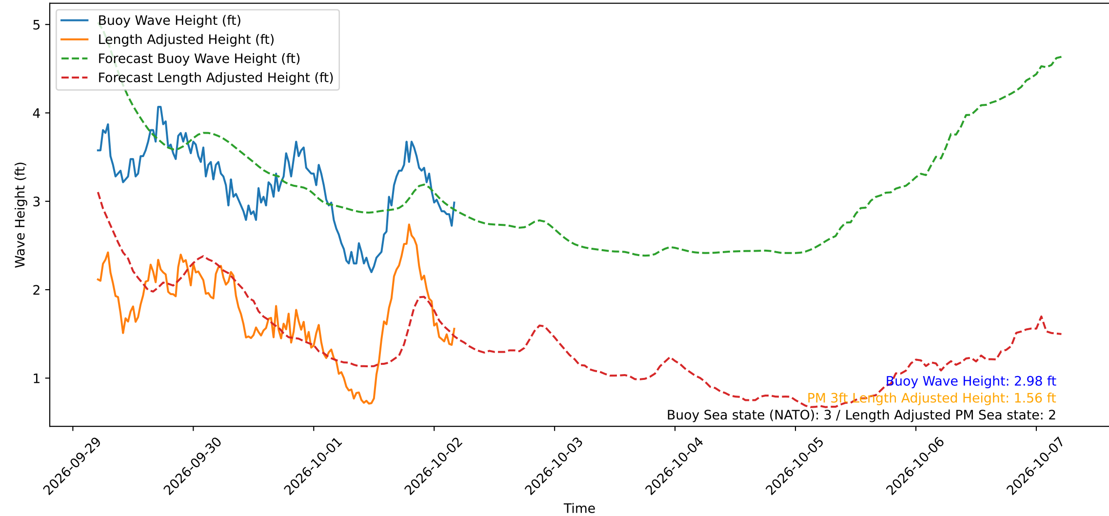
Wave Heights over Time for Green Beach at 2026-10-02 04:51:14
