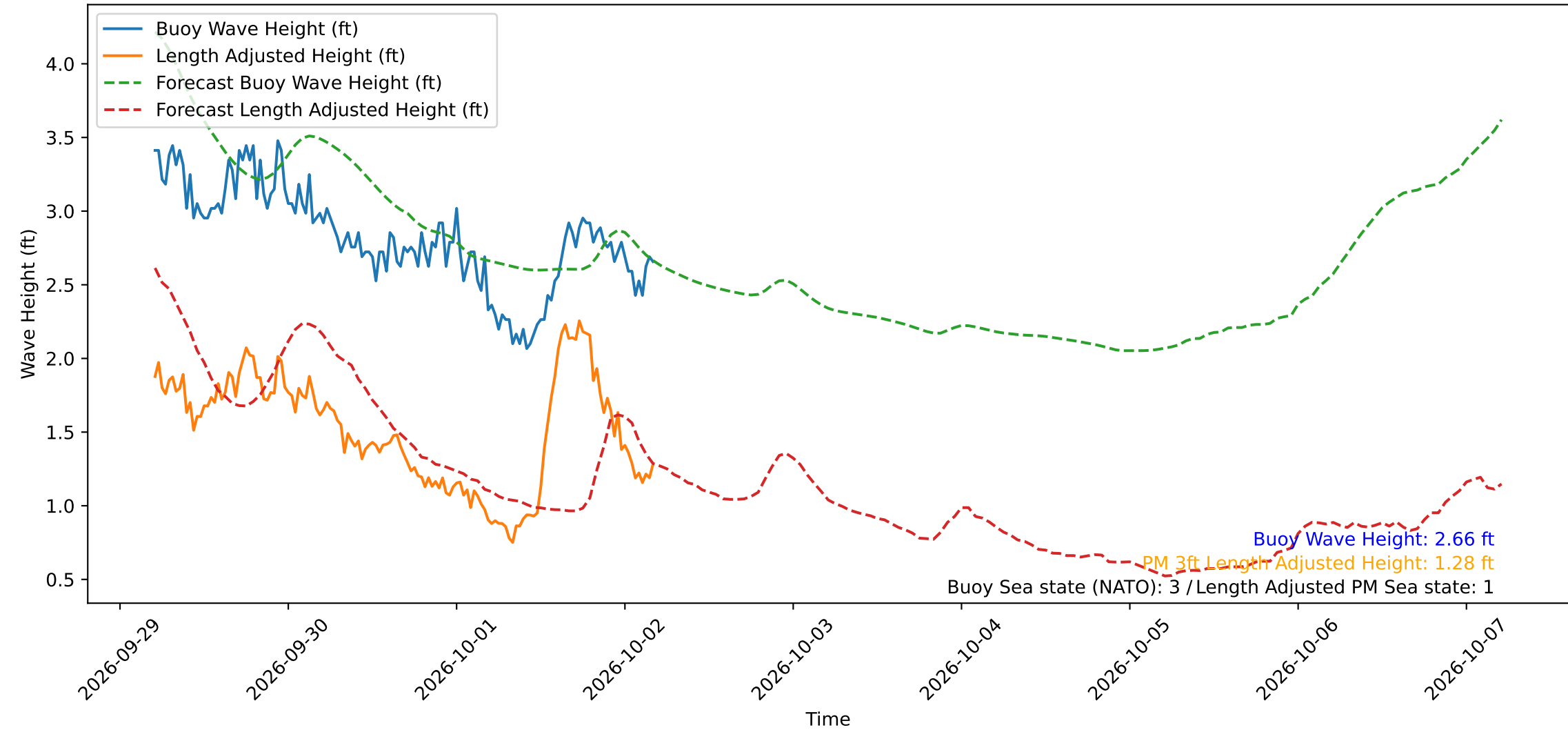
Wave Heights over Time for Red Beach at 2026-10-02 04:50:50
