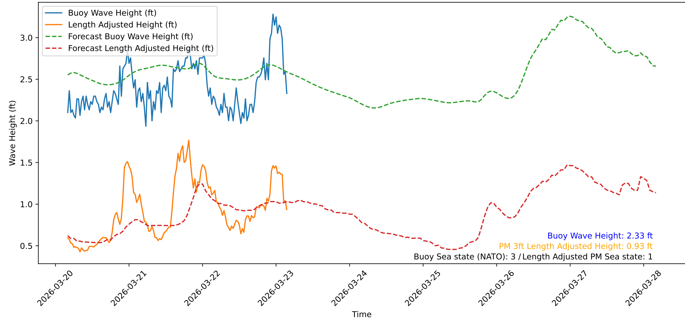
Wave Heights over Time for Green Beach at 2026-03-23 04:11:10
