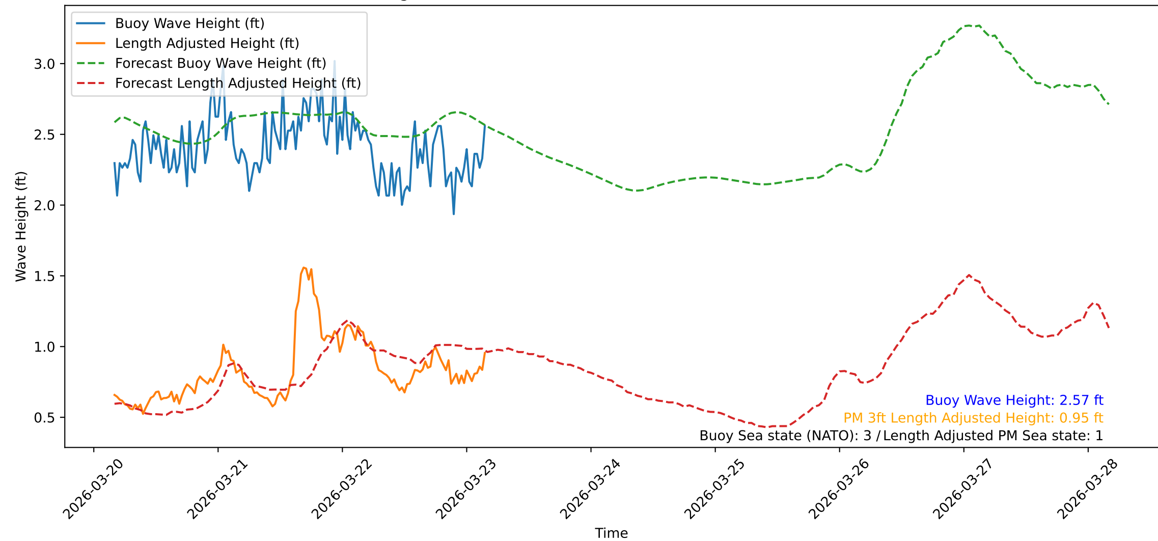
Wave Heights over Time for Oceanside Harbor at 2026-03-23 04:10:31
