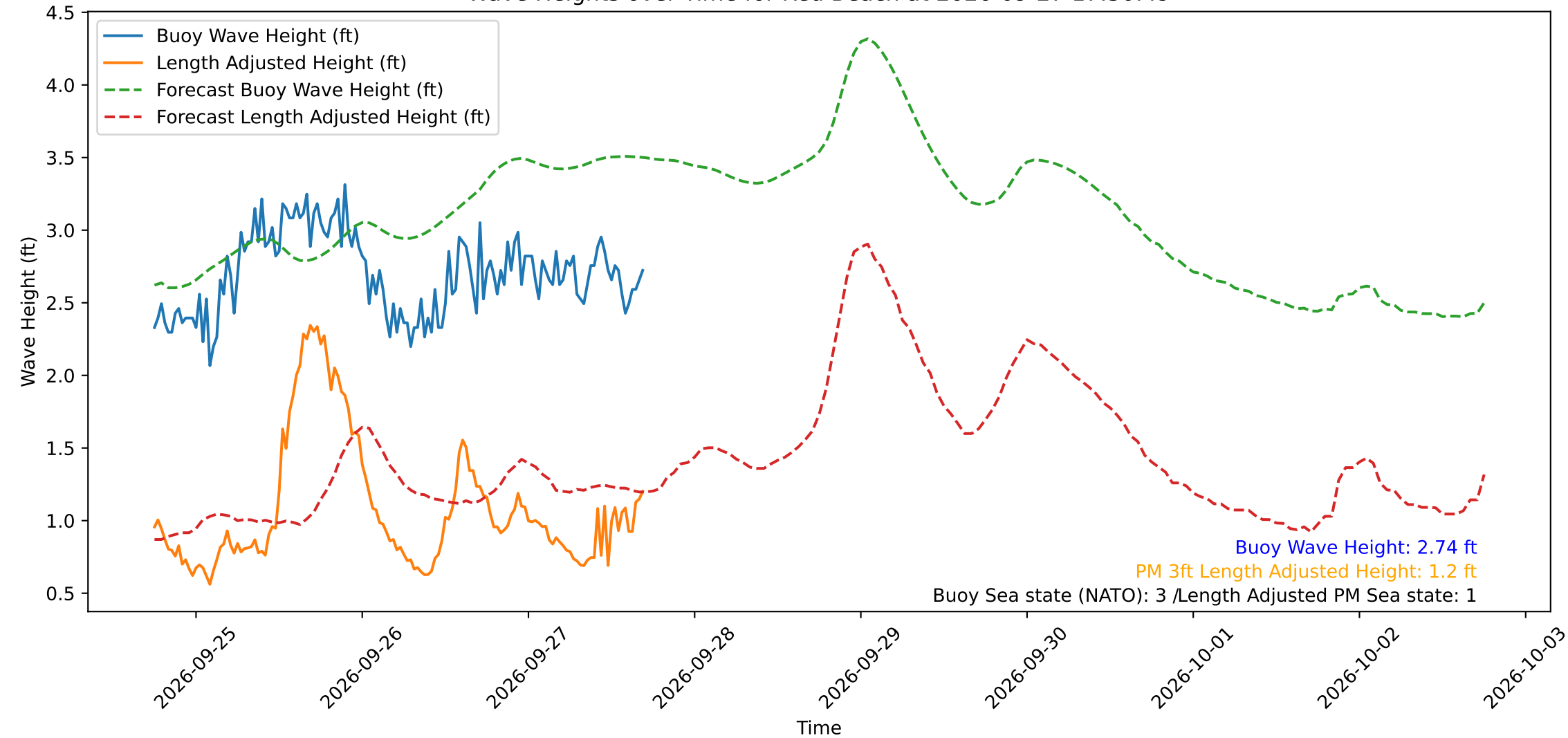
Wave Heights over Time for Red Beach at 2026-09-27 17:30:49
