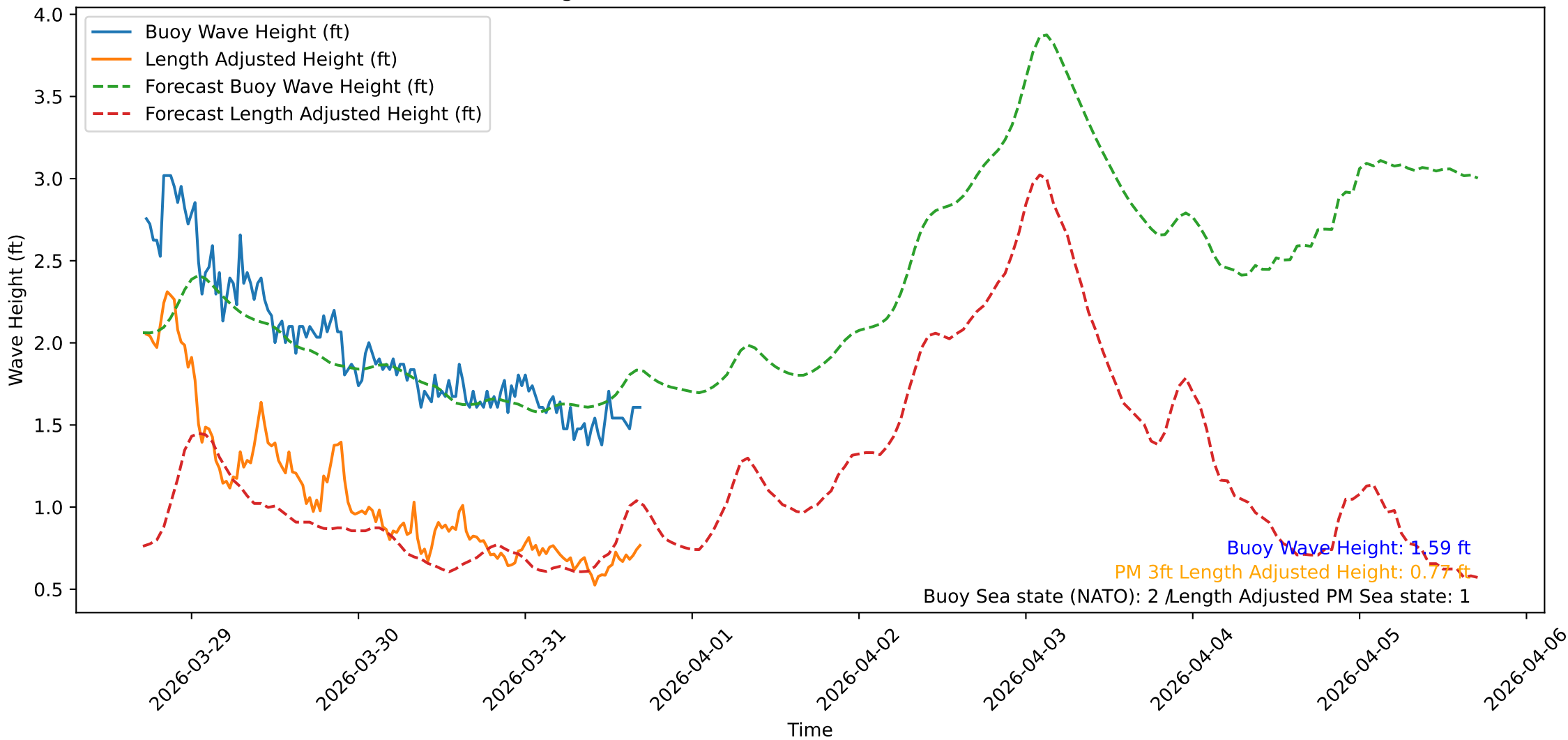
Wave Heights over Time for Red Beach at 2026-03-31 17:20:47
