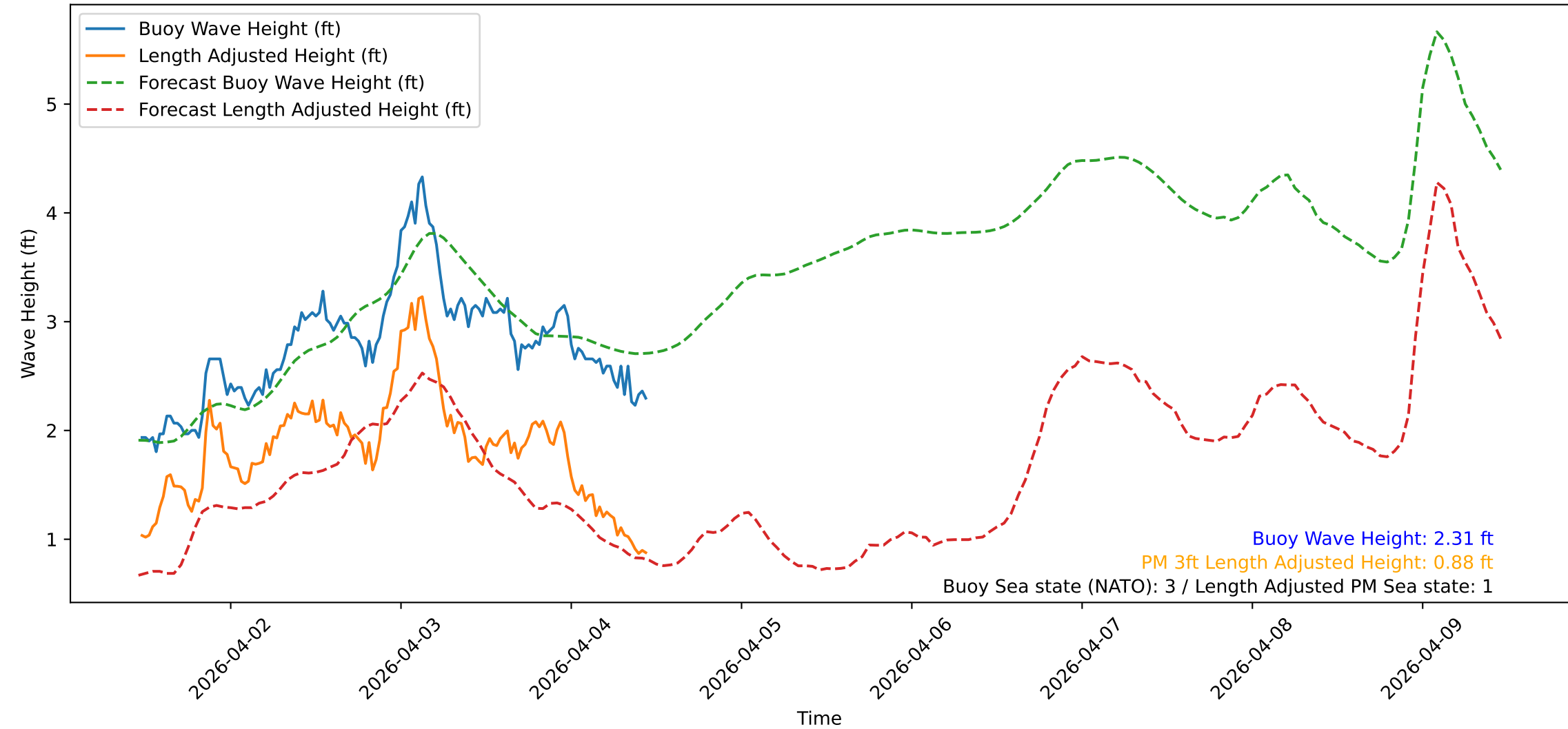
Wave Heights over Time for Green Beach at 2026-04-04 11:21:10
