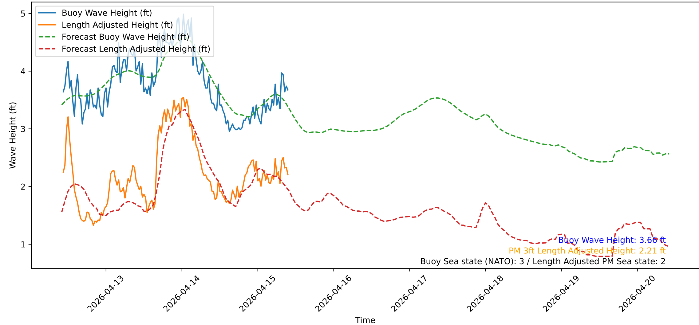
Wave Heights over Time for Green Beach at 2026-04-15 10:21:14
