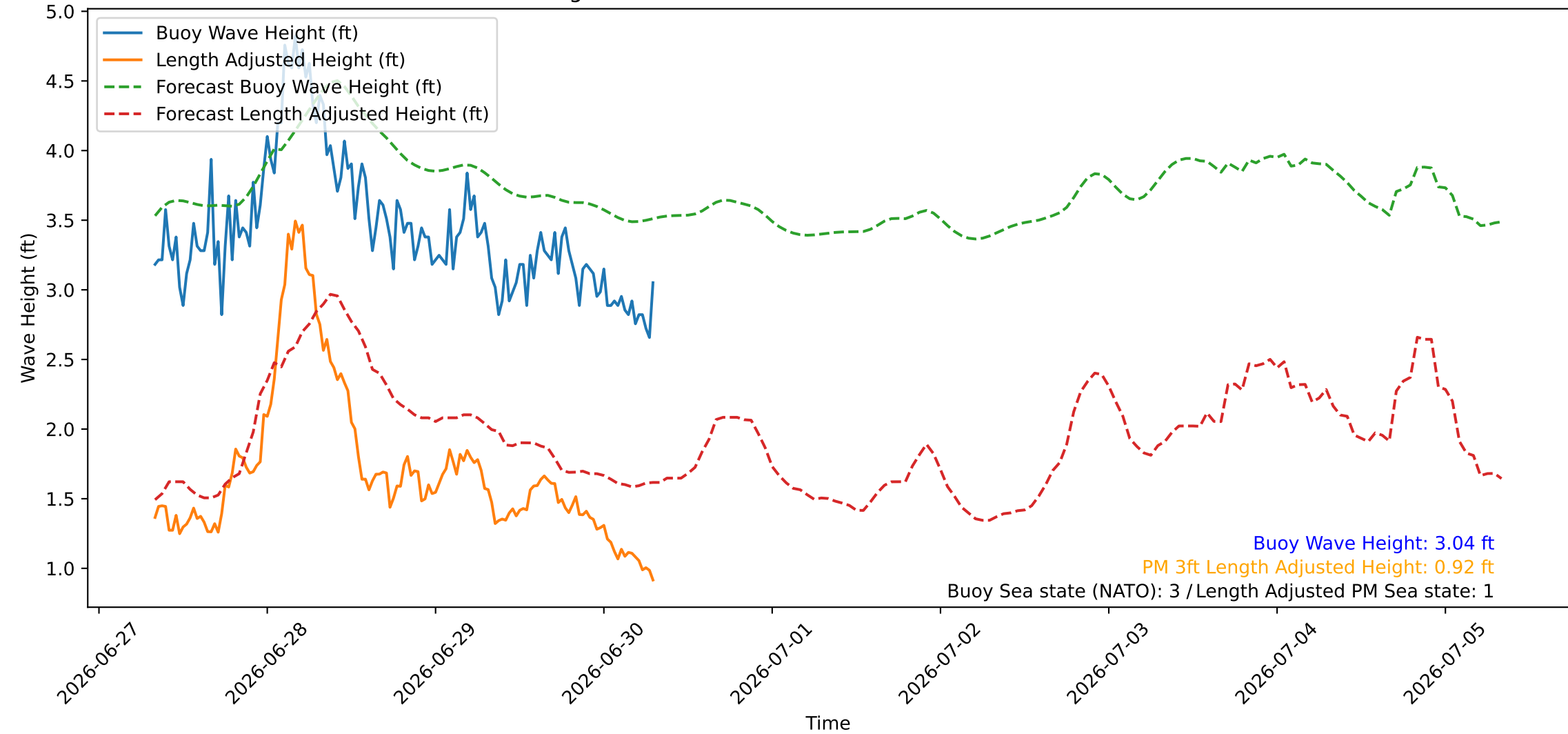
Wave Heights over Time for Green Beach at 2026-06-30 07:51:09
