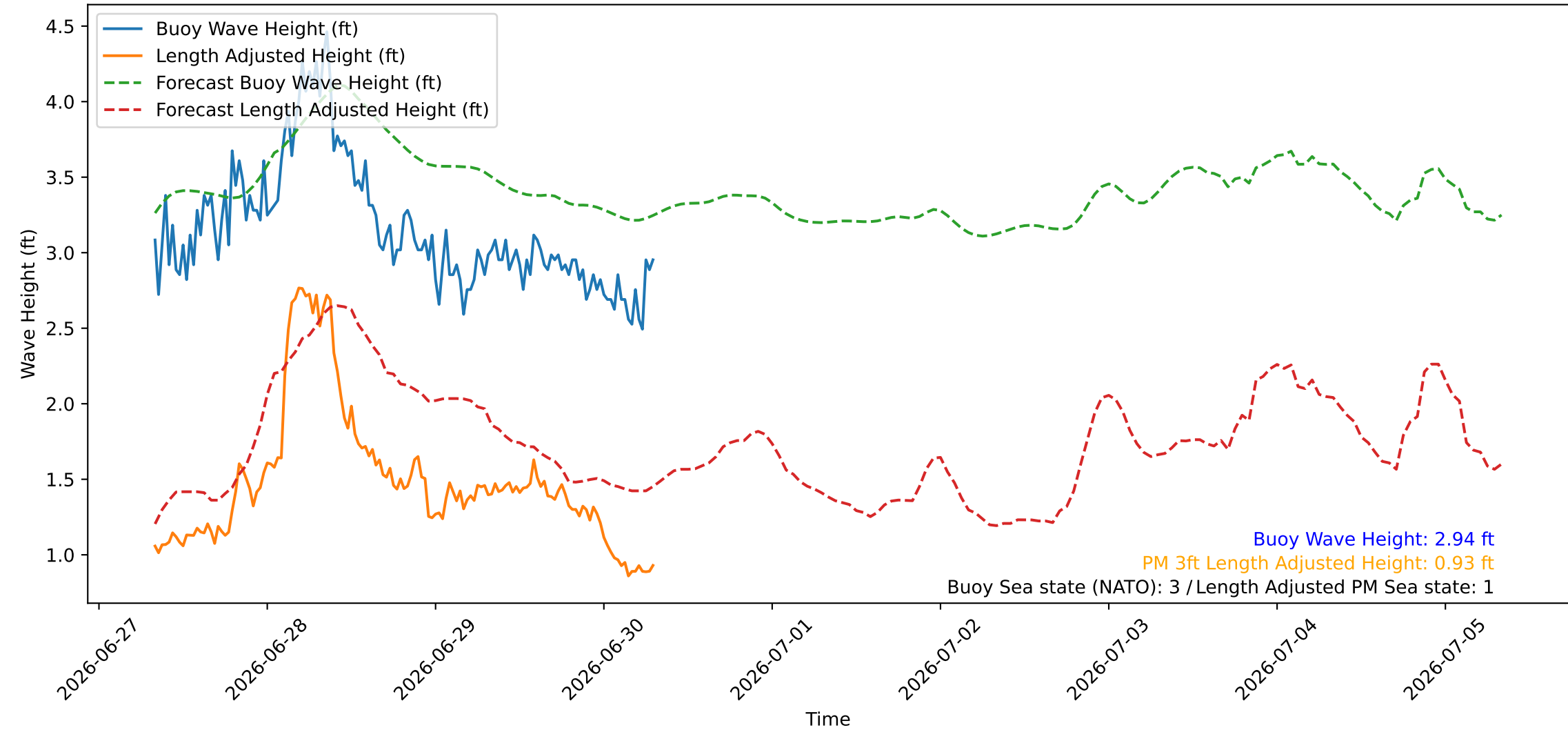
Wave Heights over Time for Red Beach at 2026-06-30 07:50:47
