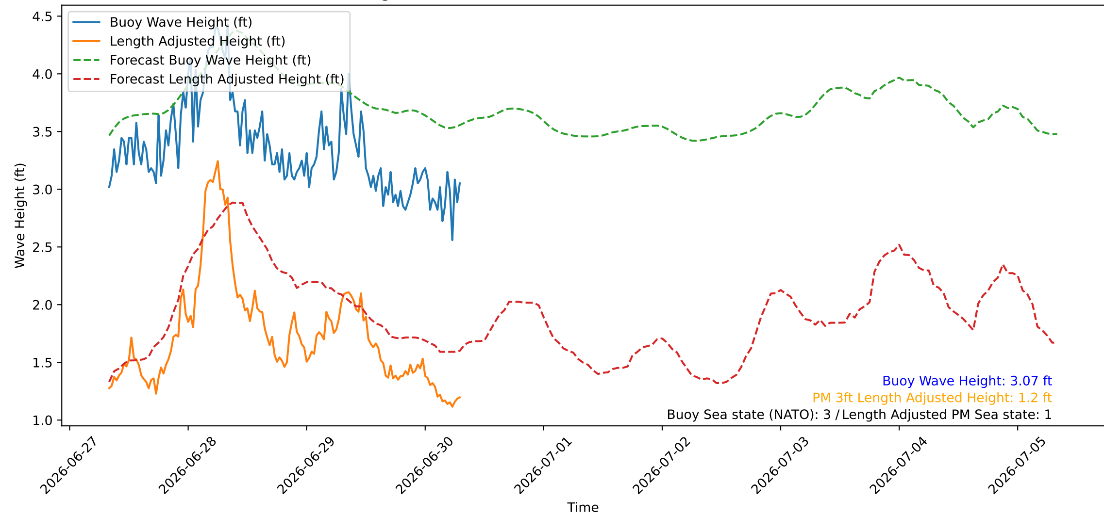
Wave Heights over Time for Oceanside Harbor at 2026-06-30 07:50:26
