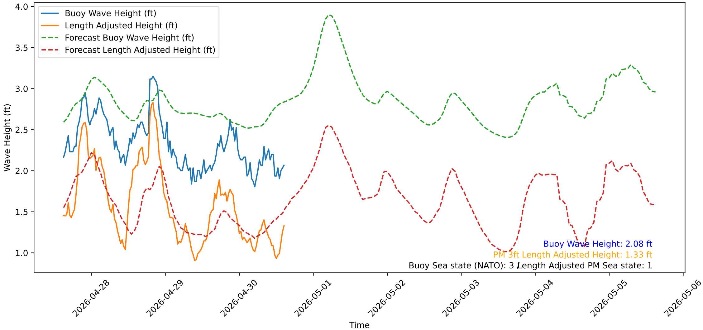
Wave Heights over Time for Green Beach at 2026-04-30 15:11:13
