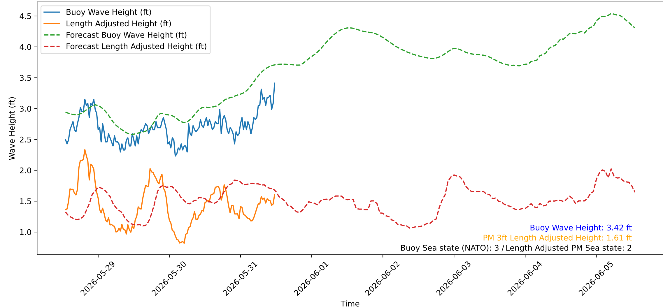
Wave Heights over Time for Red Beach at 2026-05-31 12:40:46
