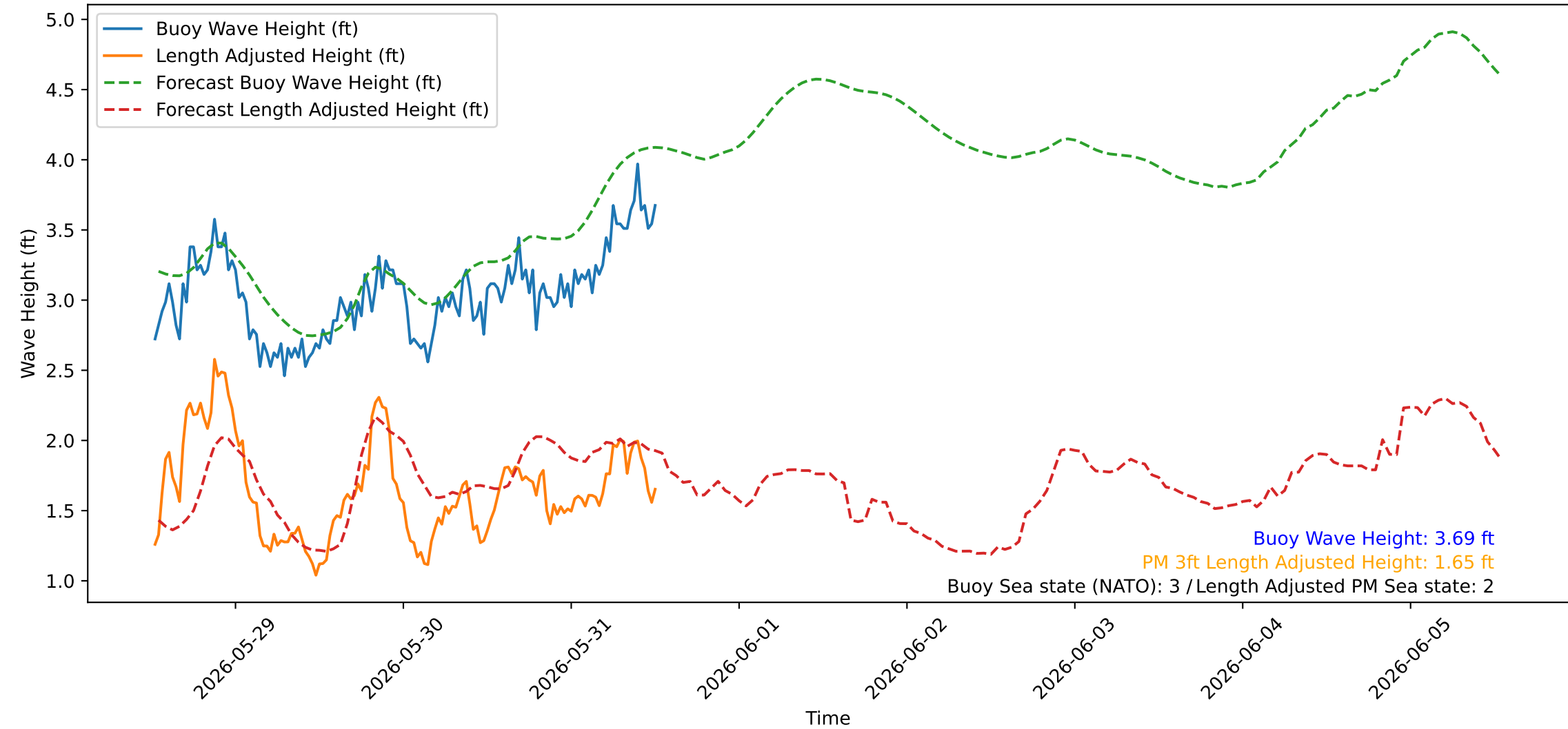
Wave Heights over Time for Green Beach at 2026-05-31 12:41:09
