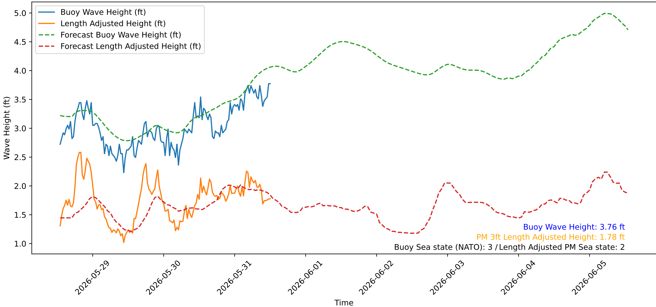
Wave Heights over Time for Oceanside Harbor at 2026-05-31 12:40:26
