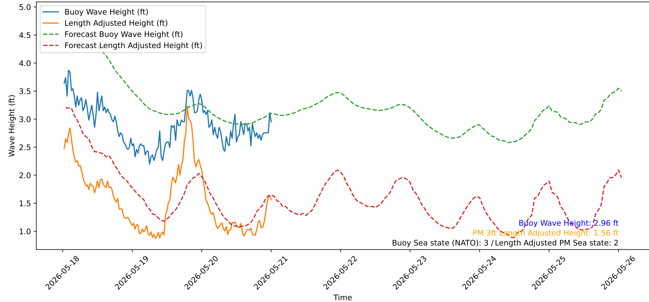
Wave Heights over Time for Oceanside Harbor at 2026-05-21 00:40:32
