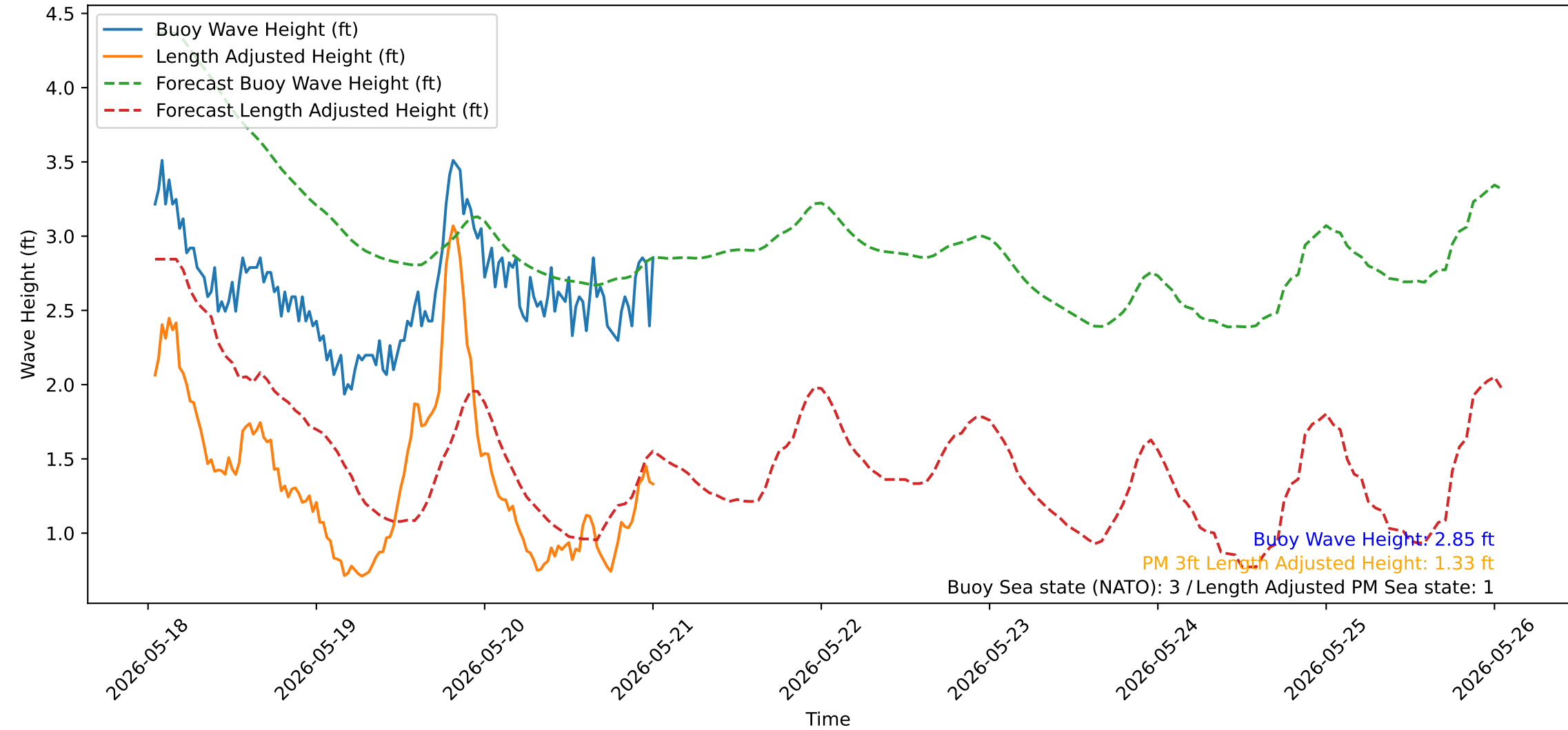
Wave Heights over Time for Red Beach at 2026-05-21 00:40:51
