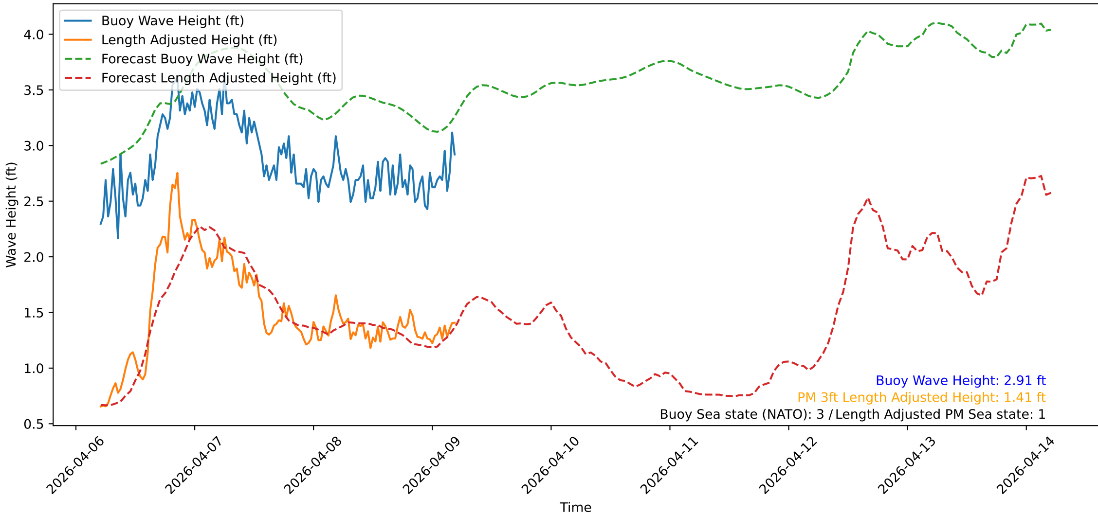
Wave Heights over Time for Oceanside Harbor at 2026-04-09 05:10:30
