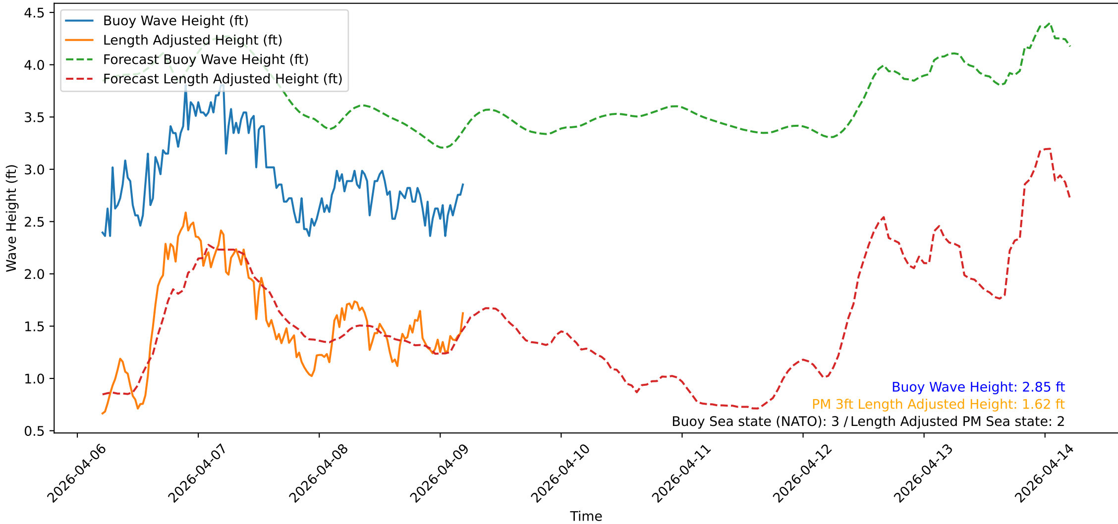
Wave Heights over Time for Green Beach at 2026-04-09 05:11:08
