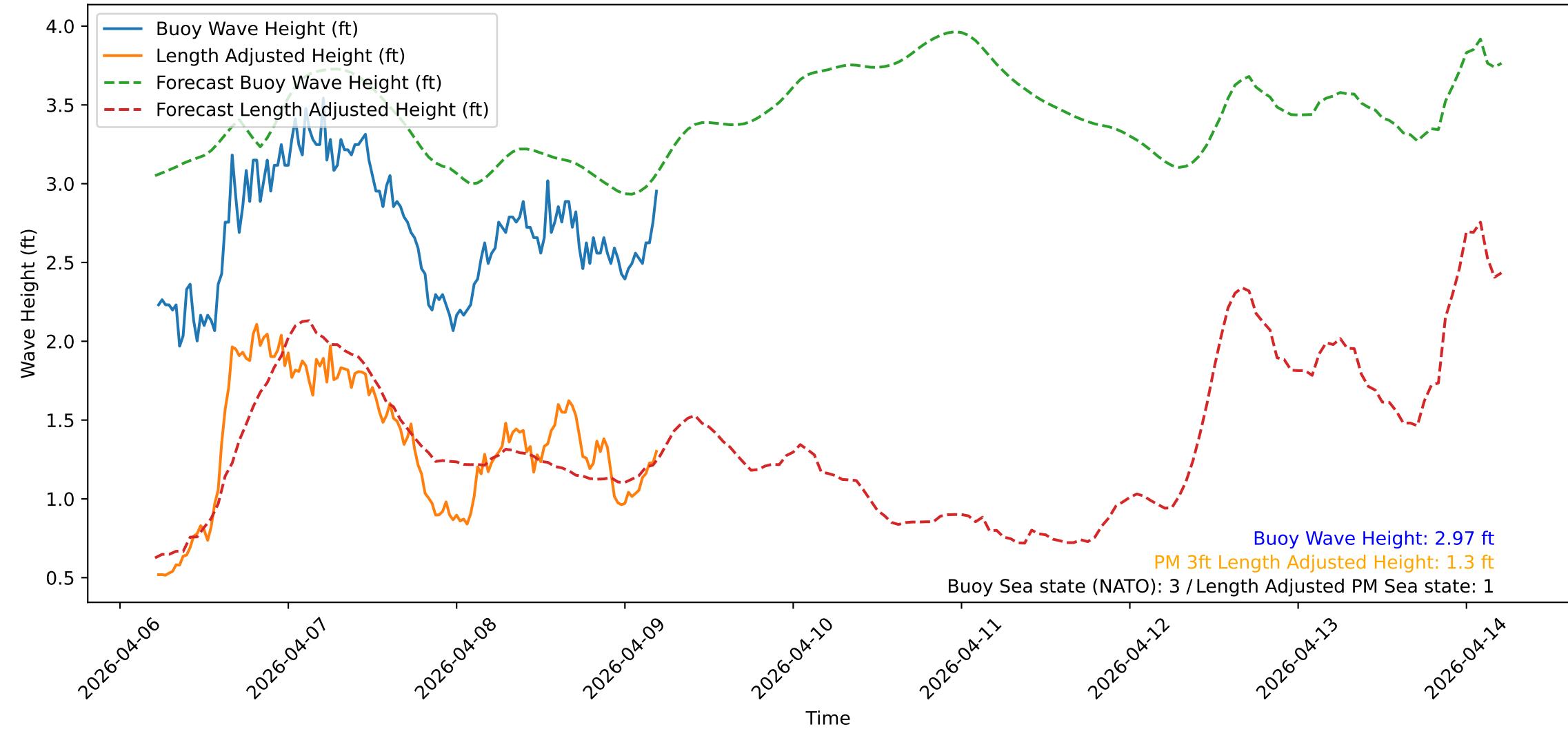
Wave Heights over Time for Red Beach at 2026-04-09 05:10:46
