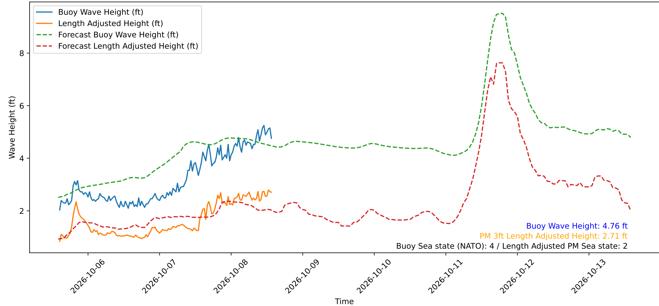
Wave Heights over Time for Green Beach at 2026-10-08 14:11:12
