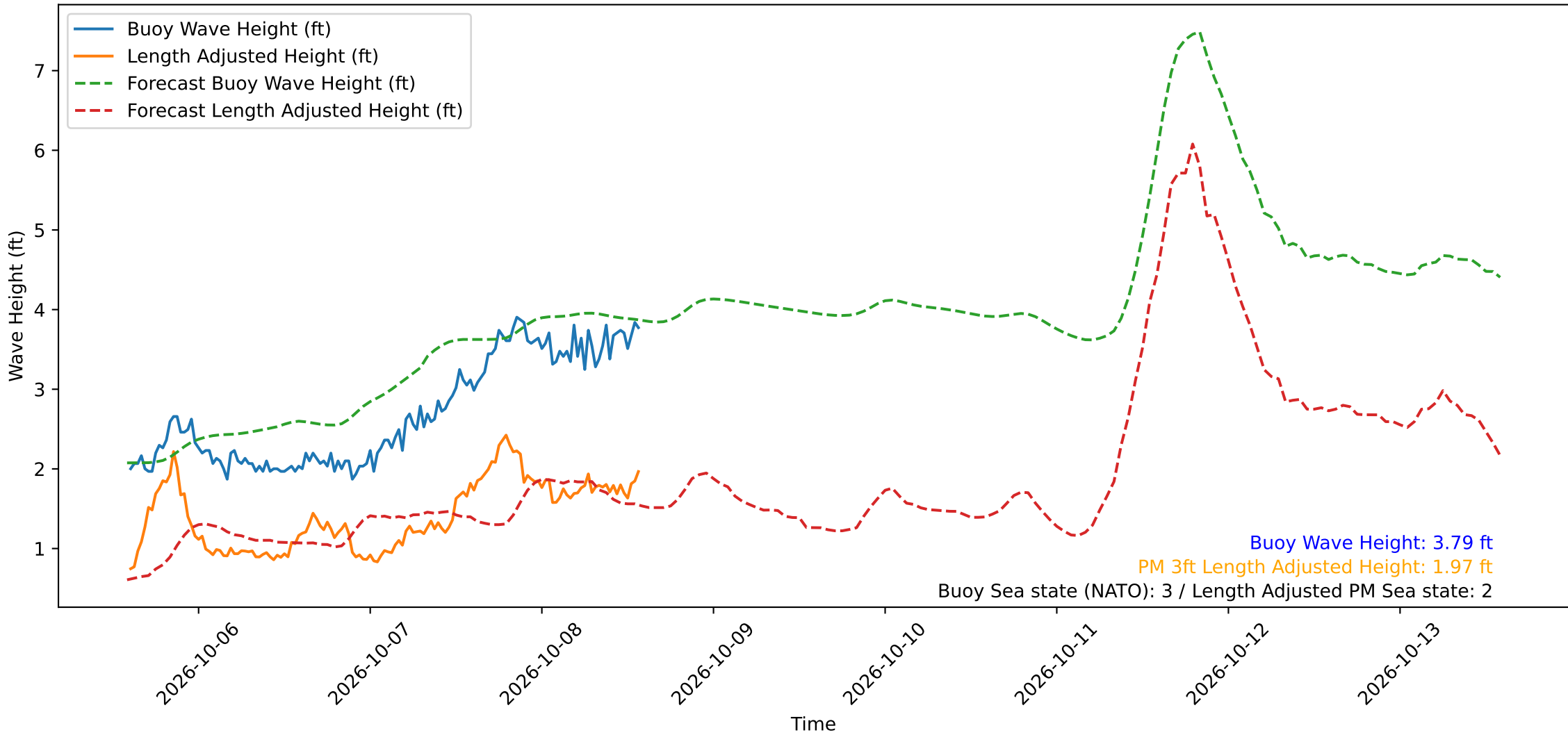
Wave Heights over Time for Red Beach at 2026-10-08 14:10:50
