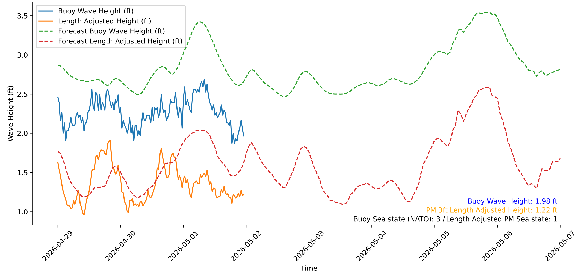
Wave Heights over Time for Oceanside Harbor at 2026-05-02 00:00:31
