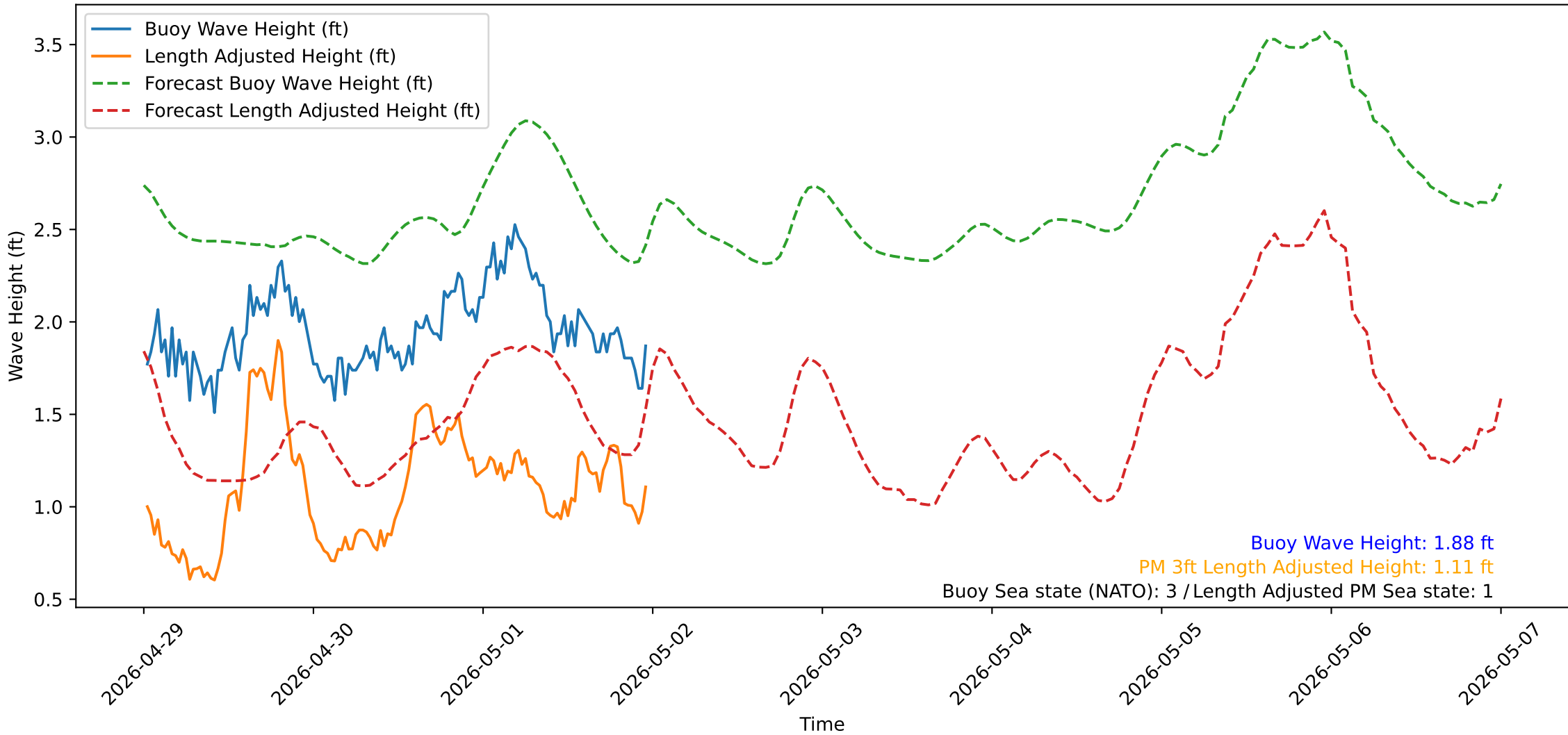
Wave Heights over Time for Red Beach at 2026-05-02 00:00:50
