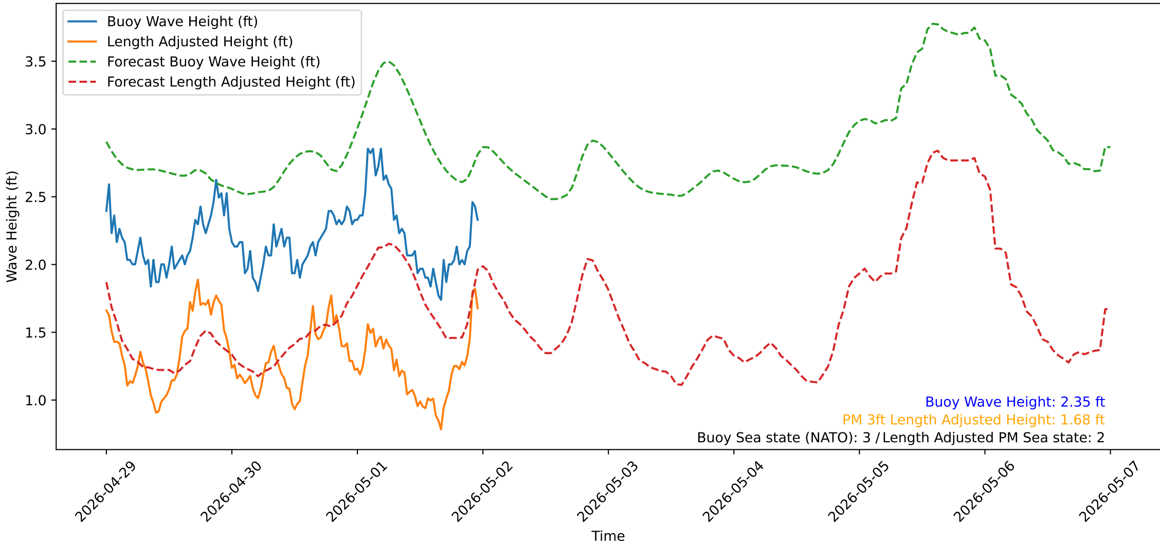
Wave Heights over Time for Green Beach at 2026-05-02 00:01:12
