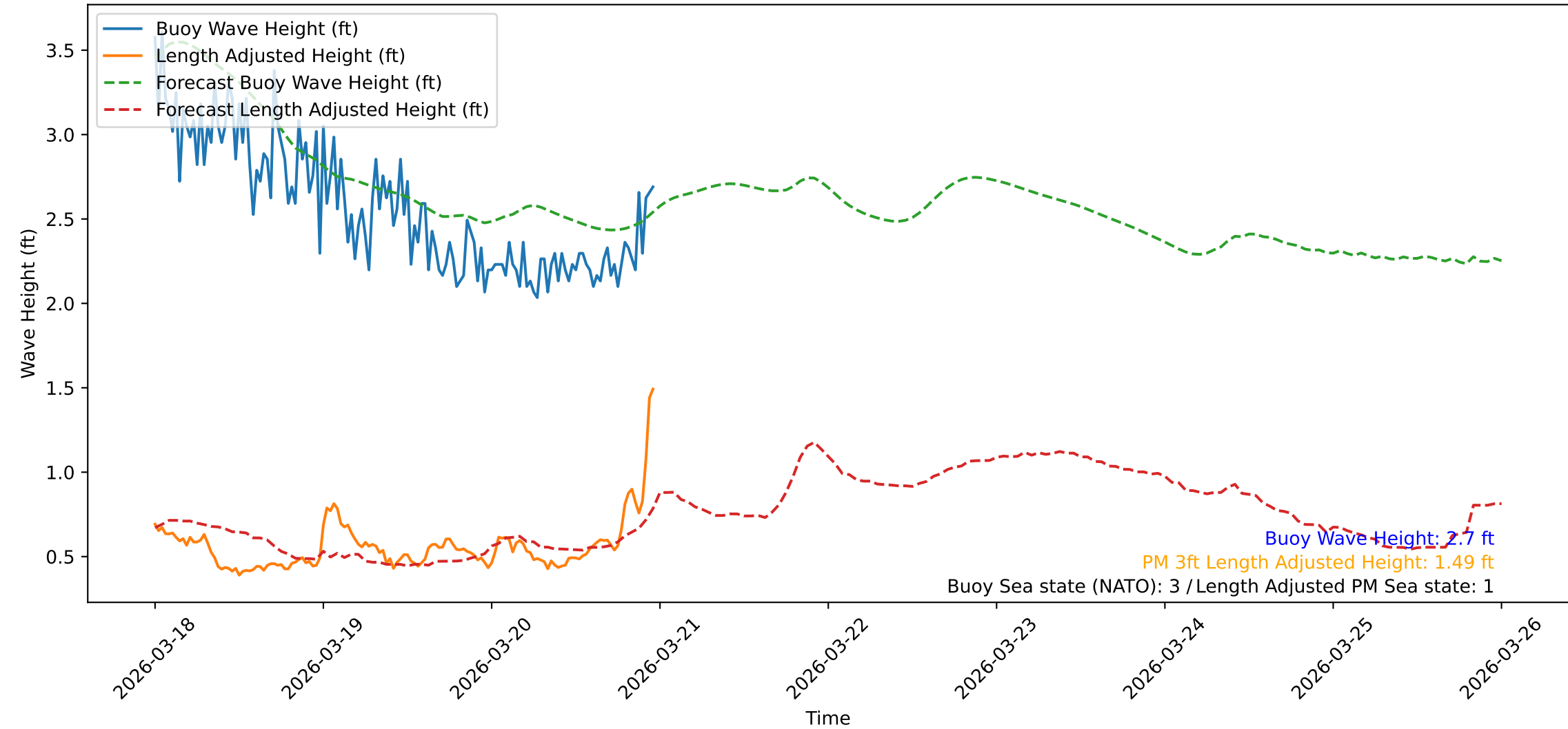
Wave Heights over Time for Green Beach at 2026-03-21 00:01:11
