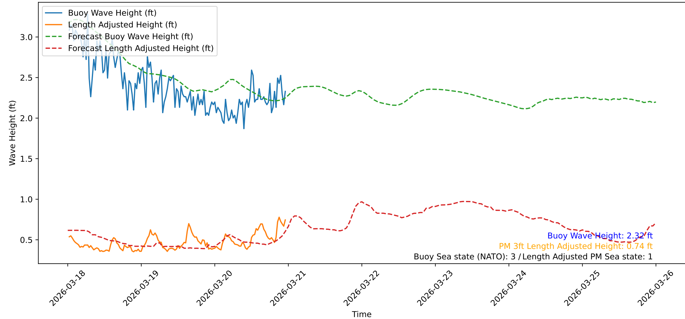
Wave Heights over Time for Red Beach at 2026-03-21 00:00:48
