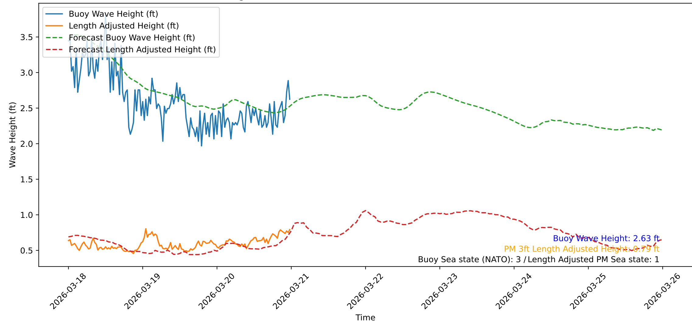
Wave Heights over Time for Oceanside Harbor at 2026-03-21 00:00:32
