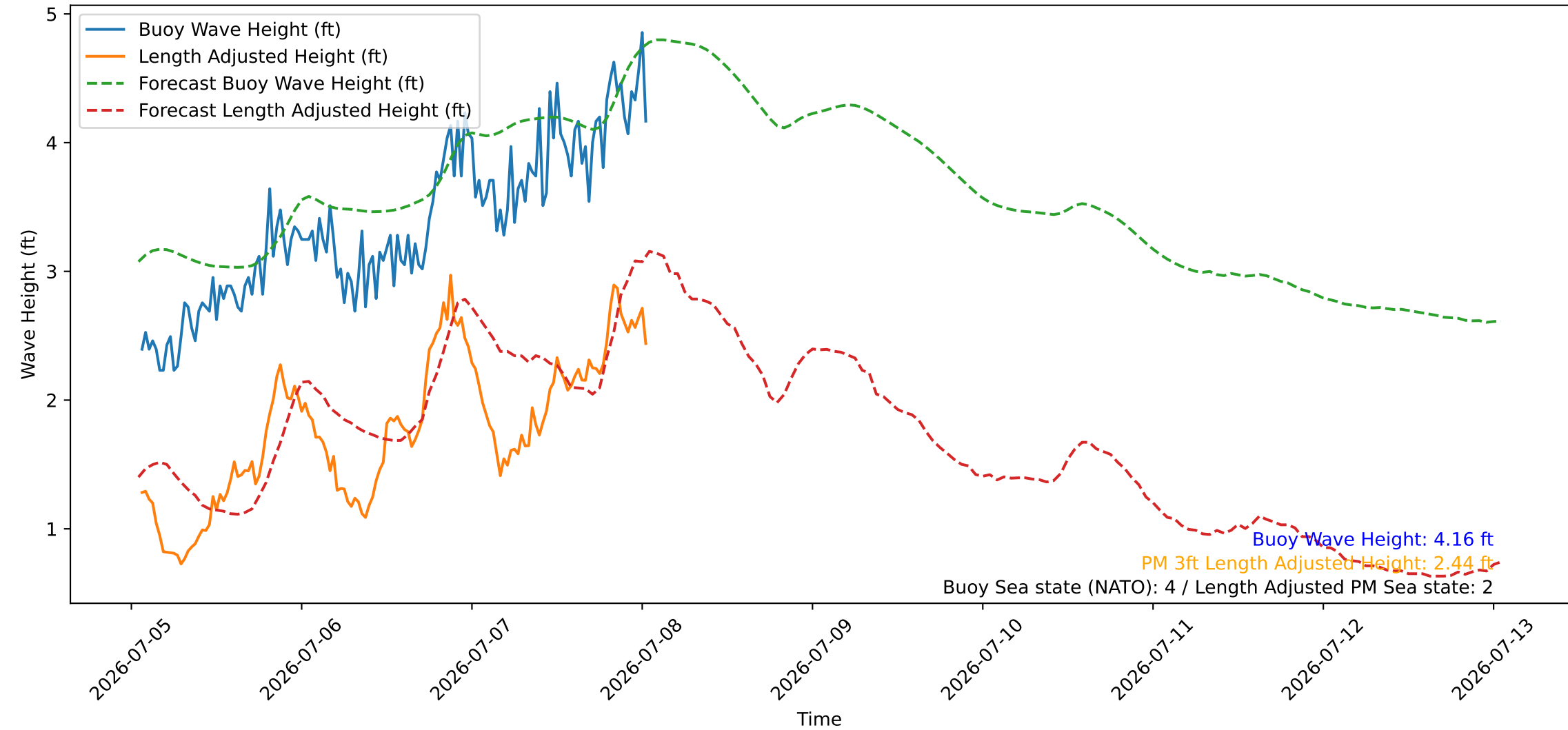
Wave Heights over Time for Red Beach at 2026-07-08 01:10:46
