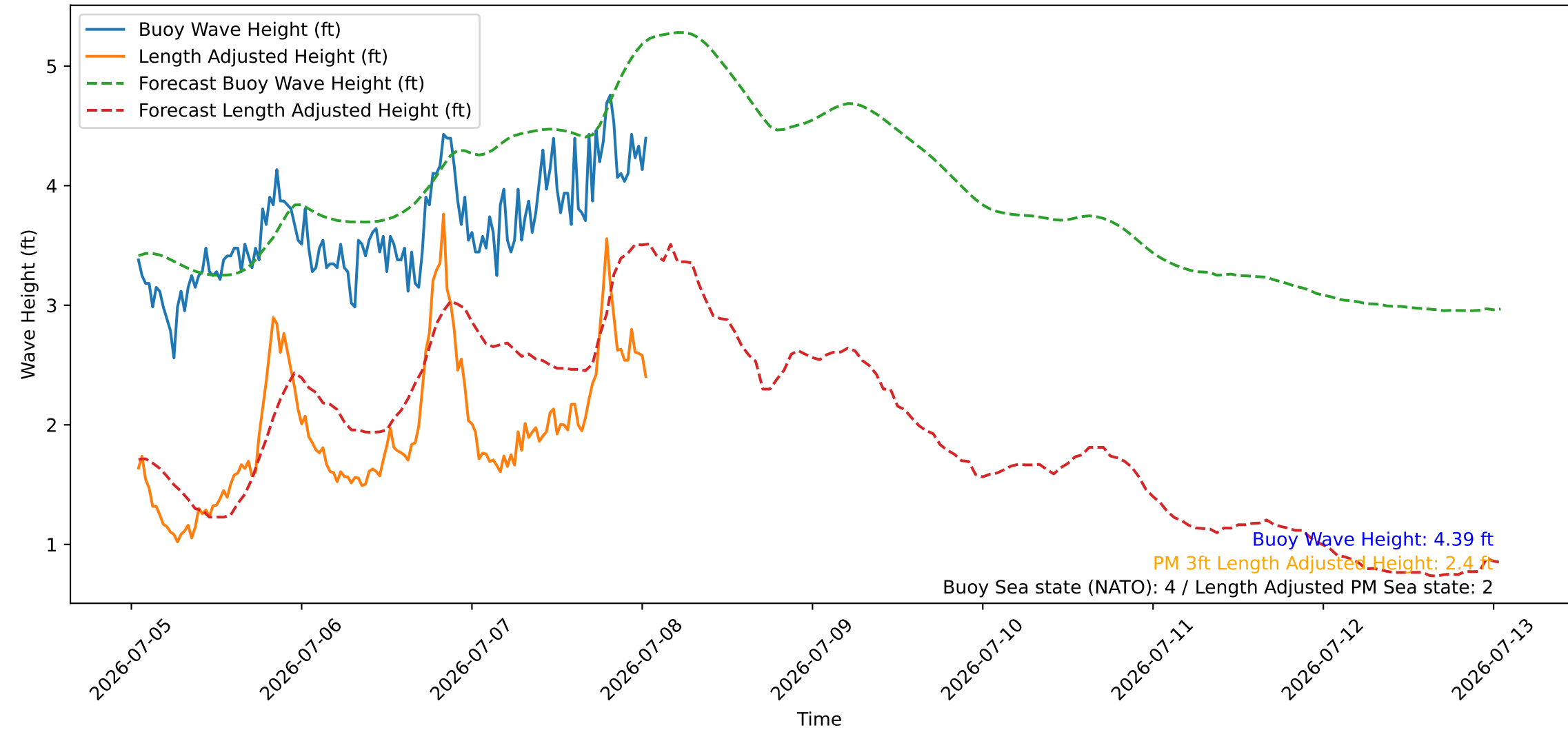
Wave Heights over Time for Green Beach at 2026-07-08 01:11:08
