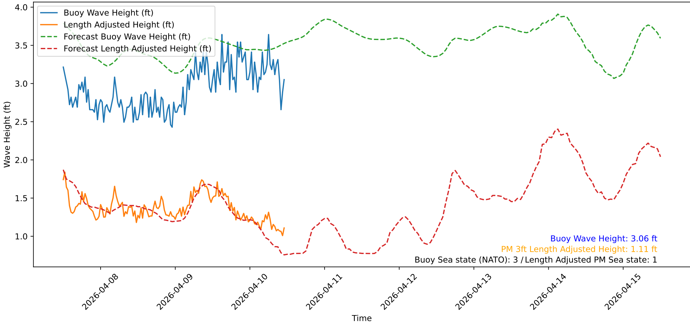
Wave Heights over Time for Oceanside Harbor at 2026-04-10 12:00:32
