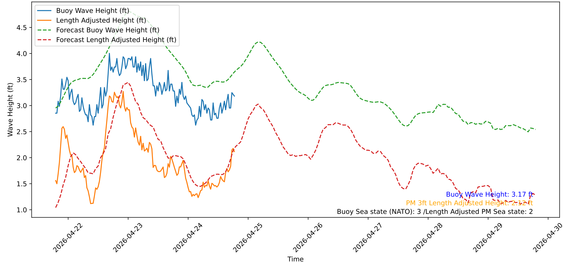
Wave Heights over Time for Green Beach at 2026-04-24 19:11:12
