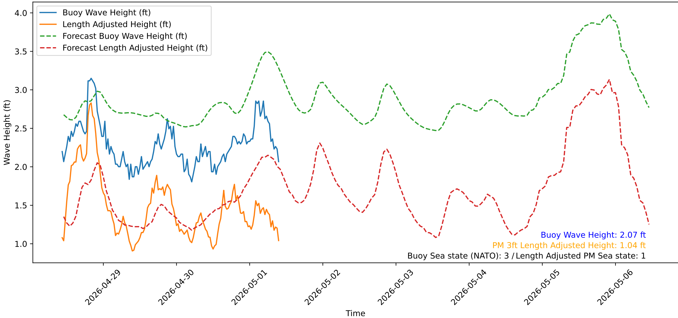
Wave Heights over Time for Green Beach at 2026-05-01 10:41:14
