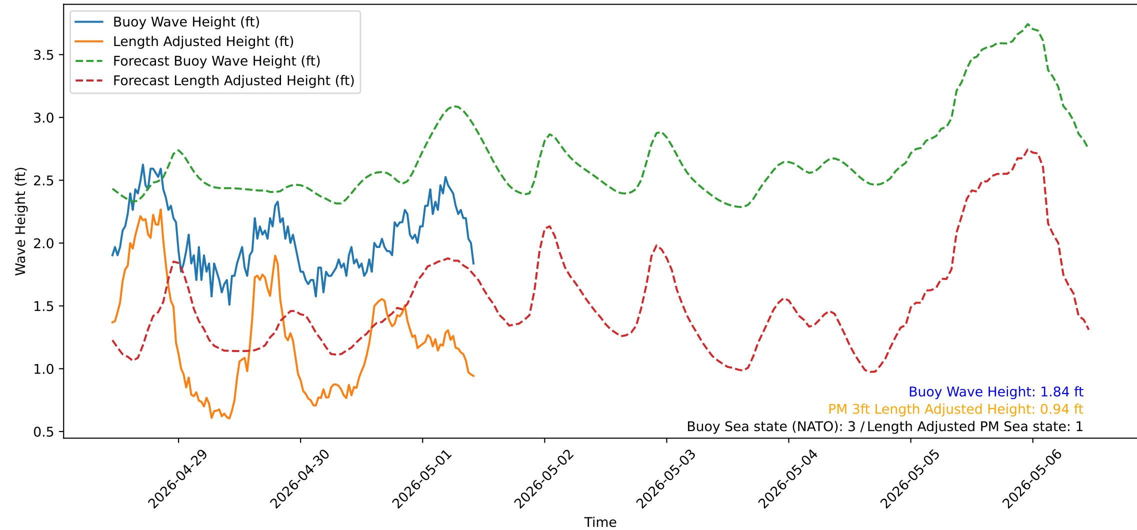
Wave Heights over Time for Red Beach at 2026-05-01 10:40:51
