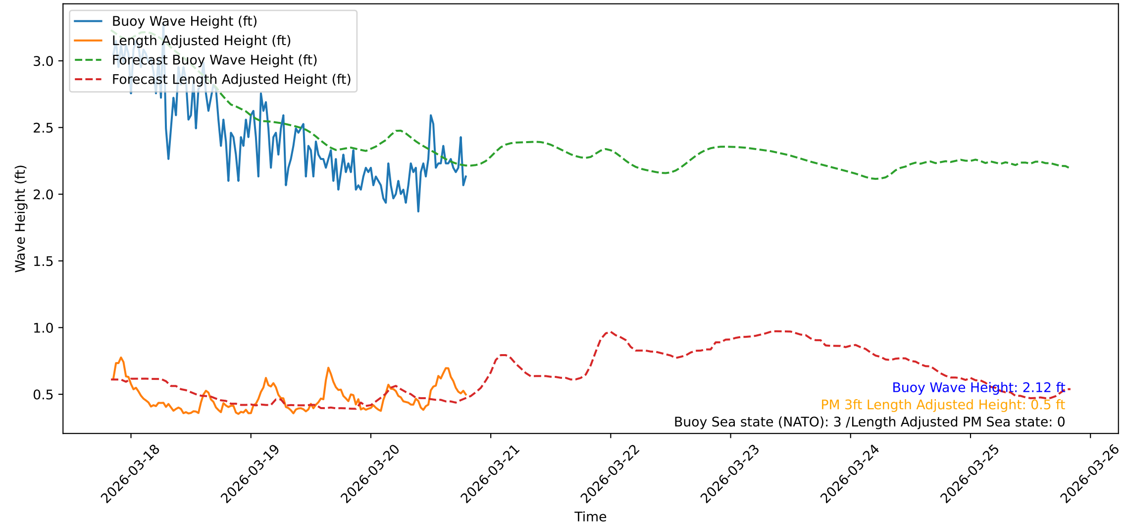
Wave Heights over Time for Red Beach at 2026-03-20 20:00:48
