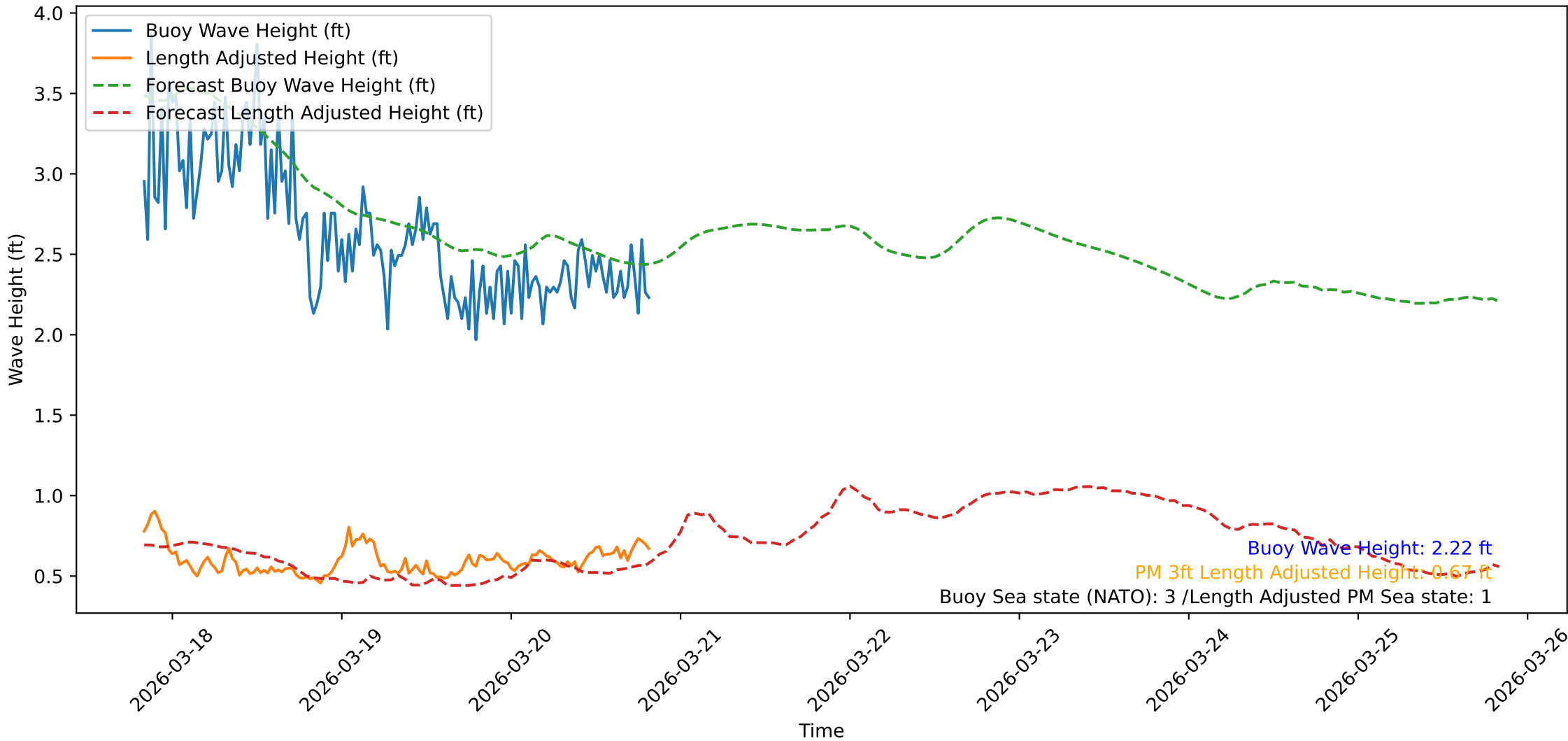
Wave Heights over Time for Oceanside Harbor at 2026-03-20 20:00:32
