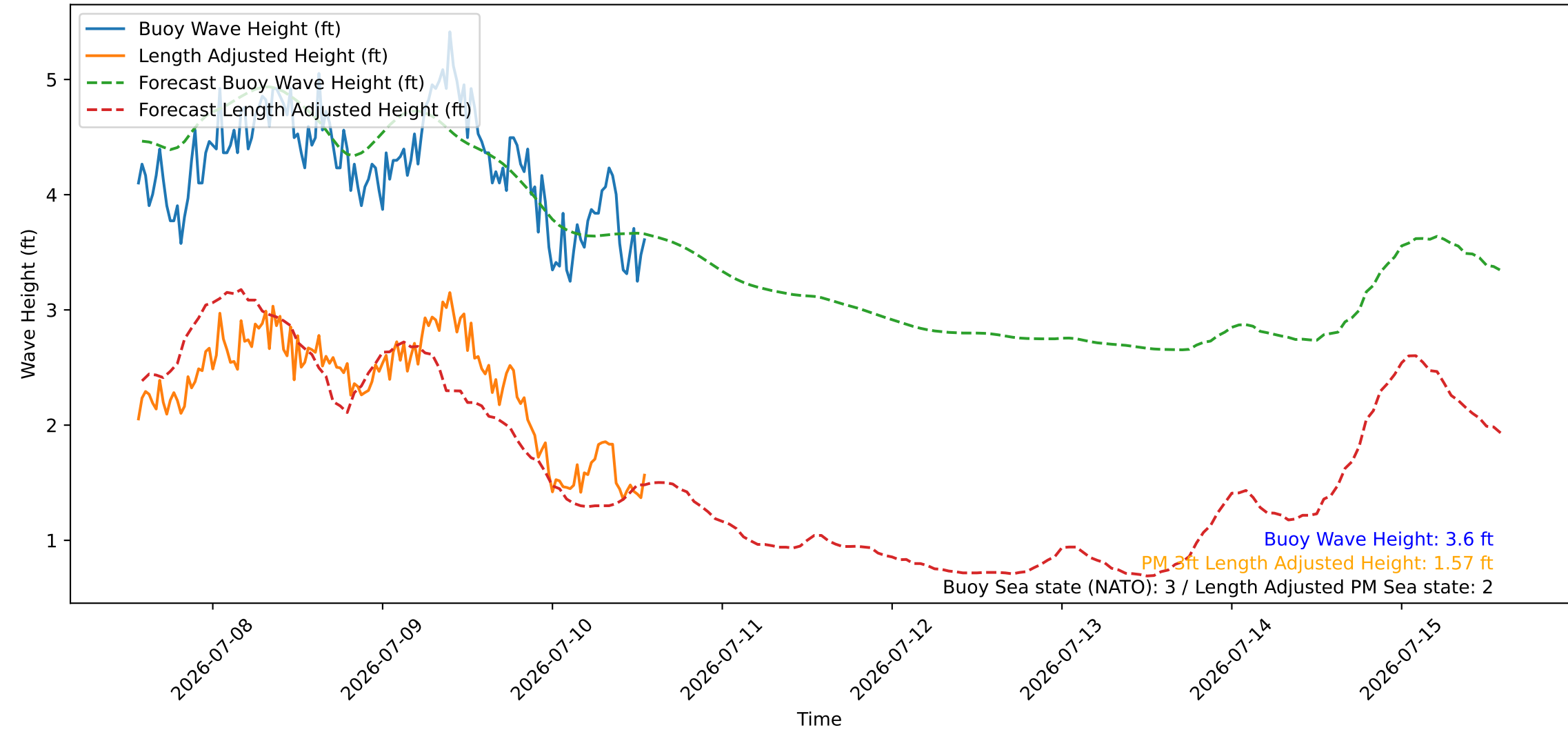
Wave Heights over Time for Oceanside Harbor at 2026-07-10 13:40:26
