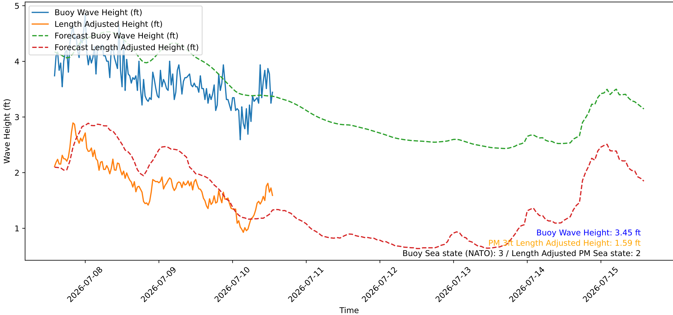
Wave Heights over Time for Red Beach at 2026-07-10 13:40:45
