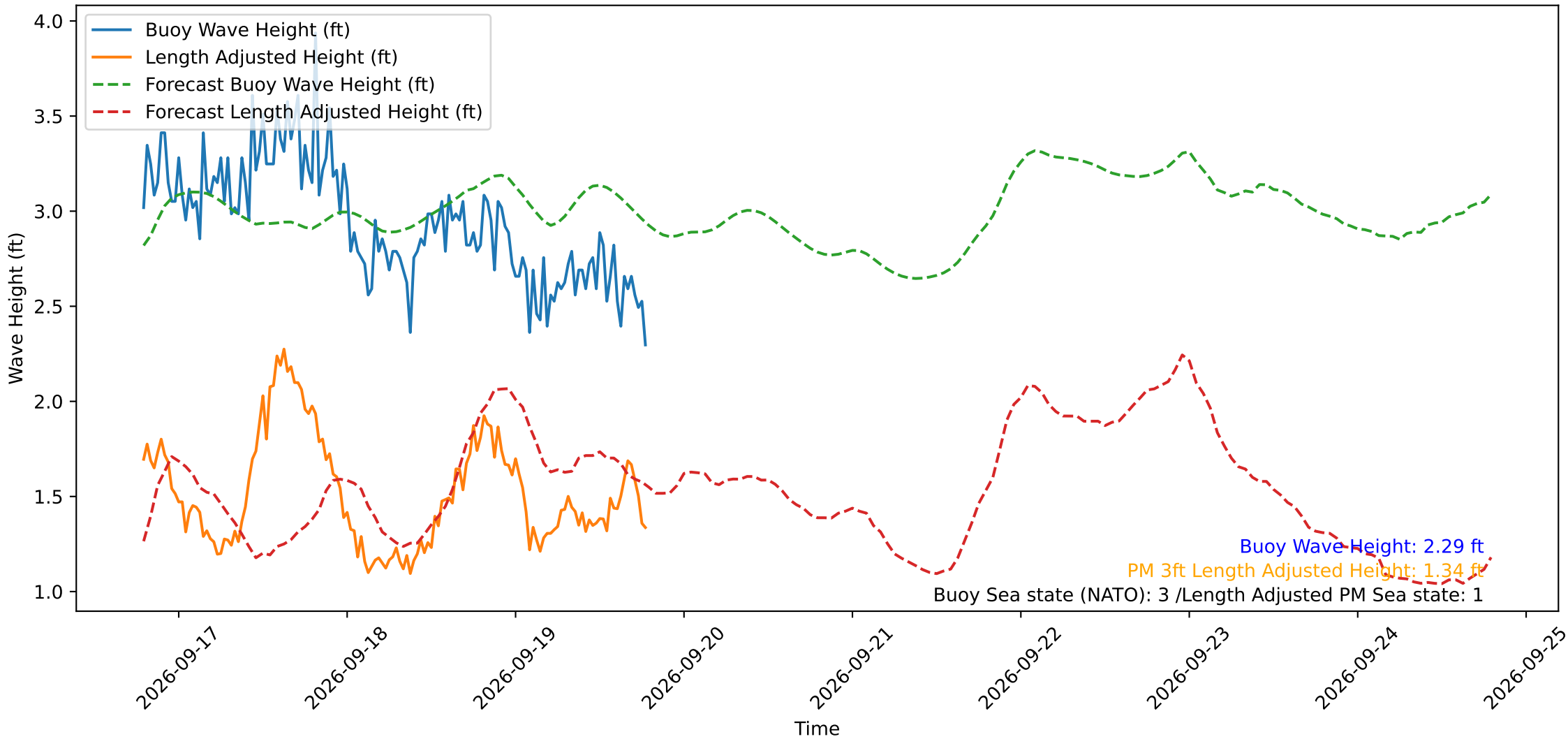
Wave Heights over Time for Oceanside Harbor at 2026-09-19 19:10:29
