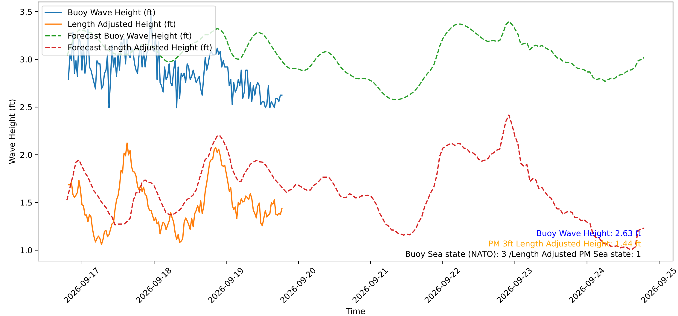
Wave Heights over Time for Green Beach at 2026-09-19 19:11:11
