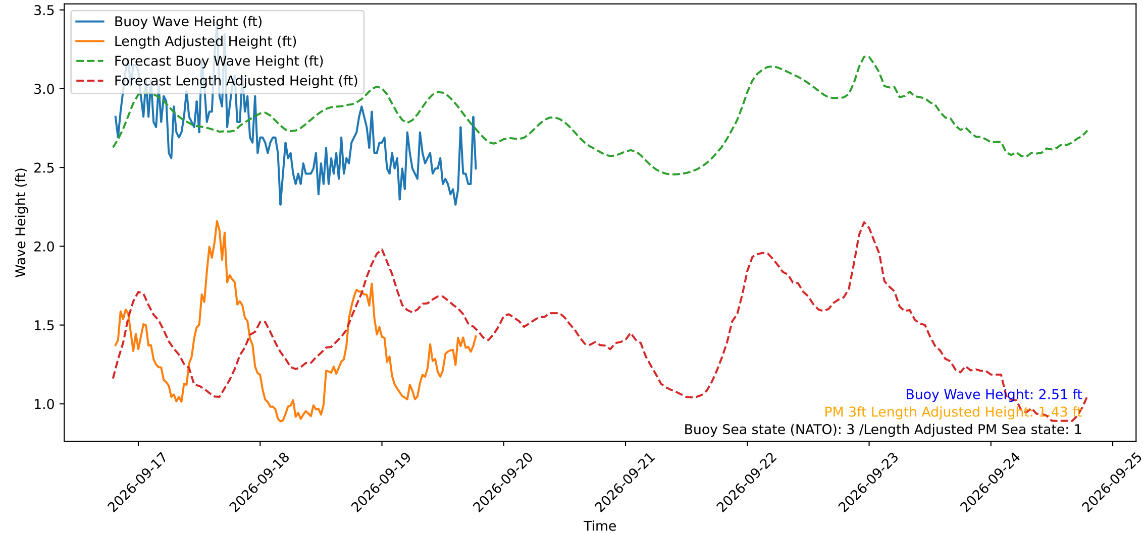
Wave Heights over Time for Red Beach at 2026-09-19 19:10:49
