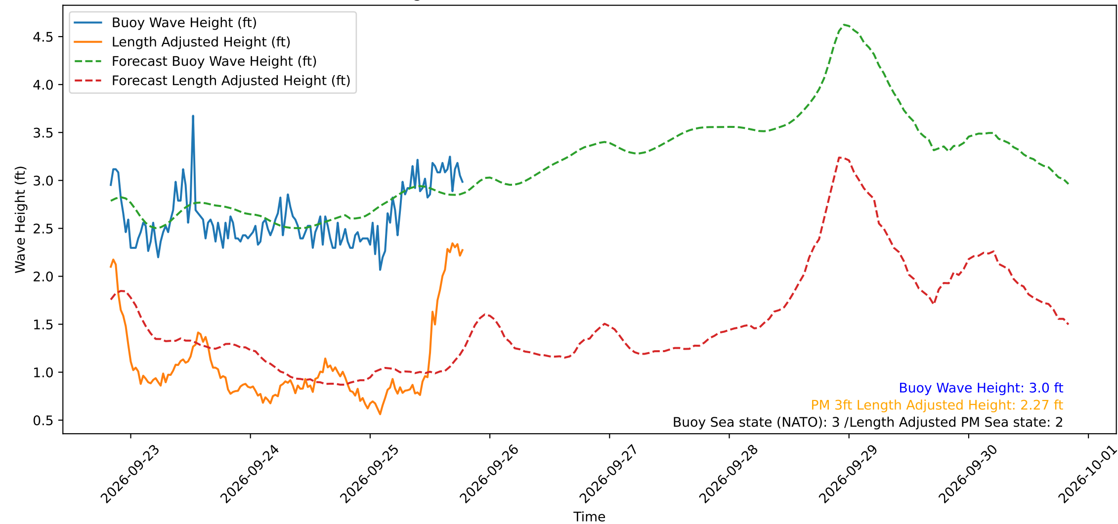
Wave Heights over Time for Red Beach at 2026-09-25 19:30:49
