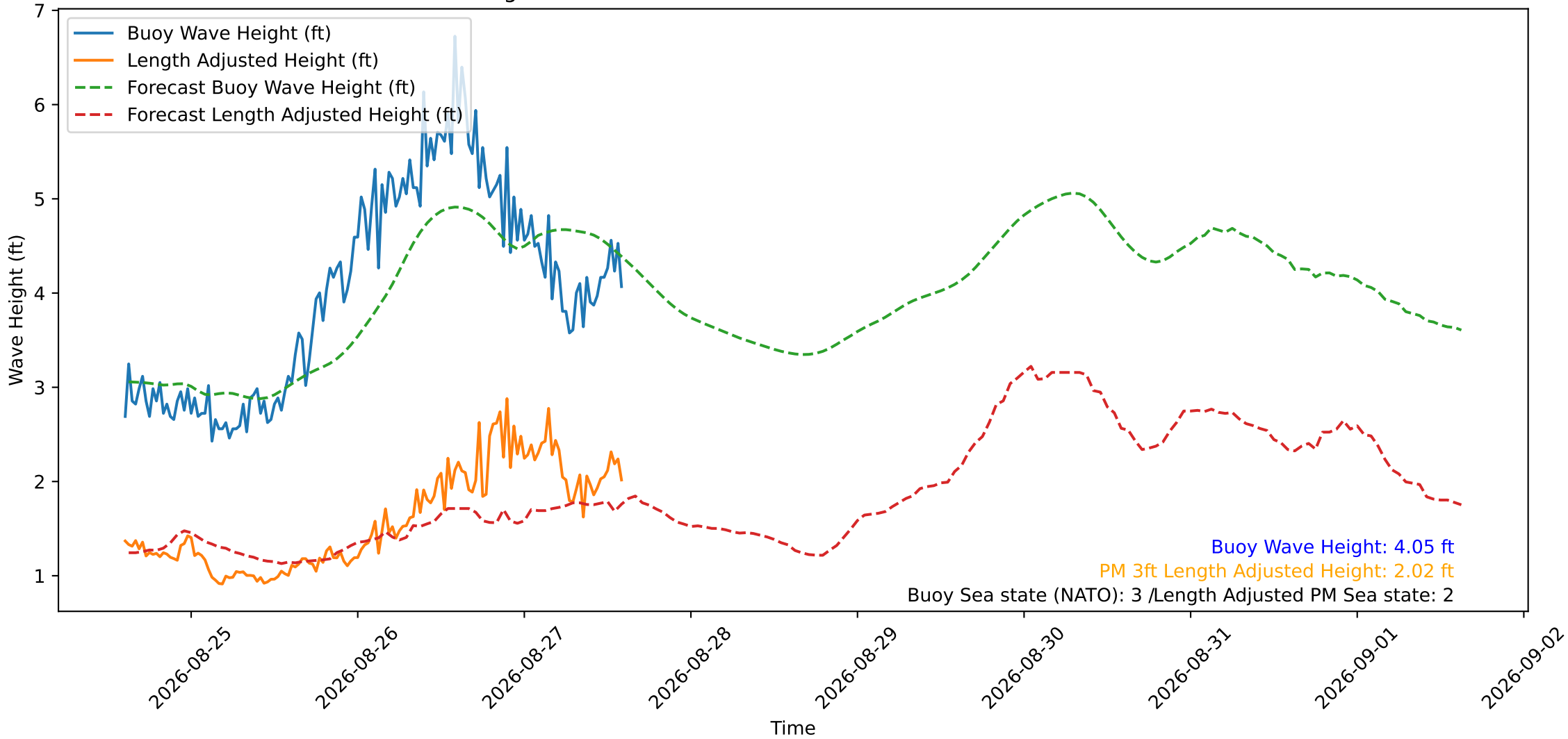
Wave Heights over Time for Oceanside Harbor at 2026-08-27 14:40:29
