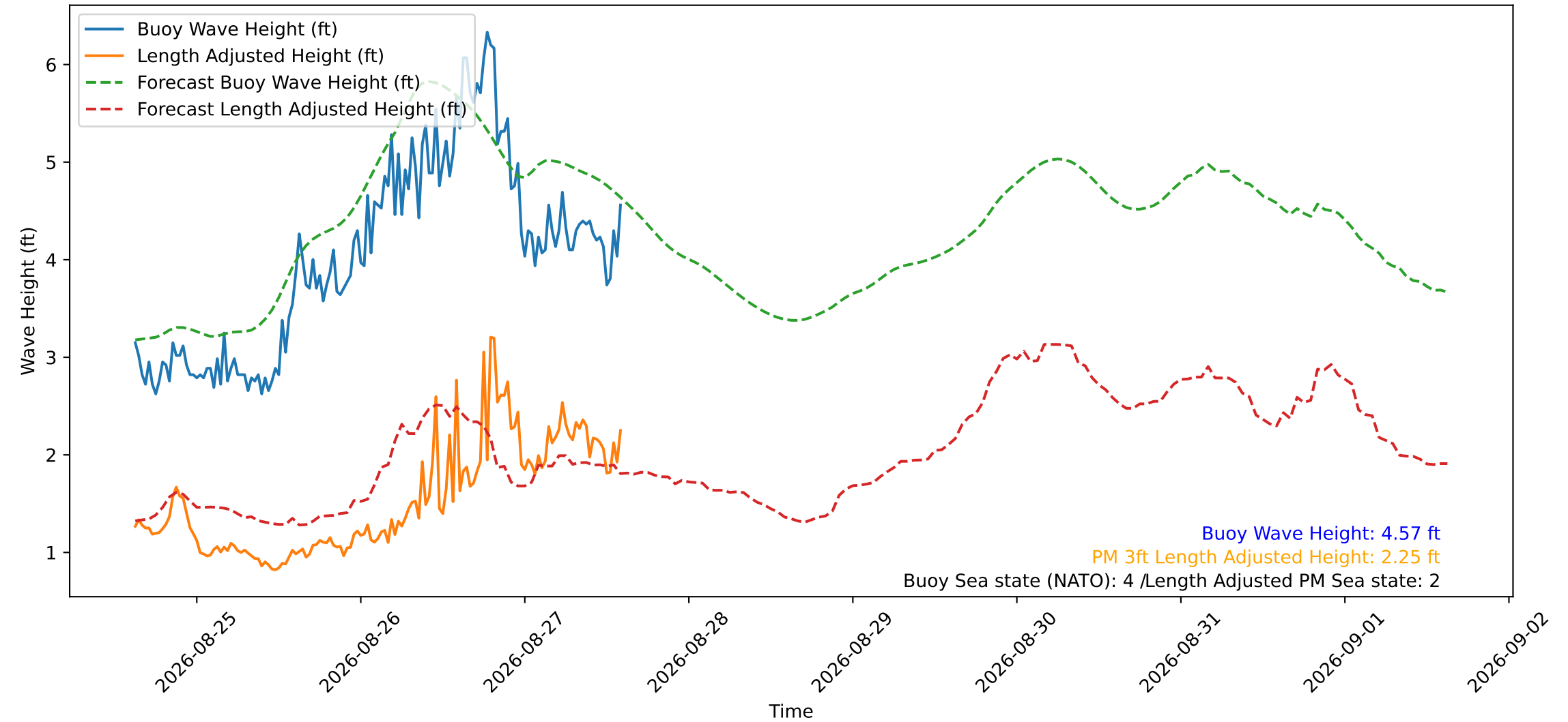
Wave Heights over Time for Green Beach at 2026-08-27 14:41:12
