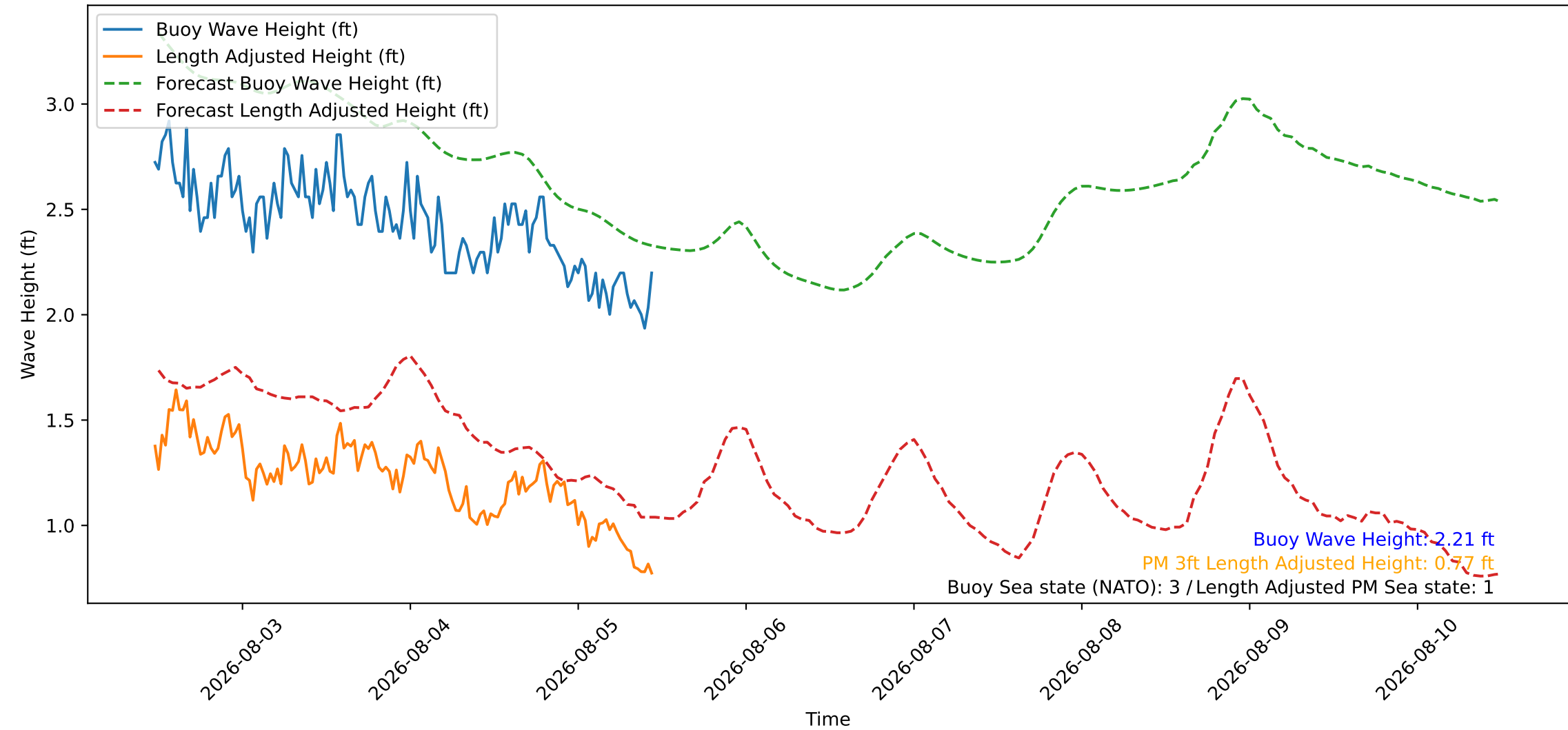
Wave Heights over Time for Oceanside Harbor at 2026-08-05 11:30:26
