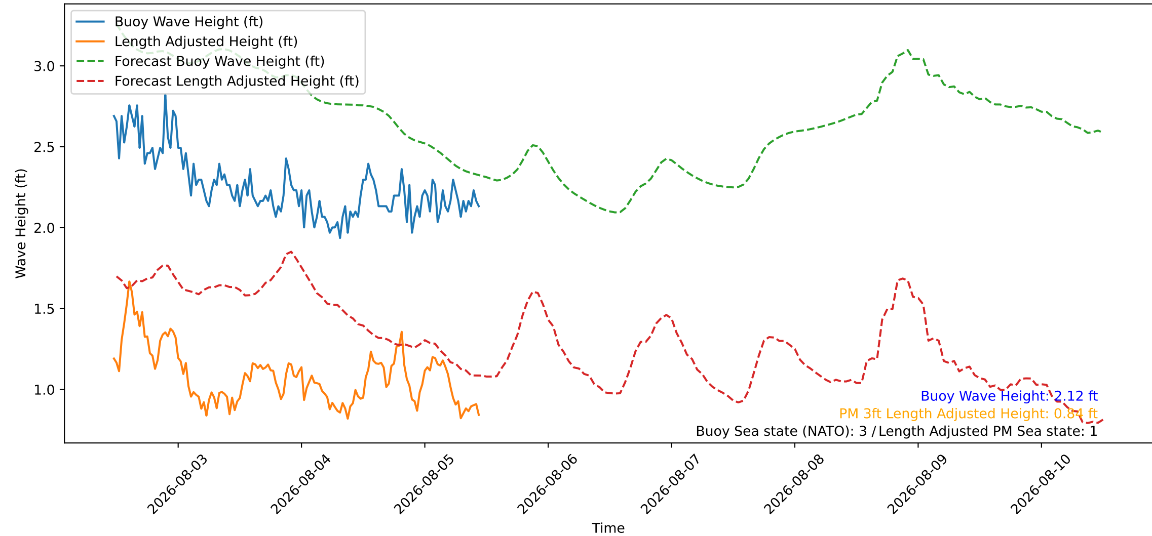
Wave Heights over Time for Green Beach at 2026-08-05 11:31:08
