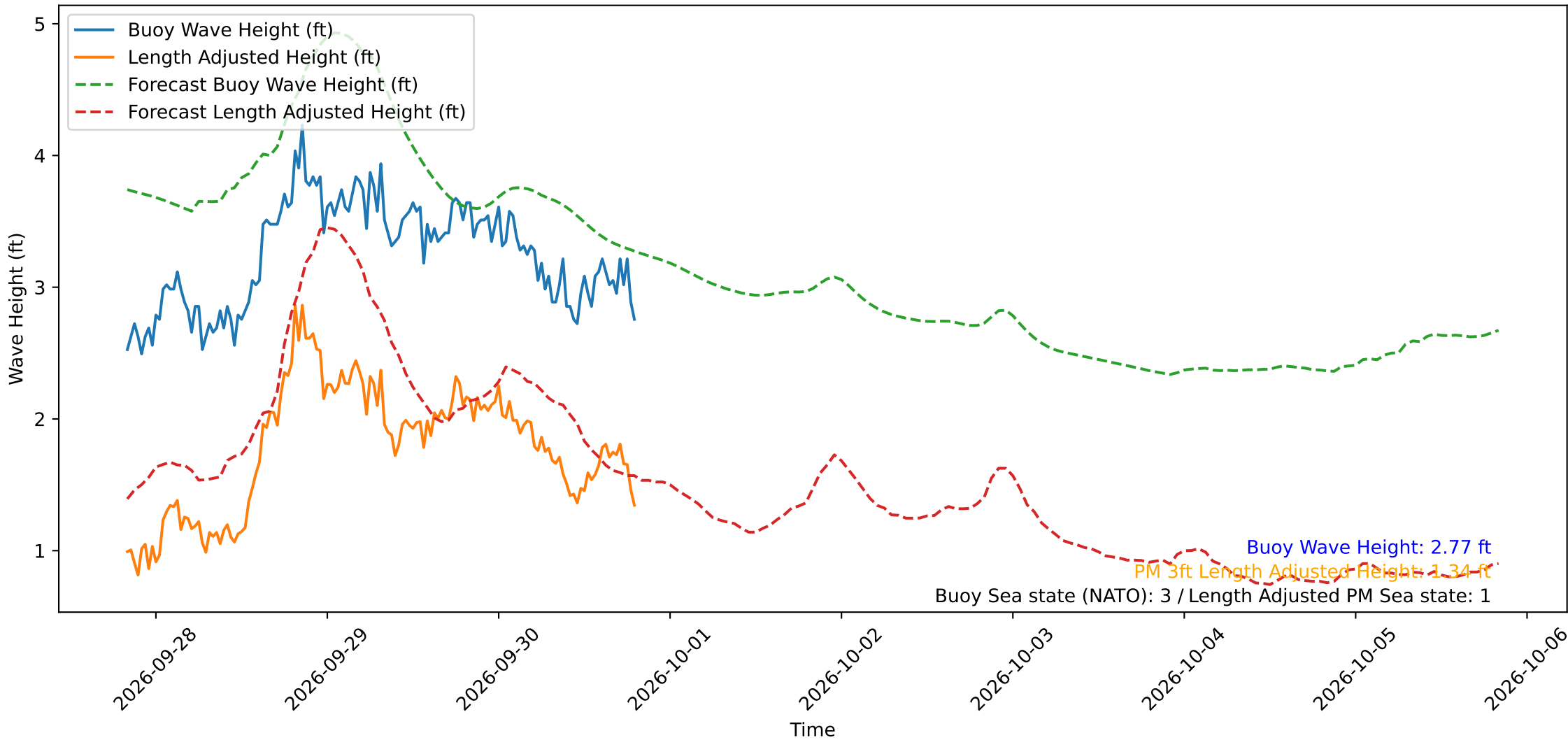
Wave Heights over Time for Oceanside Harbor at 2026-09-30 20:00:30
