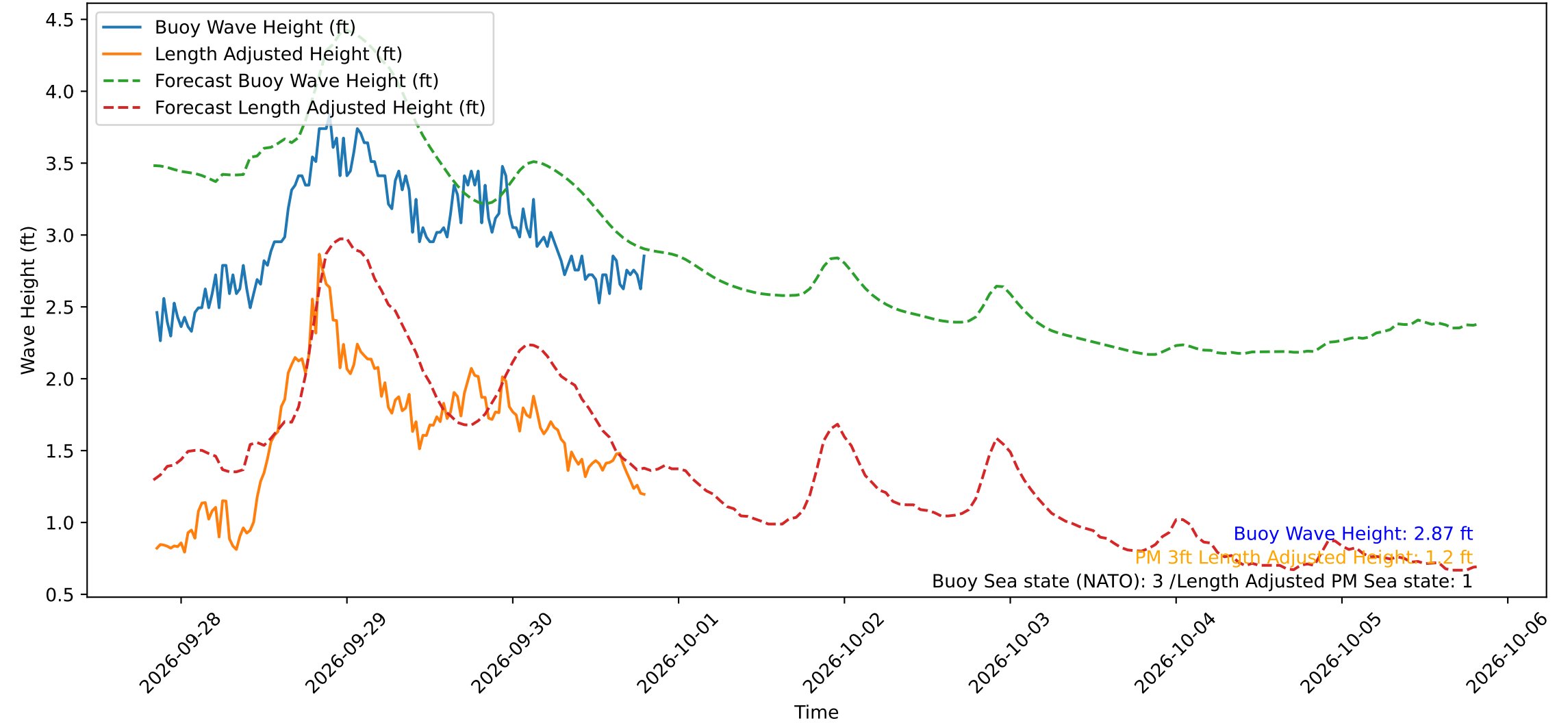
Wave Heights over Time for Red Beach at 2026-09-30 20:00:50
