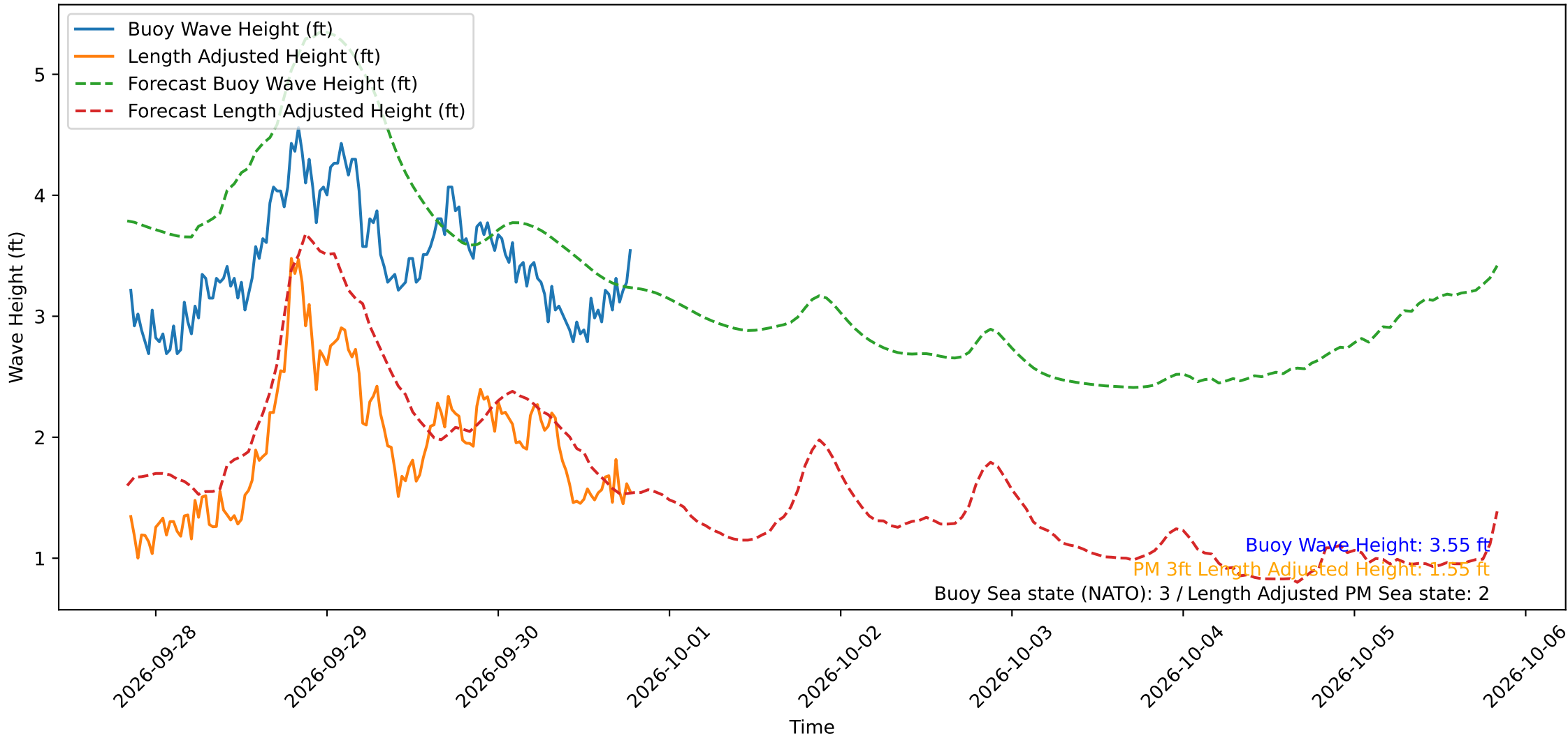
Wave Heights over Time for Green Beach at 2026-09-30 20:01:13
