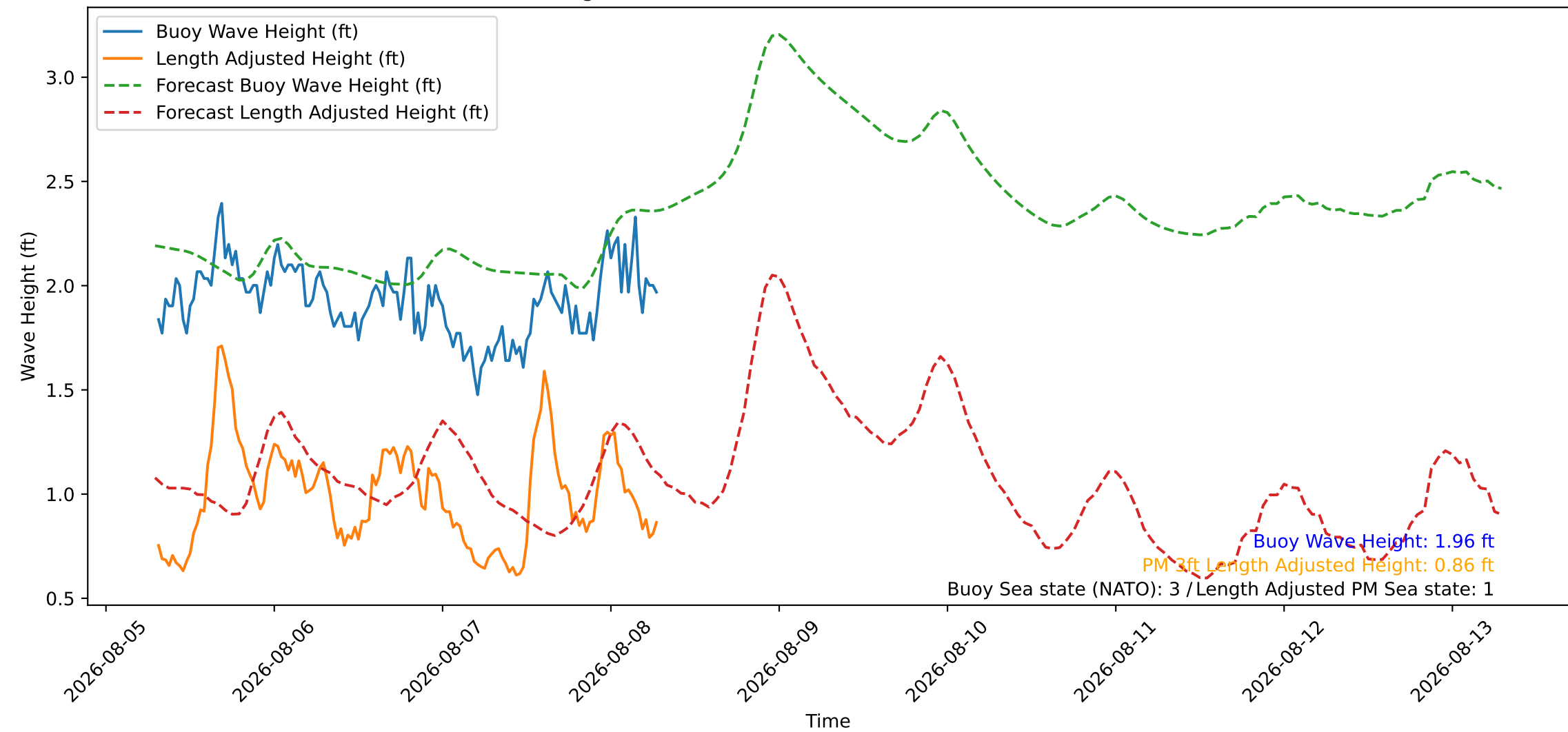
Wave Heights over Time for Red Beach at 2026-08-08 07:10:46
