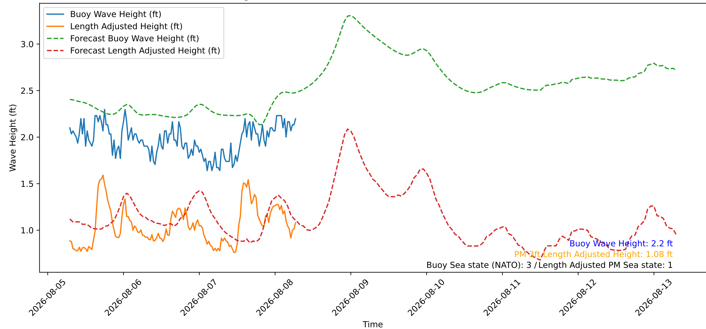
Wave Heights over Time for Oceanside Harbor at 2026-08-08 07:10:26
