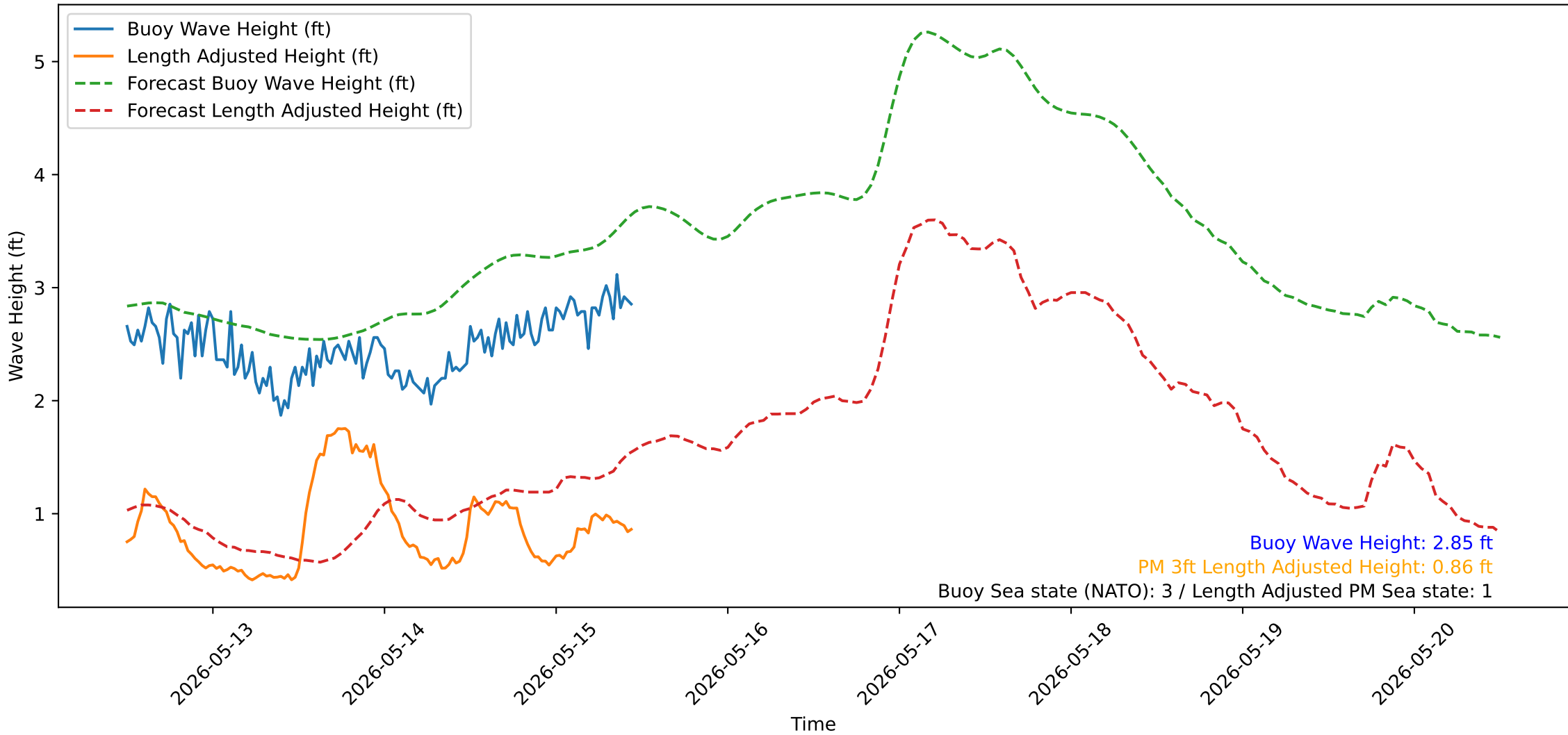
Wave Heights over Time for Red Beach at 2026-05-15 11:30:51
