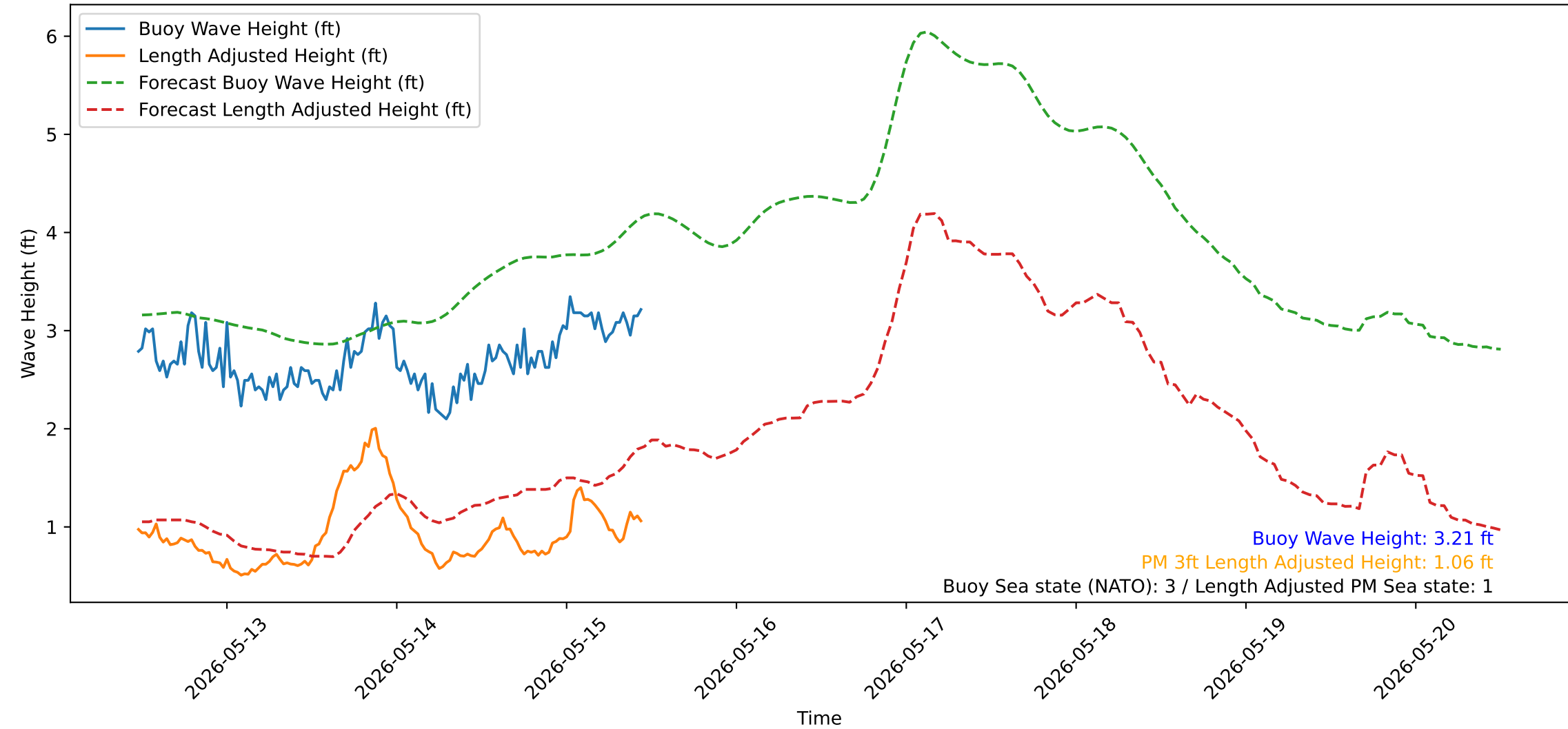
Wave Heights over Time for Green Beach at 2026-05-15 11:31:14
