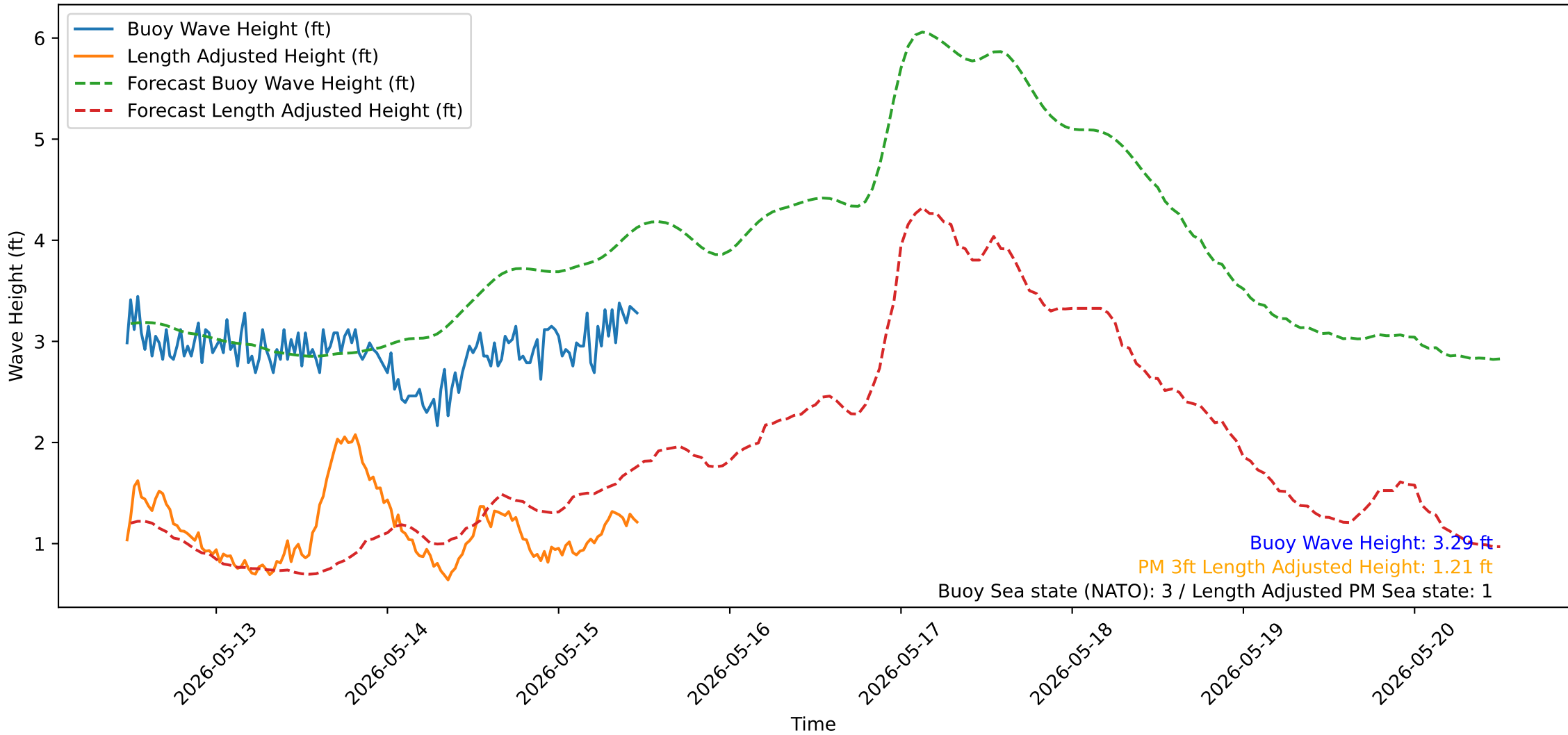
Wave Heights over Time for Oceanside Harbor at 2026-05-15 11:30:32
