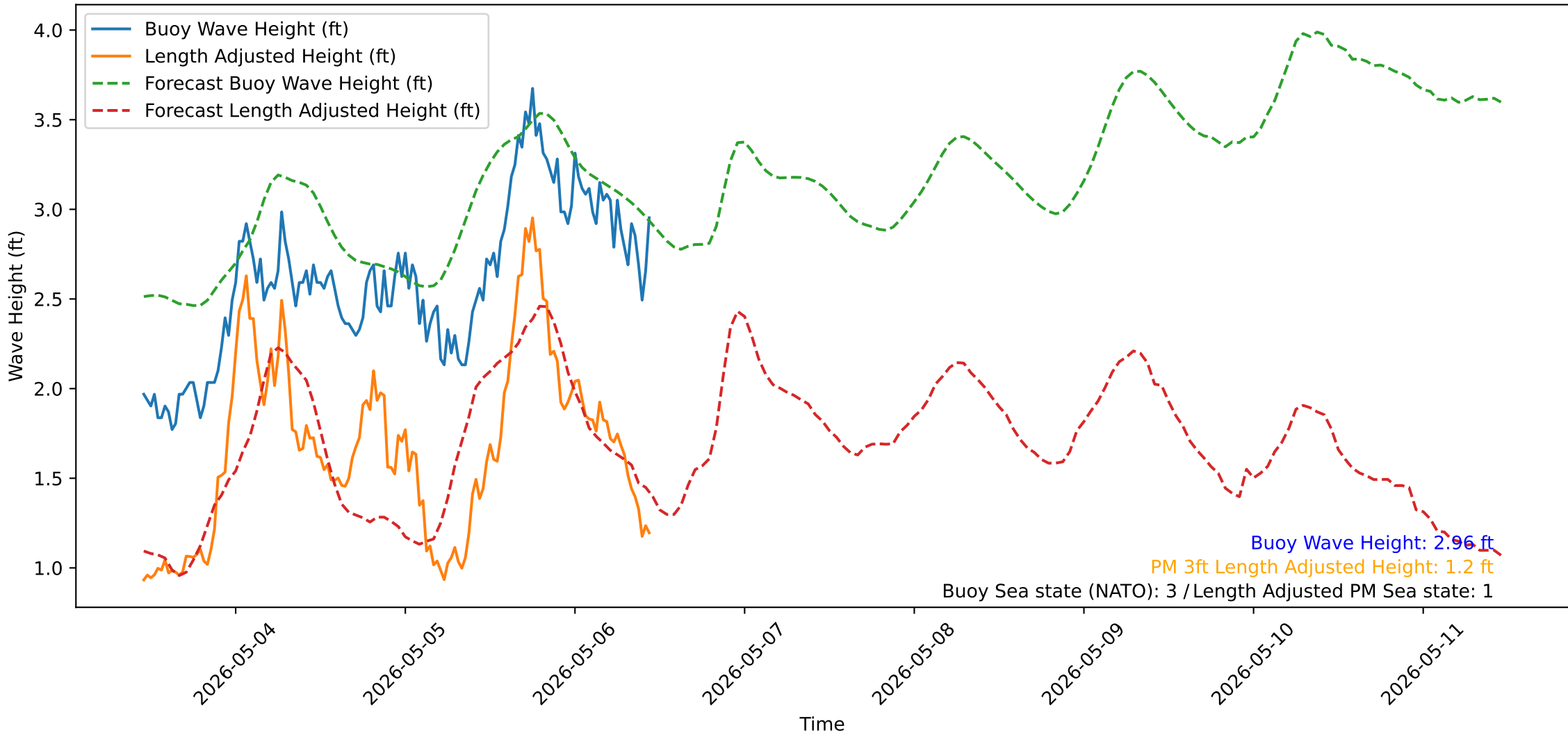
Wave Heights over Time for Green Beach at 2026-05-06 11:11:12
