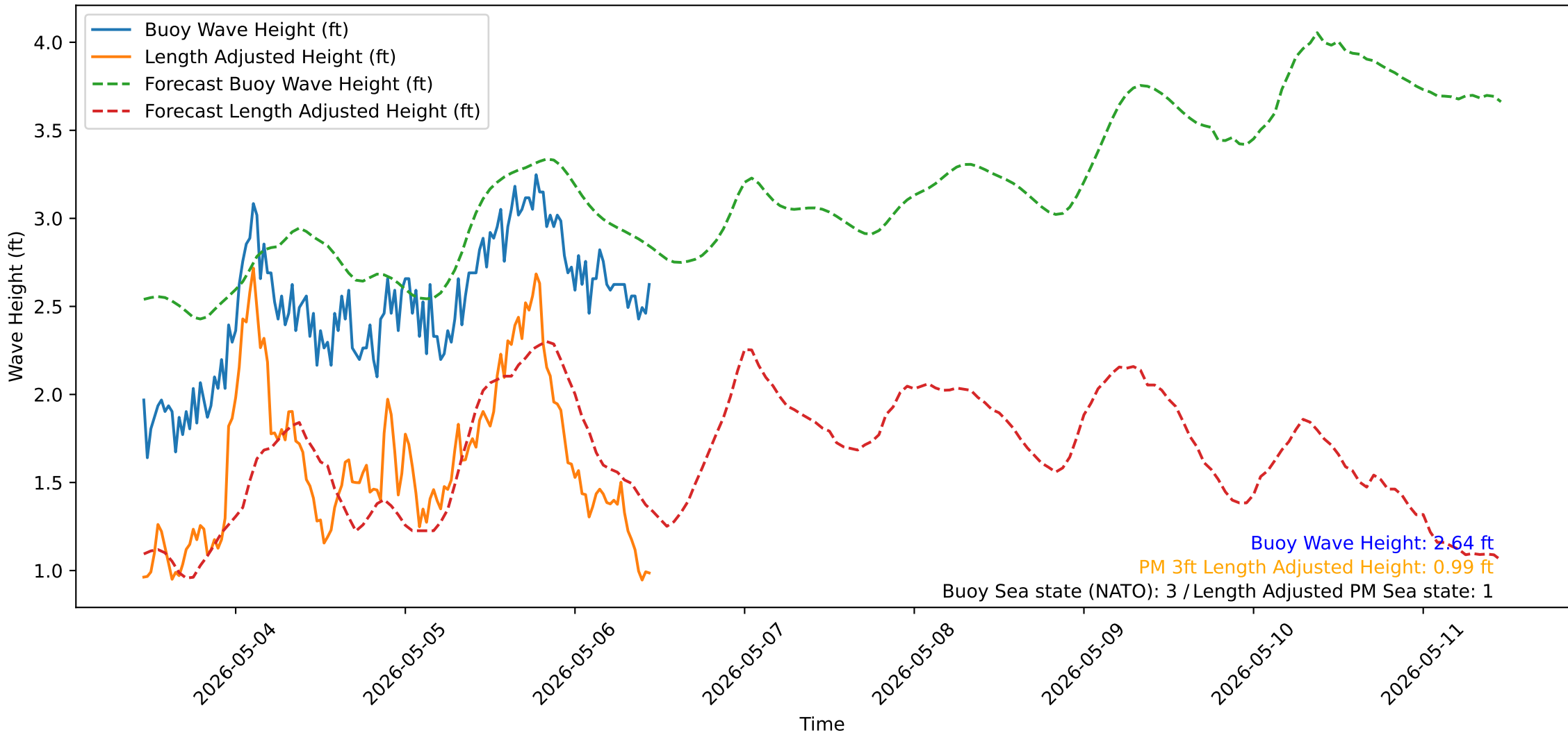
Wave Heights over Time for Oceanside Harbor at 2026-05-06 11:10:31
