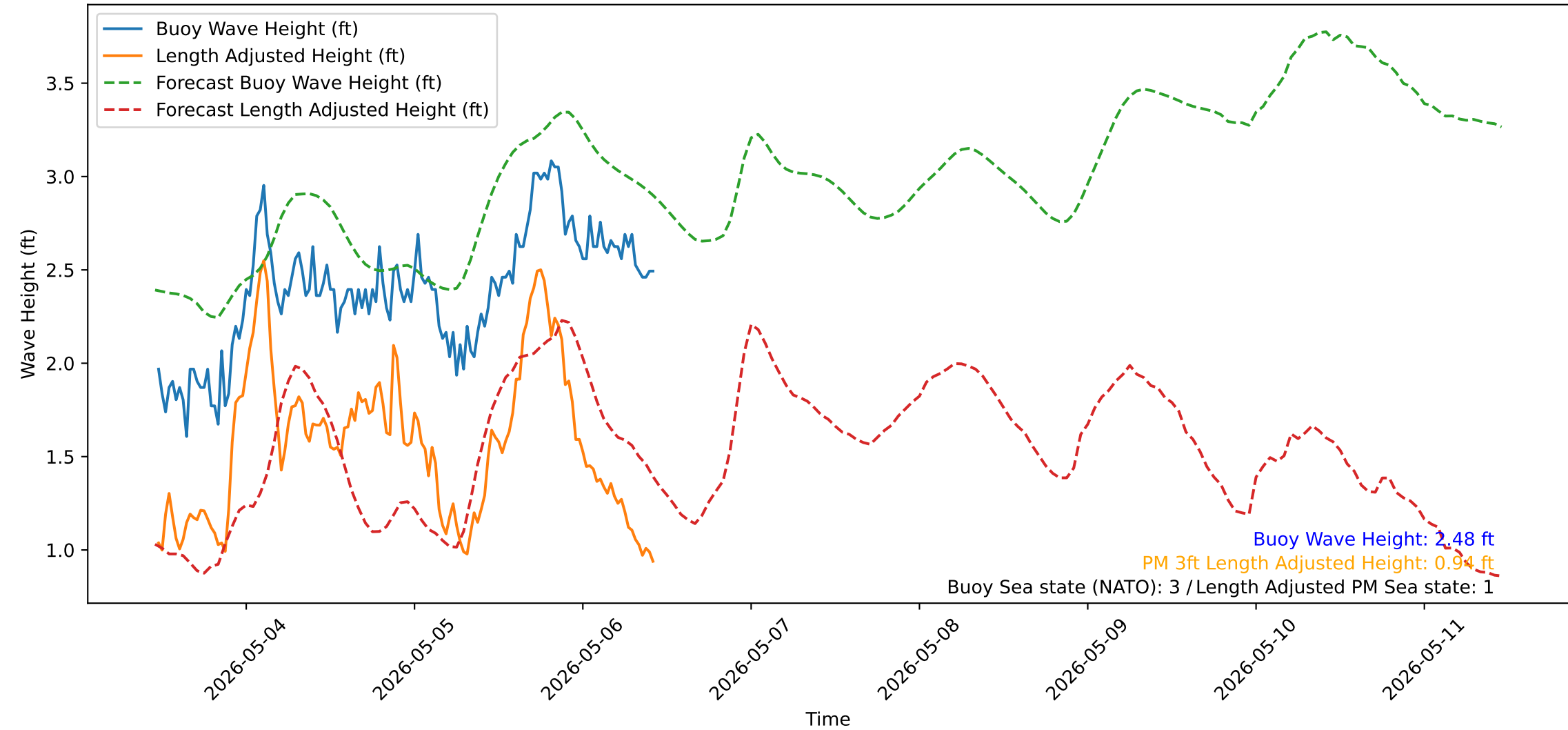
Wave Heights over Time for Red Beach at 2026-05-06 11:10:50
