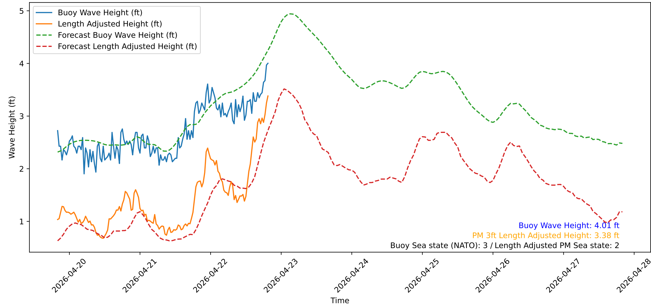
Wave Heights over Time for Oceanside Harbor at 2026-04-22 20:00:31
