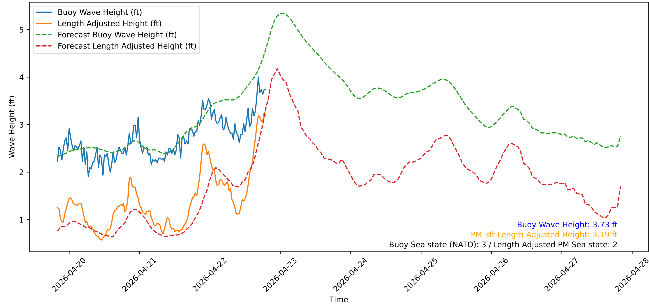
Wave Heights over Time for Green Beach at 2026-04-22 20:01:13
