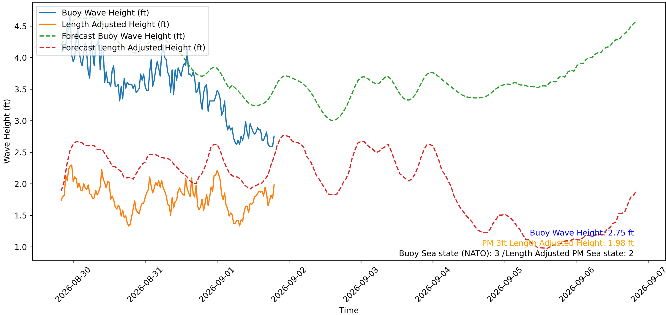
Wave Heights over Time for Red Beach at 2026-09-01 19:40:50
