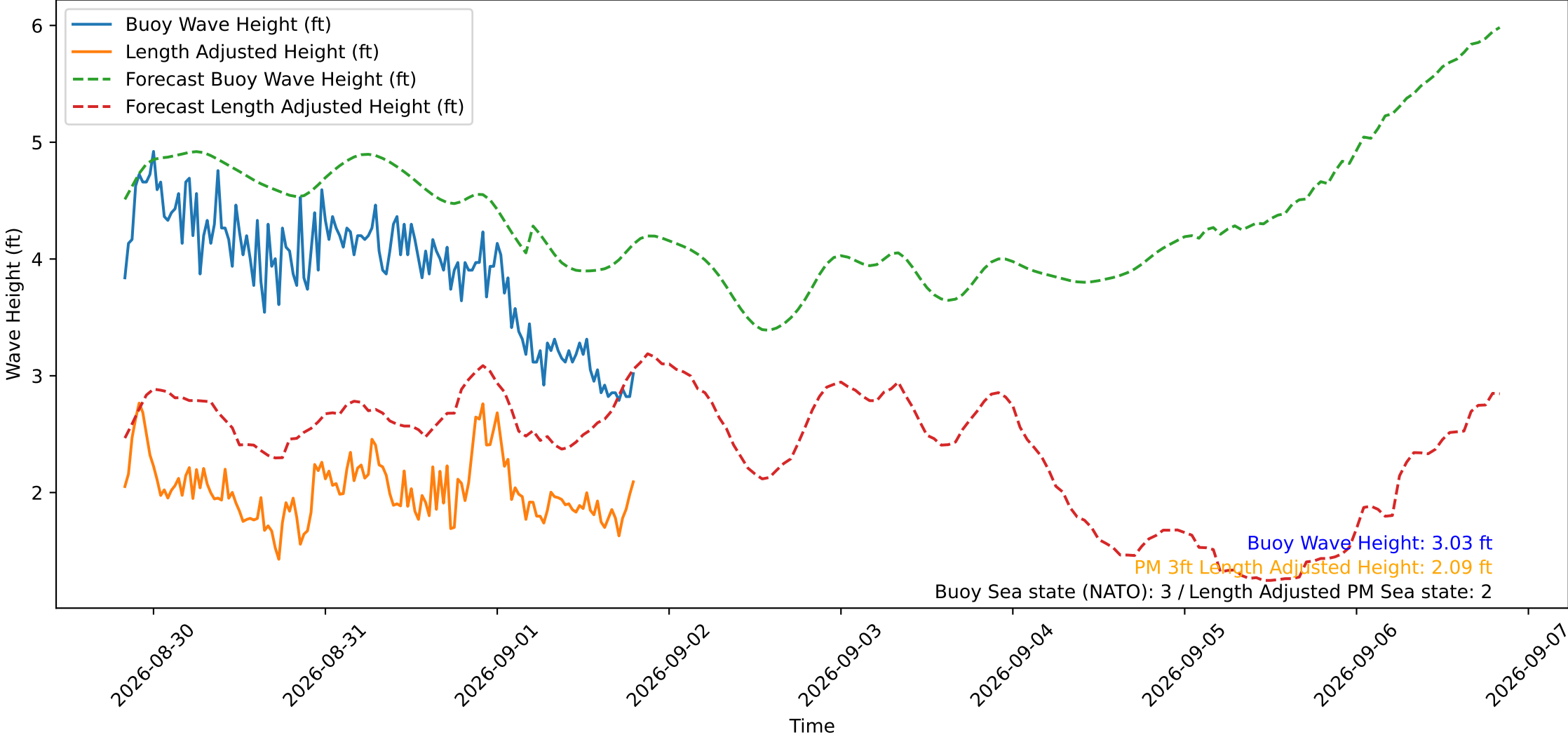
Wave Heights over Time for Green Beach at 2026-09-01 19:41:13
