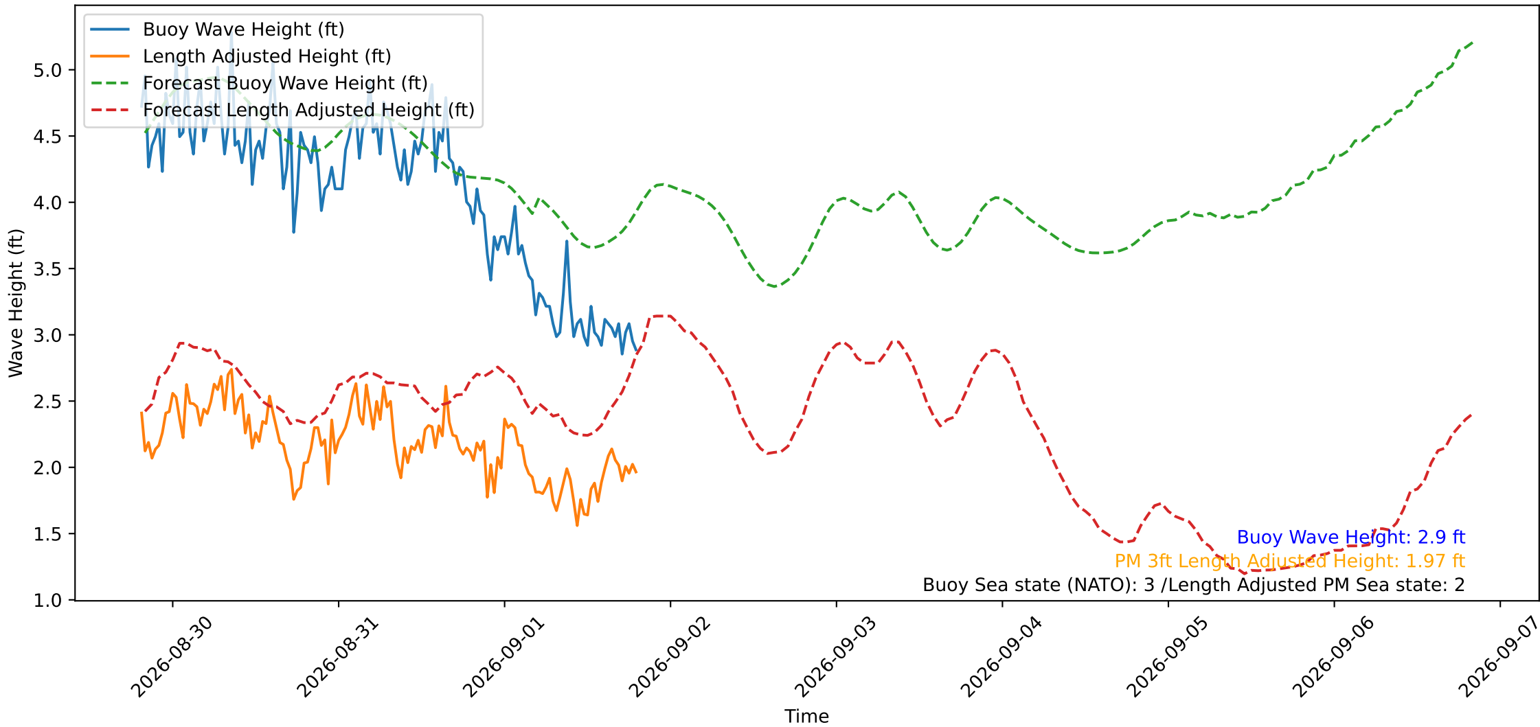
Wave Heights over Time for Oceanside Harbor at 2026-09-01 19:40:30
