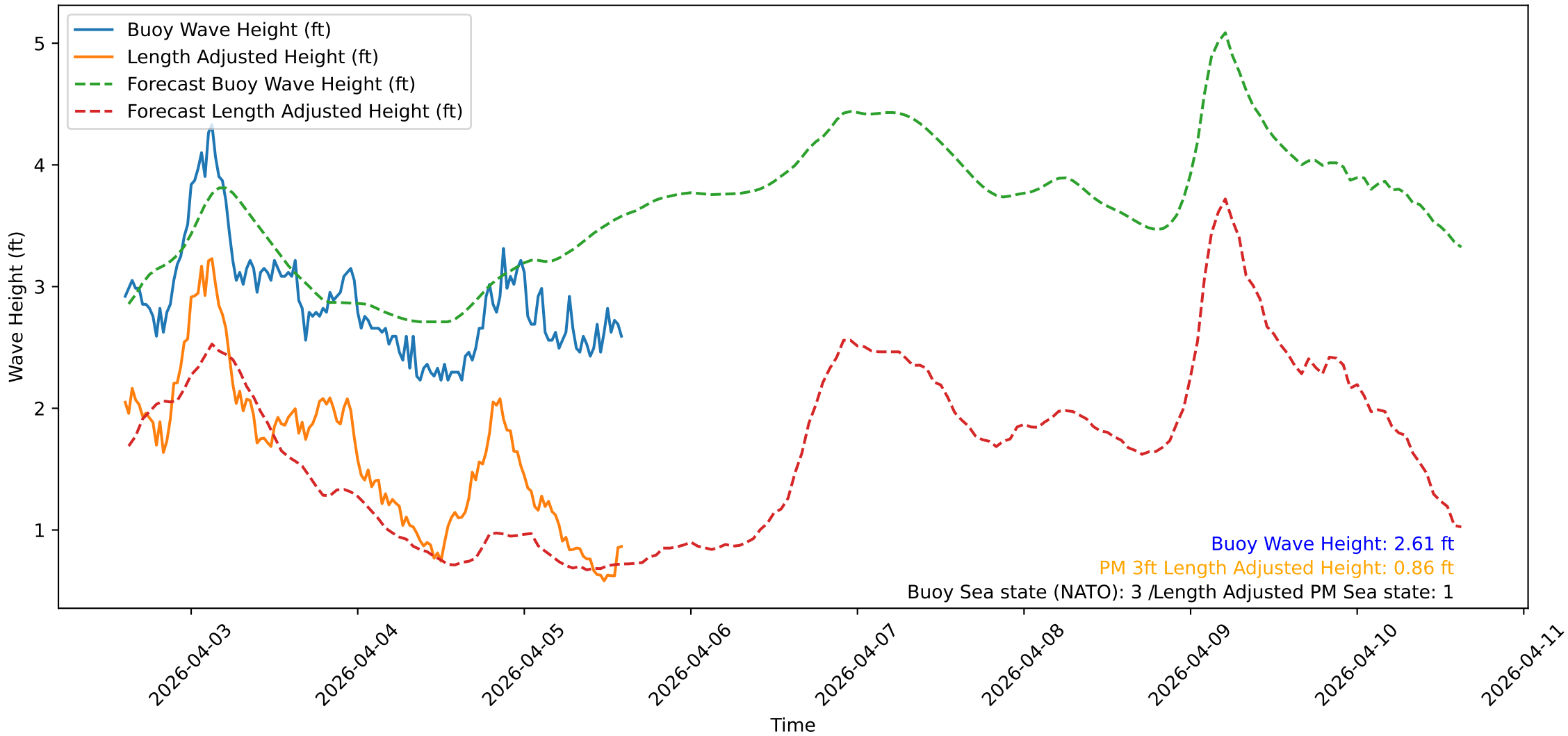
Wave Heights over Time for Green Beach at 2026-04-05 14:41:11
