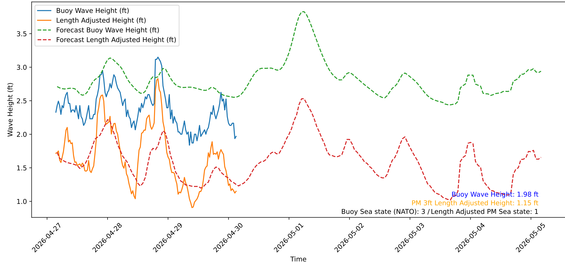
Wave Heights over Time for Green Beach at 2026-04-30 03:41:12
