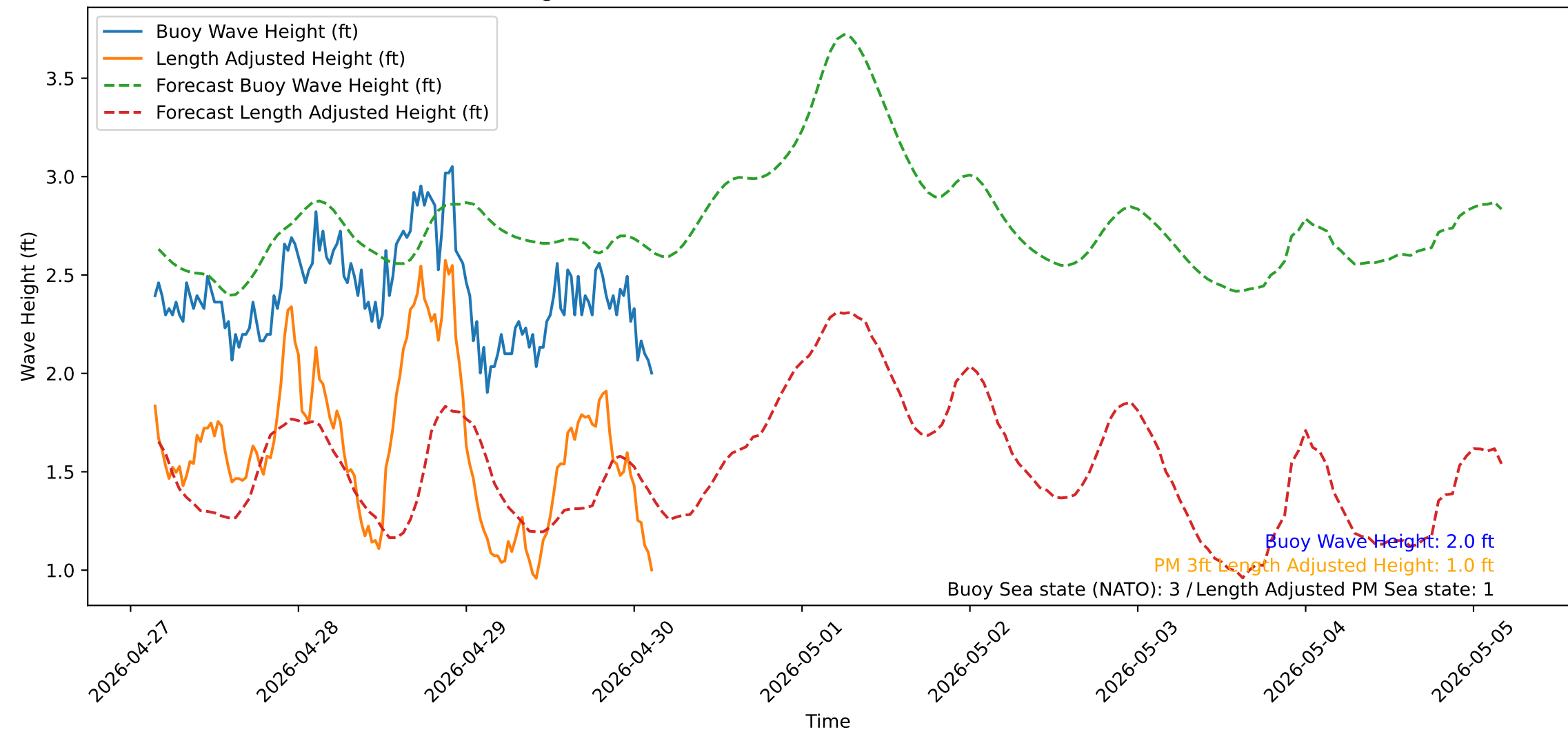
Wave Heights over Time for Oceanside Harbor at 2026-04-30 03:40:31
