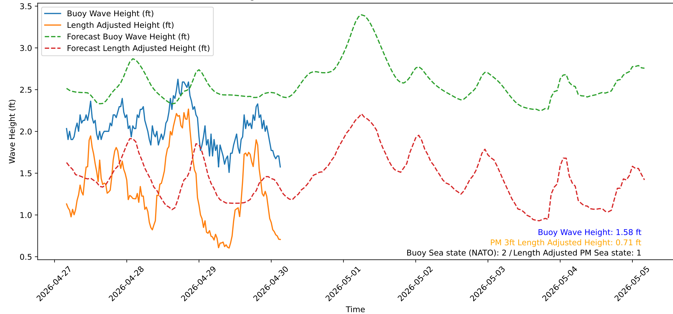
Wave Heights over Time for Red Beach at 2026-04-30 03:40:50
