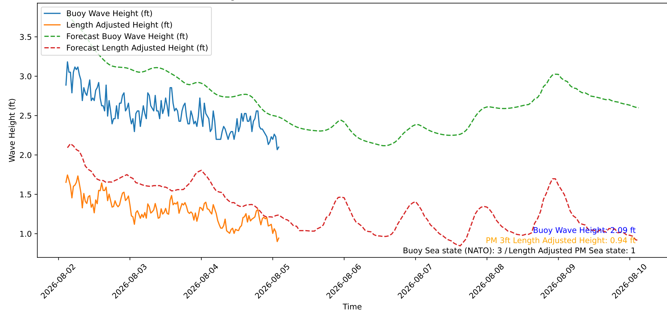
Wave Heights over Time for Oceanside Harbor at 2026-08-05 02:30:27
