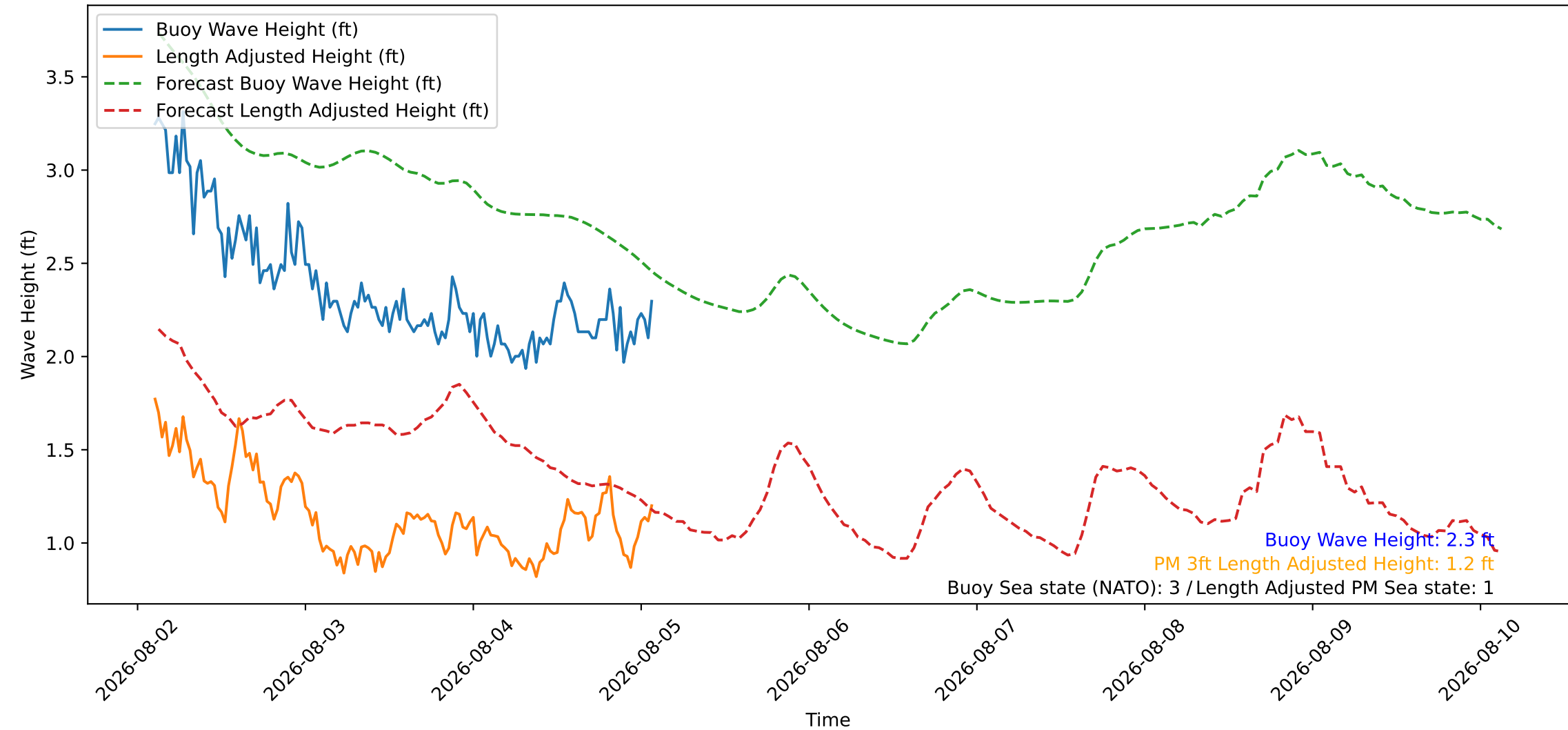
Wave Heights over Time for Green Beach at 2026-08-05 02:31:09
