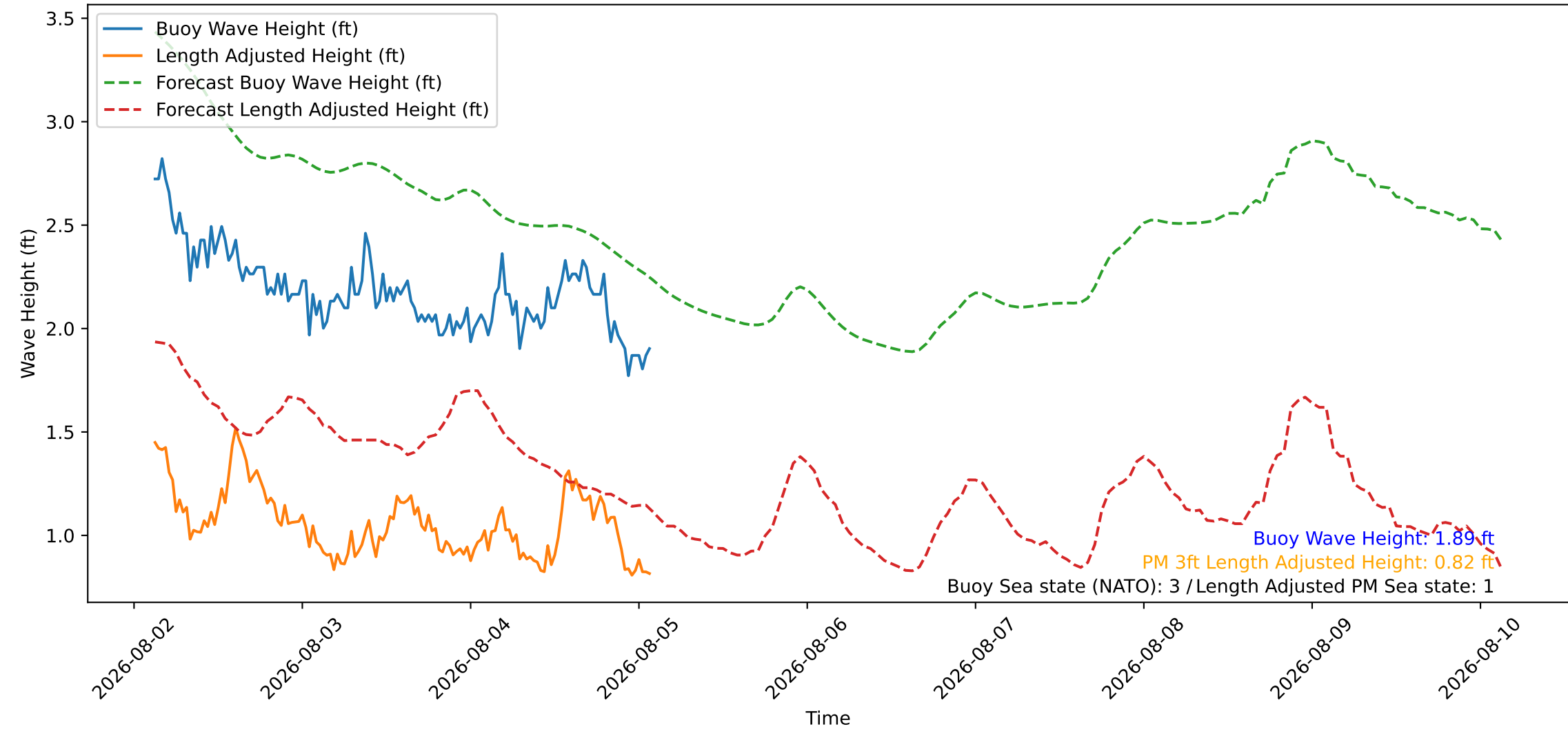
Wave Heights over Time for Red Beach at 2026-08-05 02:30:47
