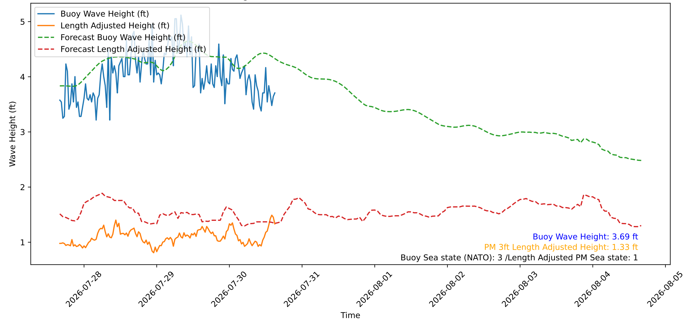
Wave Heights over Time for Red Beach at 2026-07-30 15:50:48
