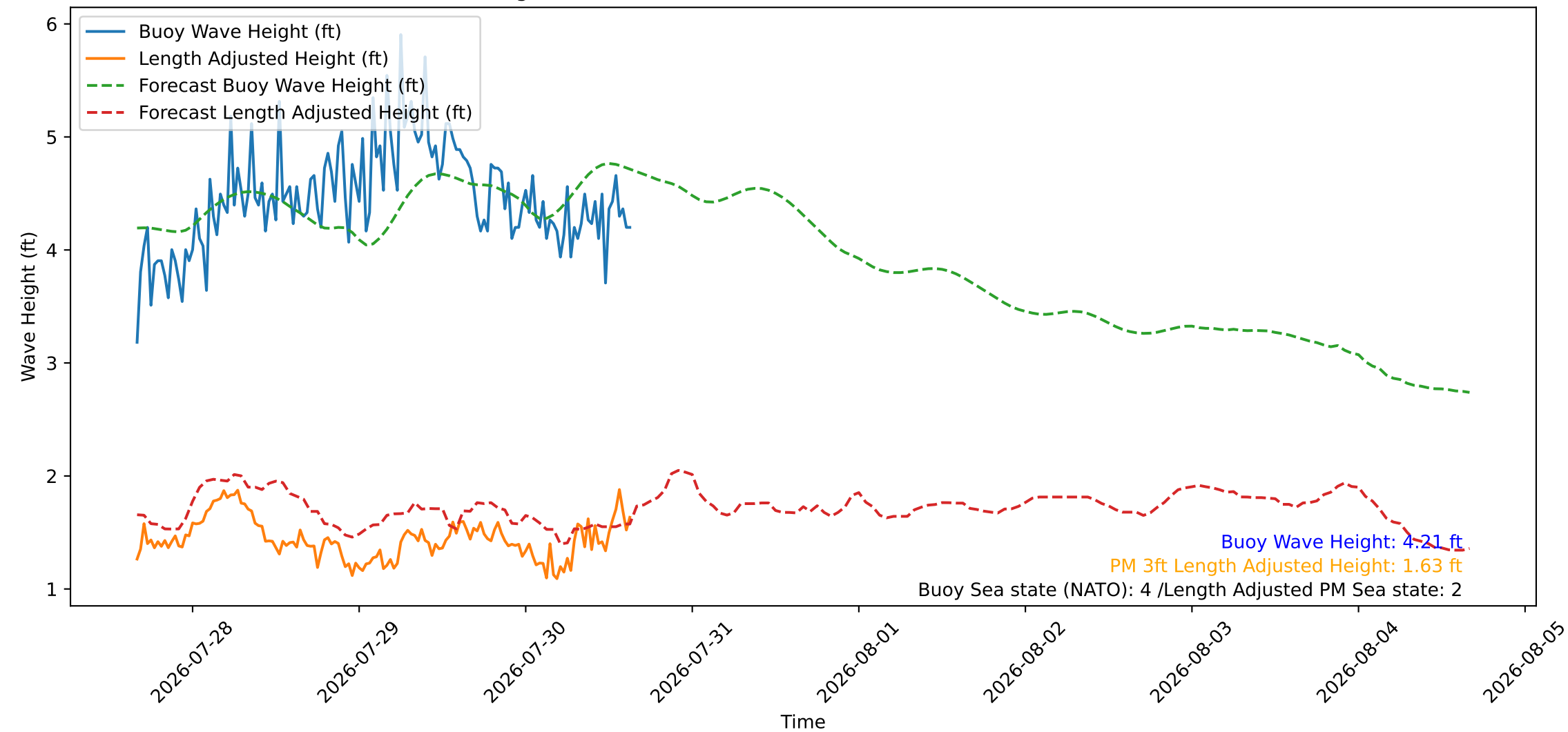
Wave Heights over Time for Oceanside Harbor at 2026-07-30 15:50:26
