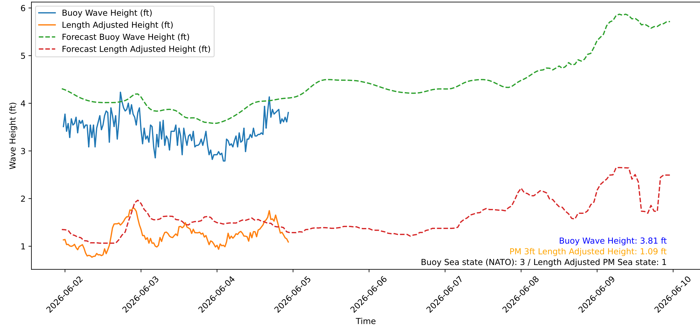
Wave Heights over Time for Green Beach at 2026-06-04 23:21:09
