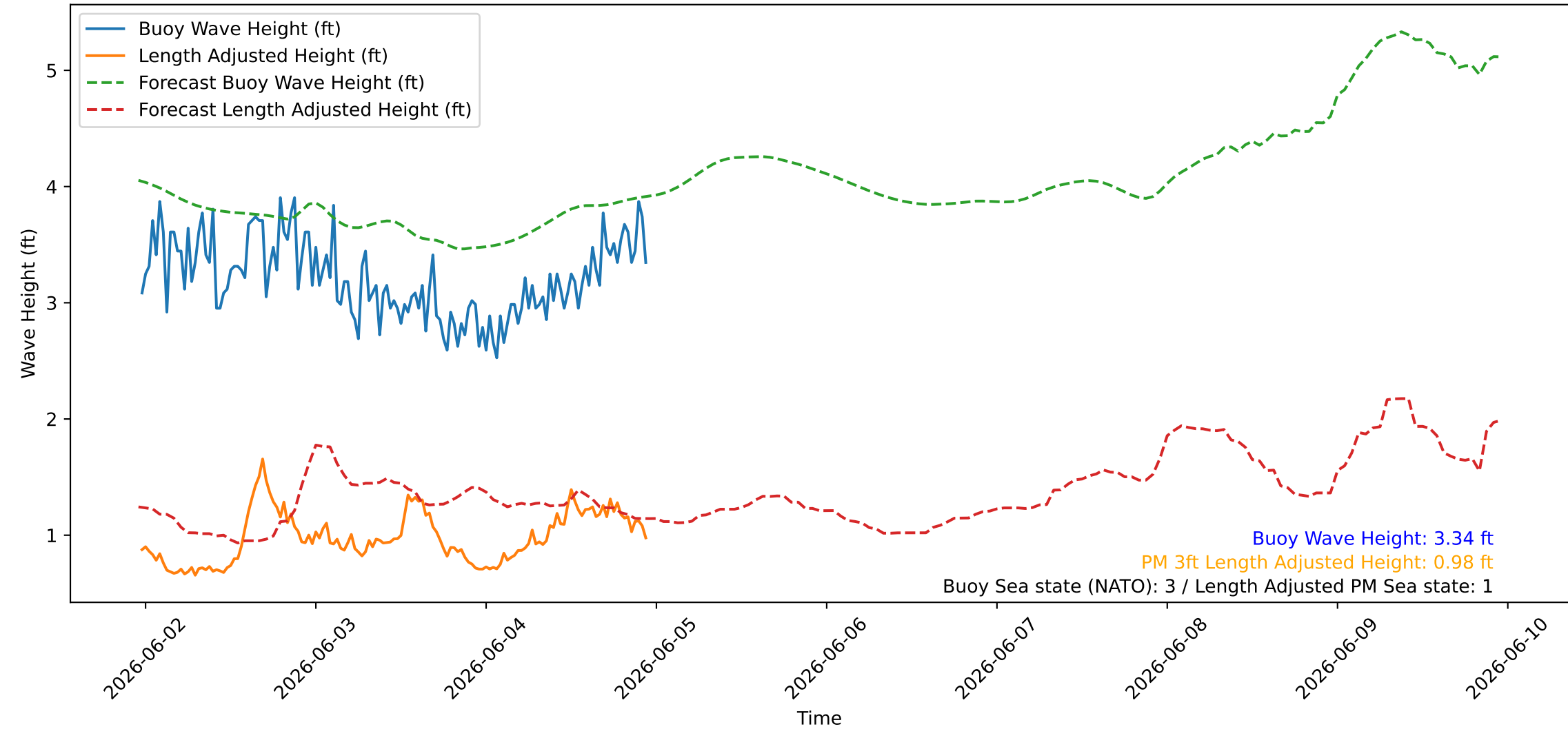
Wave Heights over Time for Red Beach at 2026-06-04 23:20:47
