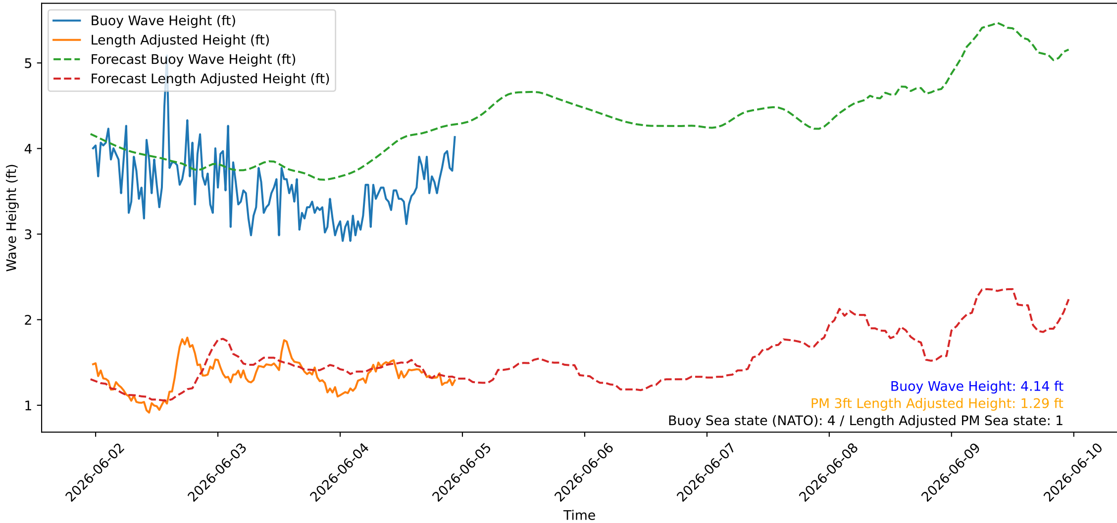
Wave Heights over Time for Oceanside Harbor at 2026-06-04 23:20:26
