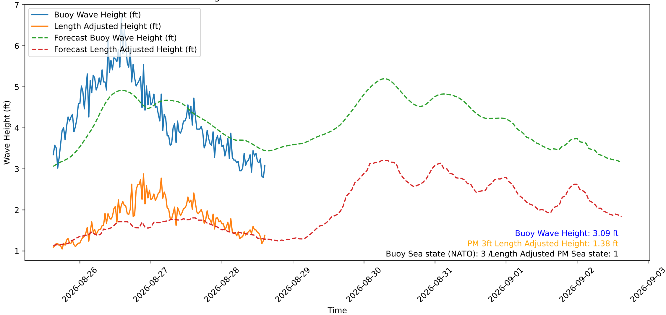
Wave Heights over Time for Oceanside Harbor at 2026-08-28 15:10:29
