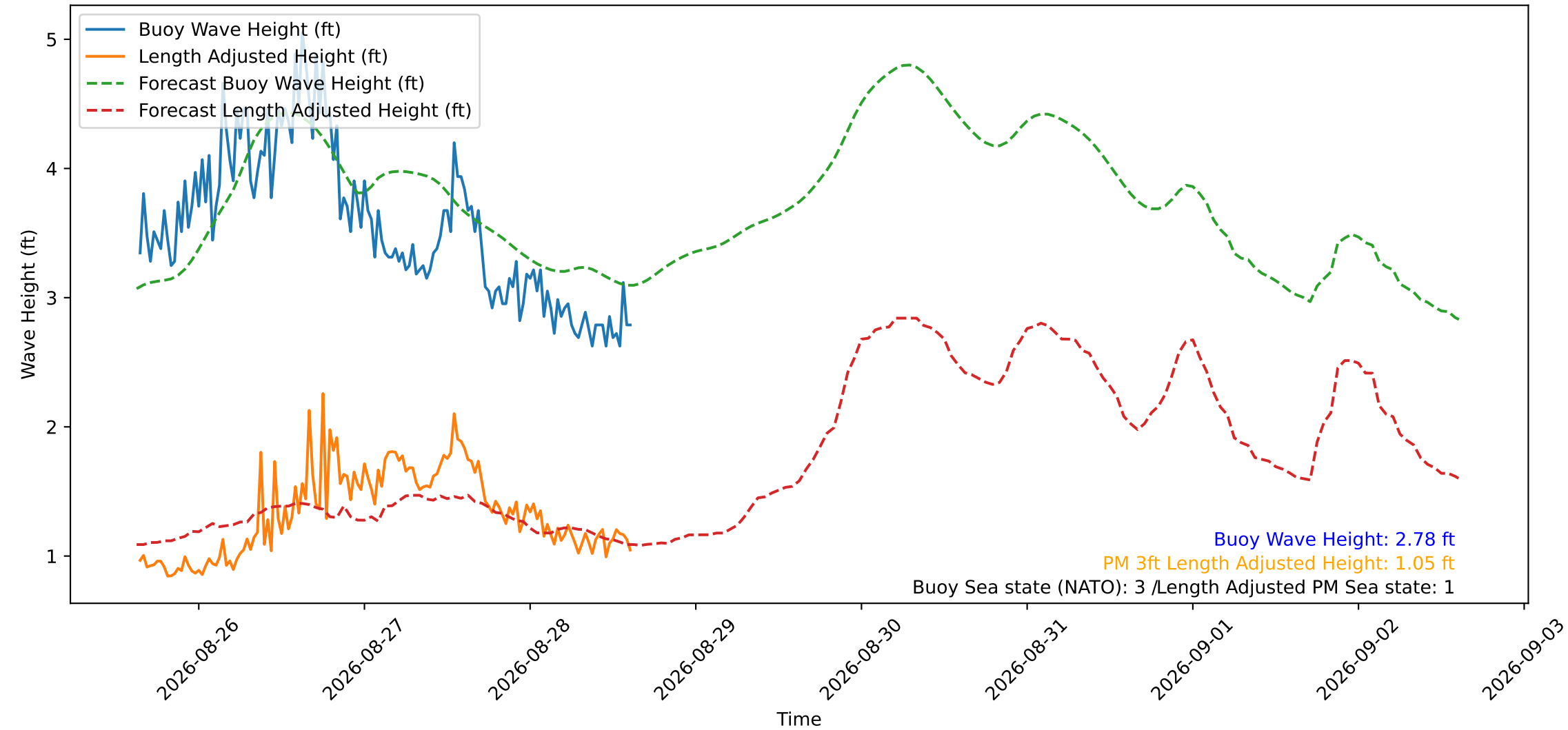
Wave Heights over Time for Red Beach at 2026-08-28 15:10:49
